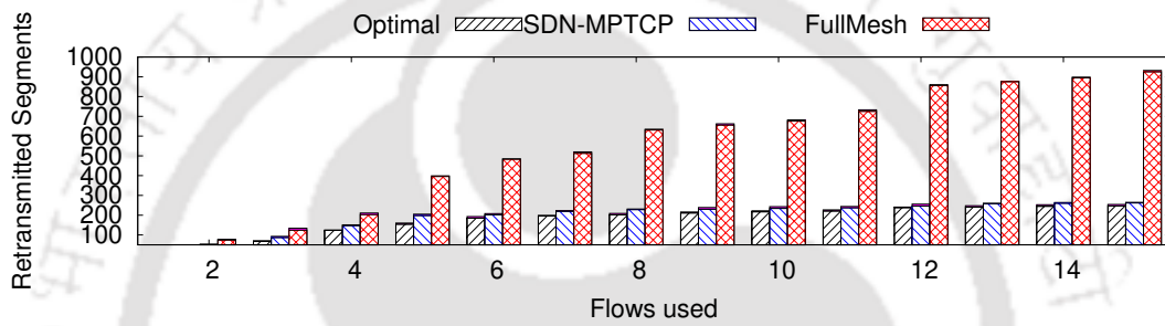
Fig. 3.13: Retransmitted Segments
