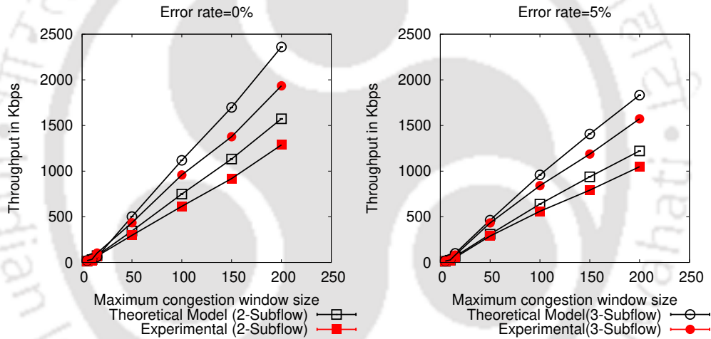
Fig. 3.8: Throughput Comparison
