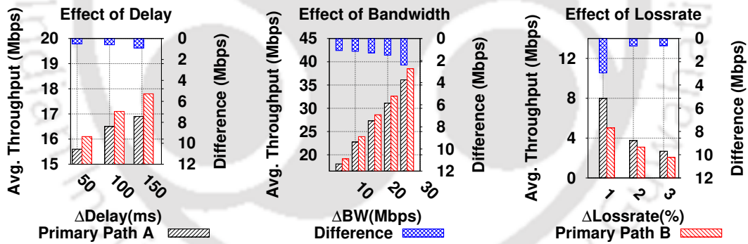
Fig. 3.5: Throughput variation
