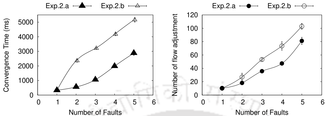
Fig. 4.6: Effect of Link Failure:Convergence Time Fig. 4.7: Effect of Link Failure:Flow Readjustments
