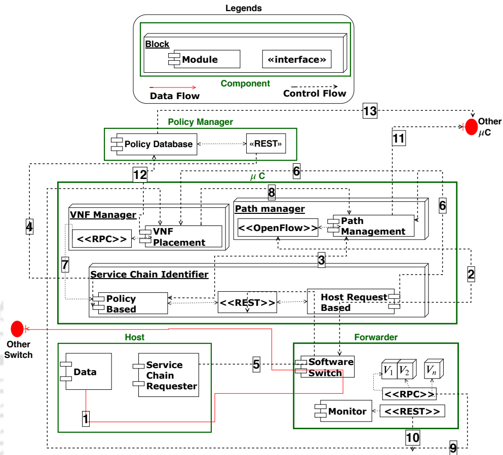
Fig. 6.2: Component diagram of Amalgam
