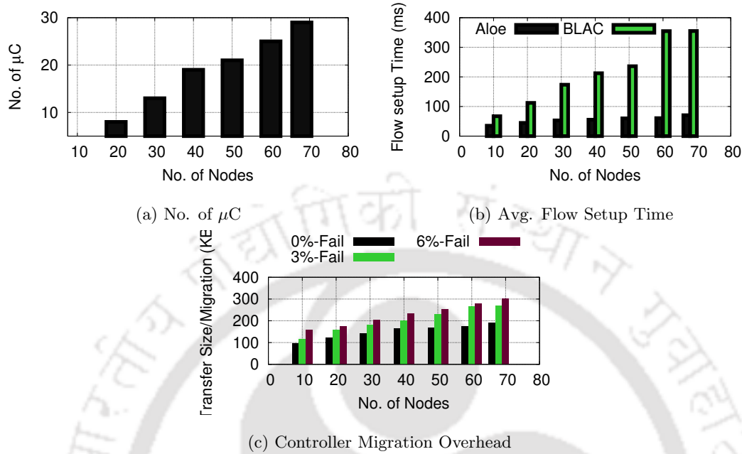
Fig. 5.10: Effect of Scaling Aloe \mu\text{C} Deployments
