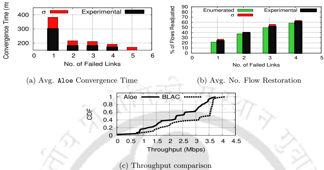
Fig. 5.8: Testbed: Effect of failure on Aloë performance ( \sigma = standard deviation)
