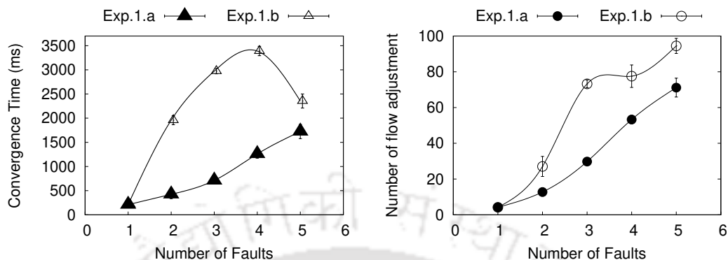
Fig. 4.4: Effect of Flipper Failure: Convergence Time Fig. 4.5: Effect of Flipper Failure: Flow Readjustments
