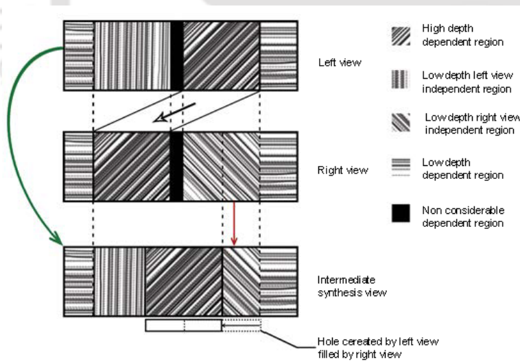
Figure 5.6: Watermarking zone shift.
