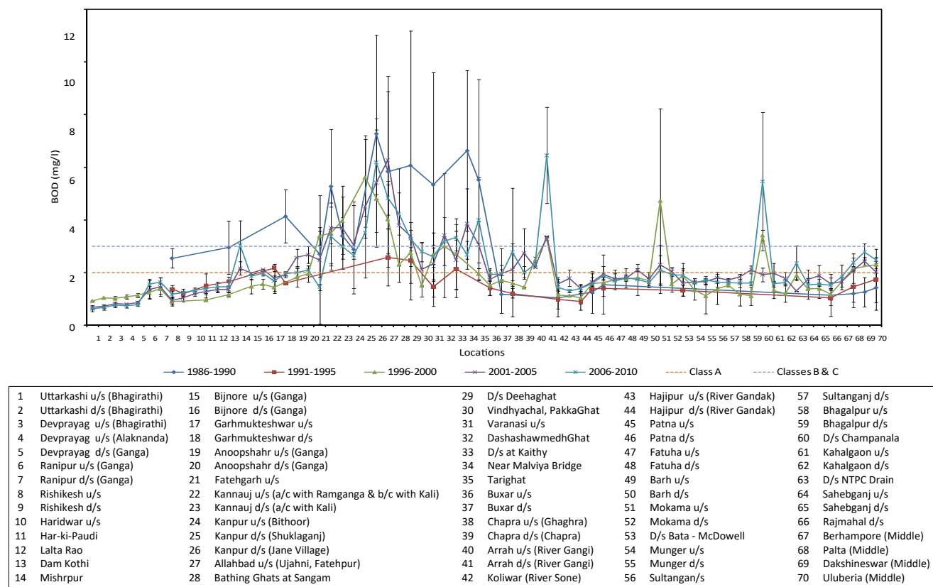
Figure 6.2: Variation in 5-year Average BOD at Various Locations along the Ganga River
