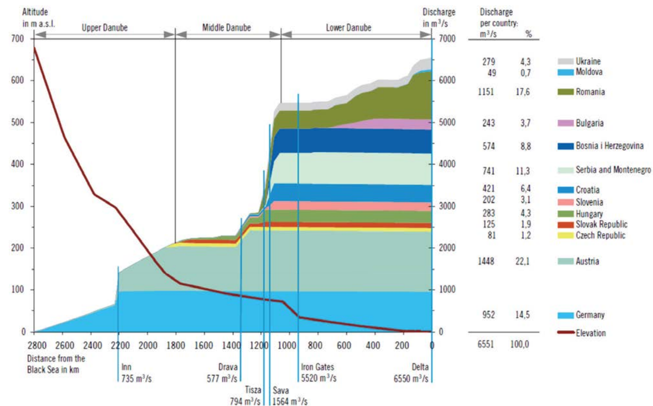
Figure 4.1: Longitudinal Profile of River Danube and Contribution to Danube River Flow from each Country of the Danube Basin during 1994–1997 [ICPDR, 2005]
