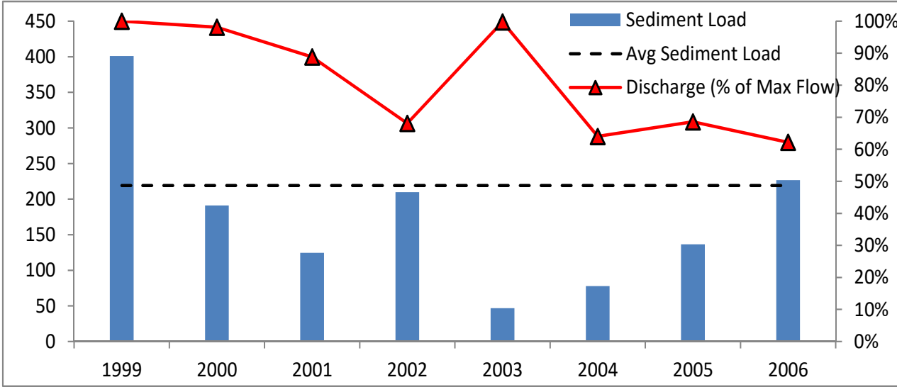
Figure A2.13: Annual Sediment Loads (in million metric tons) at Farakka (including Feeder Canal)
