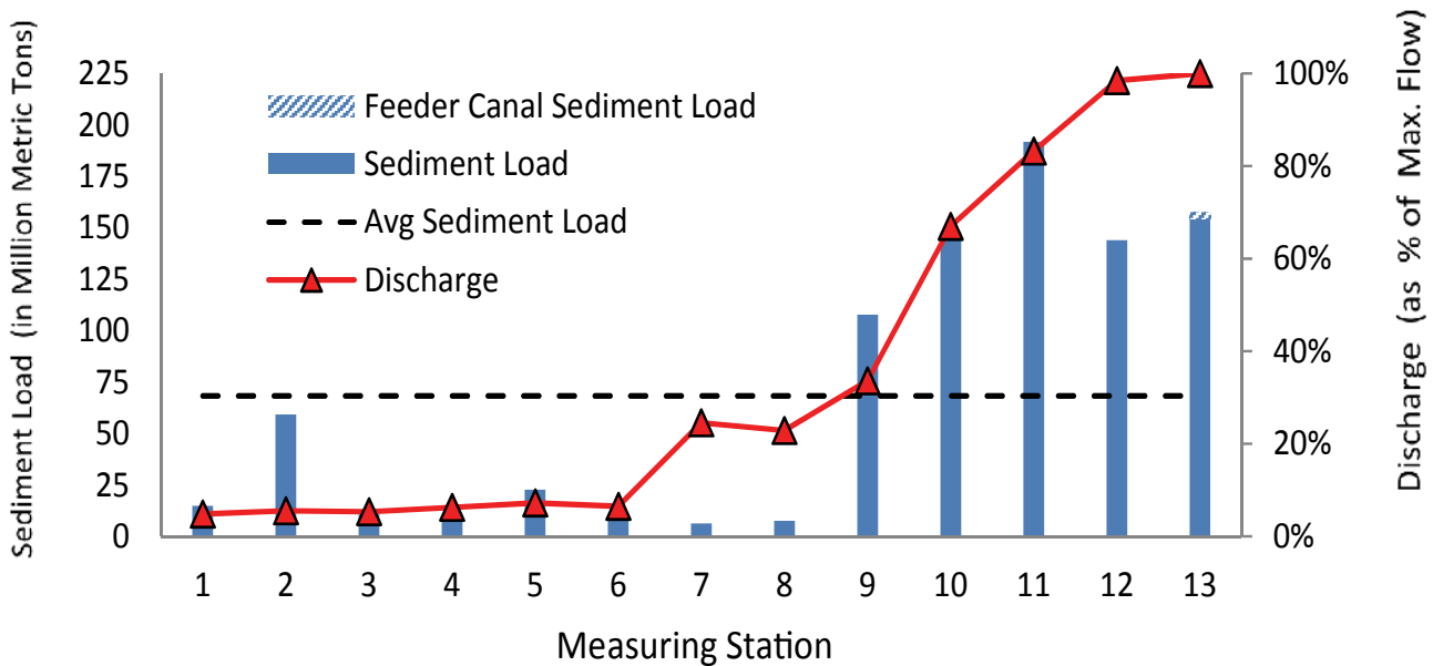
Figure 7.3: Comparison of the Average Wet Season Sediment Loads (for period 1999-2006) at Different Locations of National River Ganga
