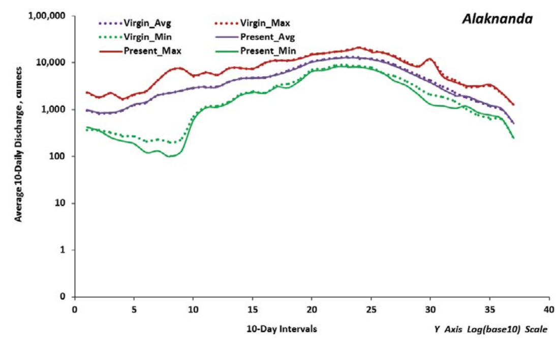
Figure A1.1: 10-Daily Hydrographs for River Alaknanda
