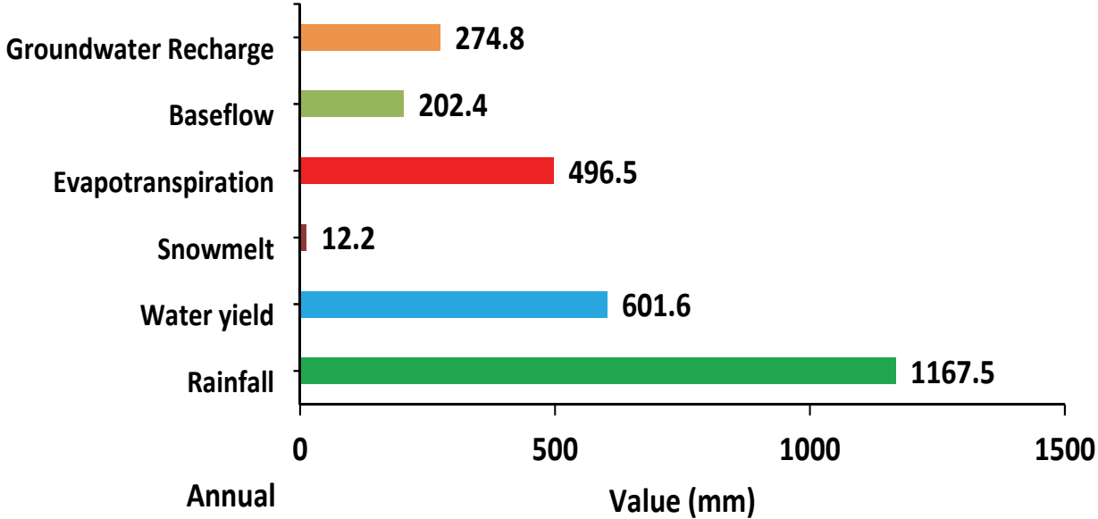
Figure 6.2a: Average (1969-2006) Annual Water Balance of the Modeled Ganga Basin
