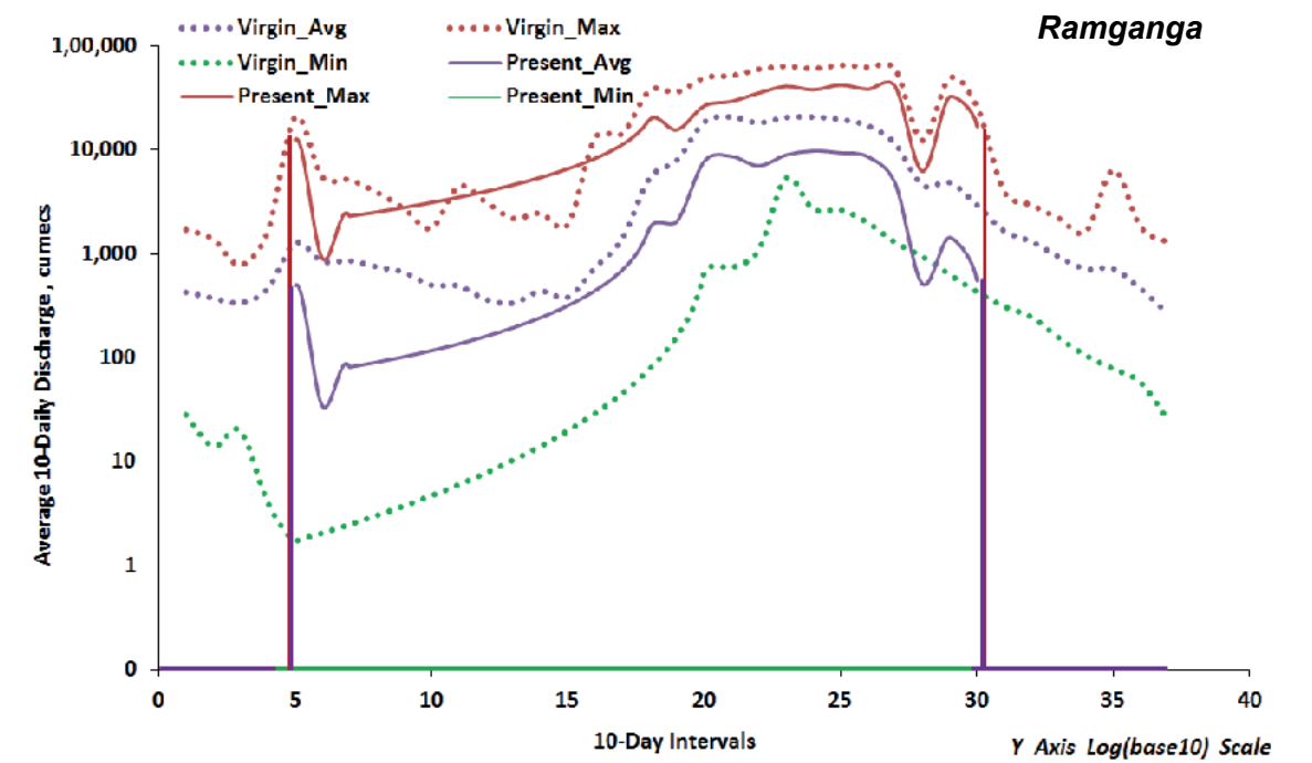
Figure A1.15: 10-Daily Hydrographs for River Ramganga
