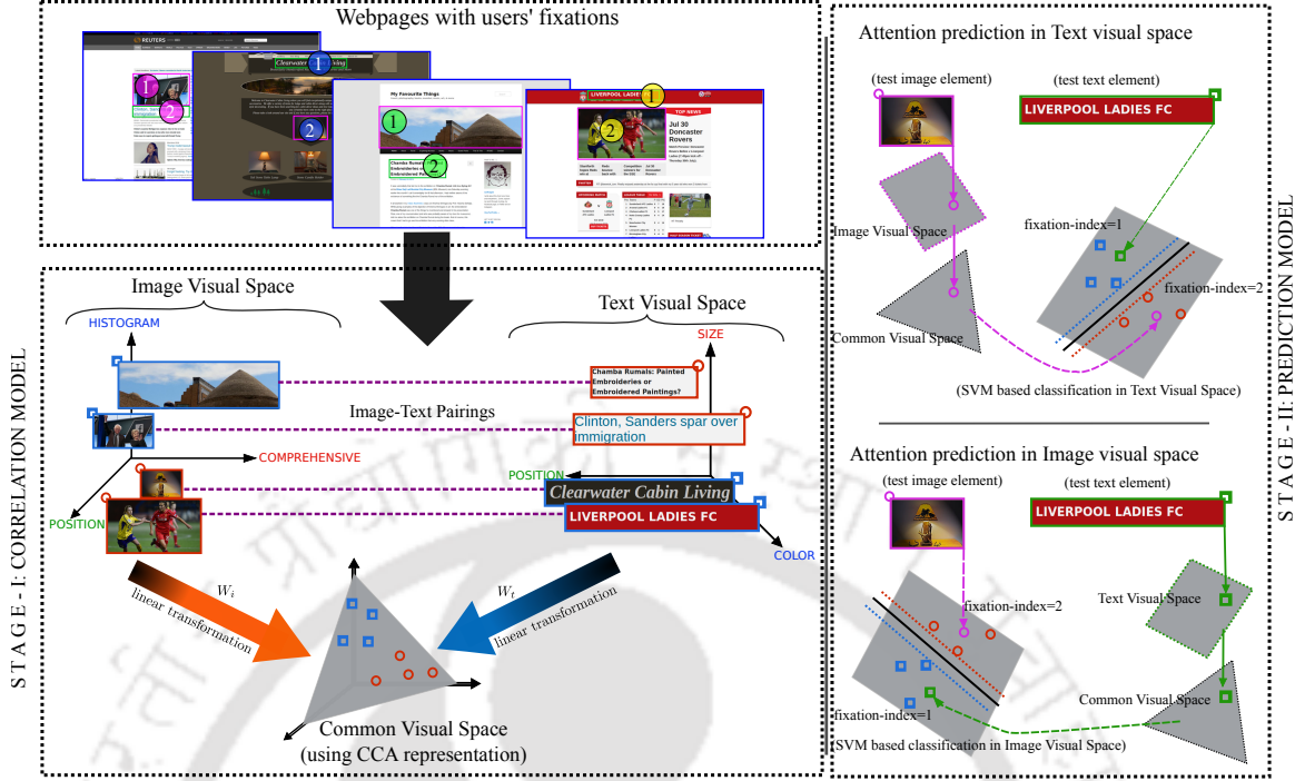
Figure 6.6: WUG: Schematic of the proposed web element attention prediction approach. Left) Stage-I: Pair the text and image elements based on shared webpage and fixation-indices, subsequently, learn a maximally correlated Common Visual Space for both the natural visual spaces. Right) Stage-II: Project all cross-modal elements into either of natural visual space through the achieved Common Visual Space and employ SVM based classification for attention prediction.
