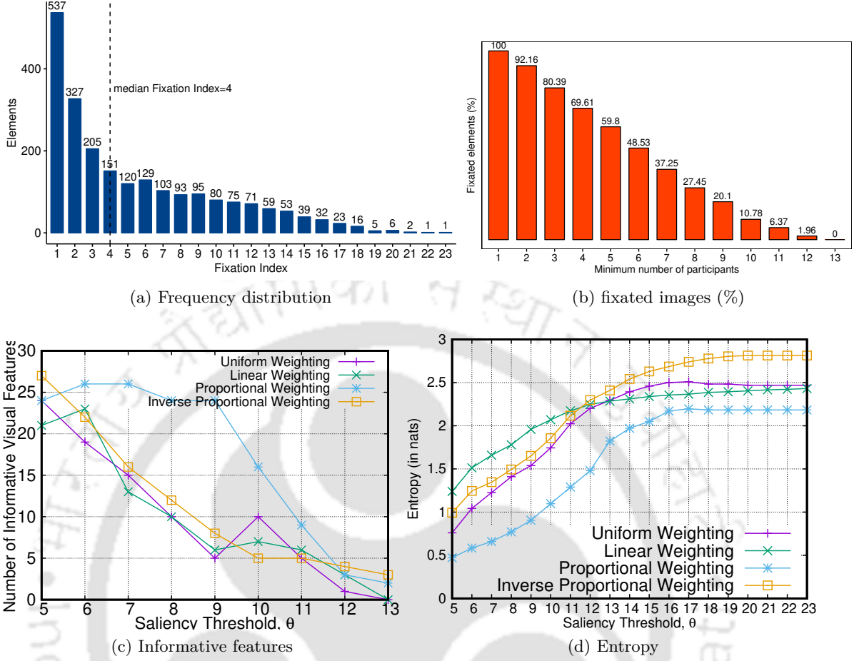
Figure 4.13: \theta based variation in (c) number of information visual features, and (d) entropy, for four weighting strategies
