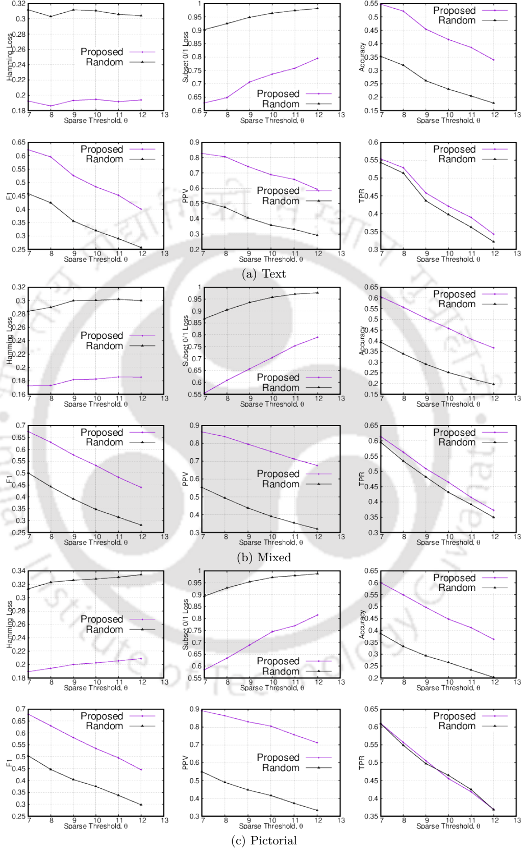
Figure 4.22: Multilabel prediction performance comparison with baseline for three categories: (from left to right) Hamming loss, Subset 0/1 loss, Accuracy, F1-score, PPV, and TPR.
