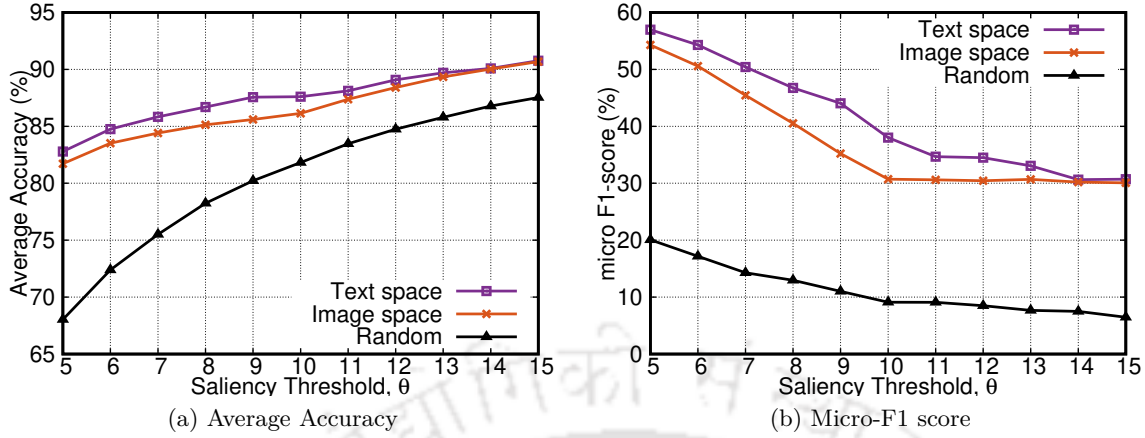
Figure 6.2: Experiment-I: Prediction performance metrics with variation in \theta
