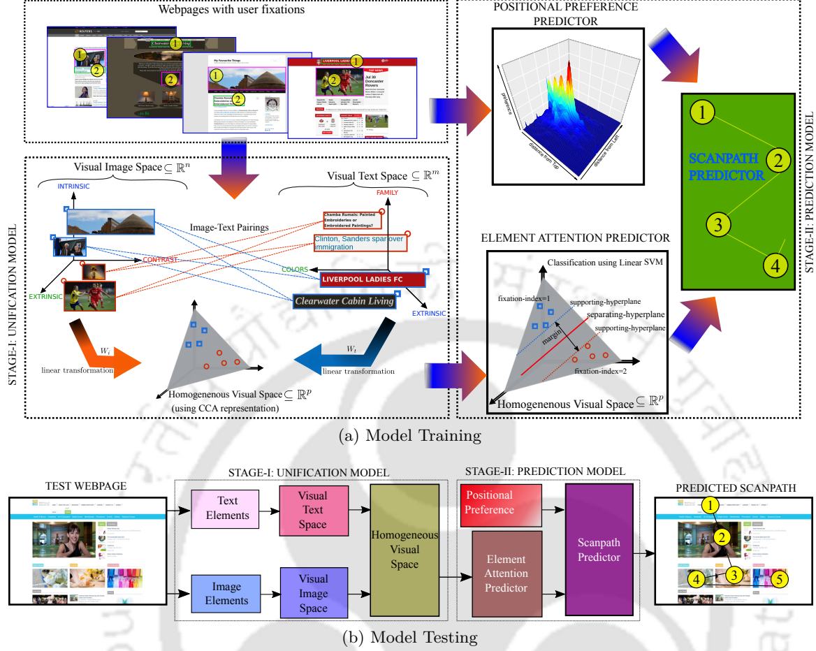
Figure 7.1: WG: Schematic of the proposed approach. UNIFICATION MODEL achieves homogeneous representation for text and images. ELEMENT ATTENTION PREDICTOR utilizes the homogeneous representation to build classifiers for attention prediction on web elements. SCANPATH PREDICTOR arranges the elements into scanpath where the positional-bias captured in POSITIONAL PREFERENCE PREDICTOR helps in resolving the conflicts among elements.
