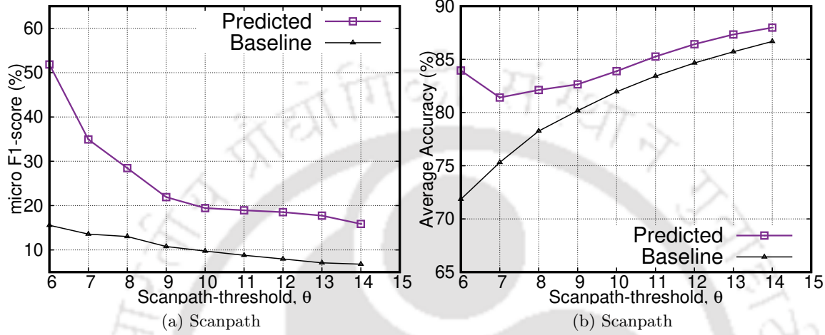
Figure 7.8: Experiment-I prediction performance with variation in scanpath-threshold \theta
