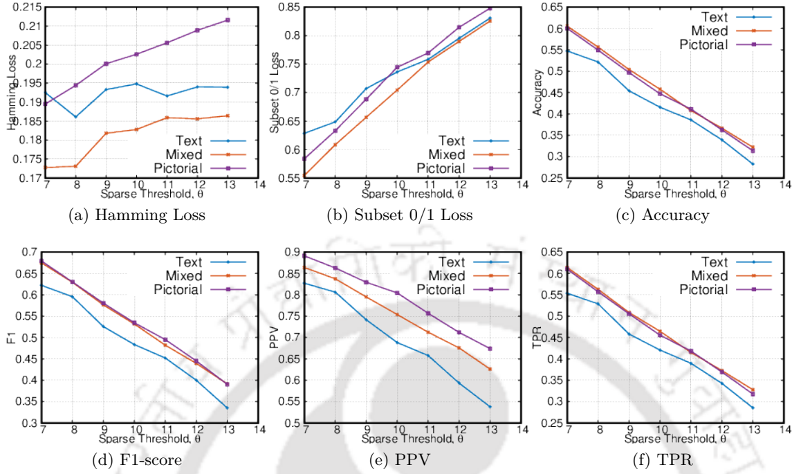
Figure 4.21: MUMLA prediction performance with variation in saliency-threshold \theta
