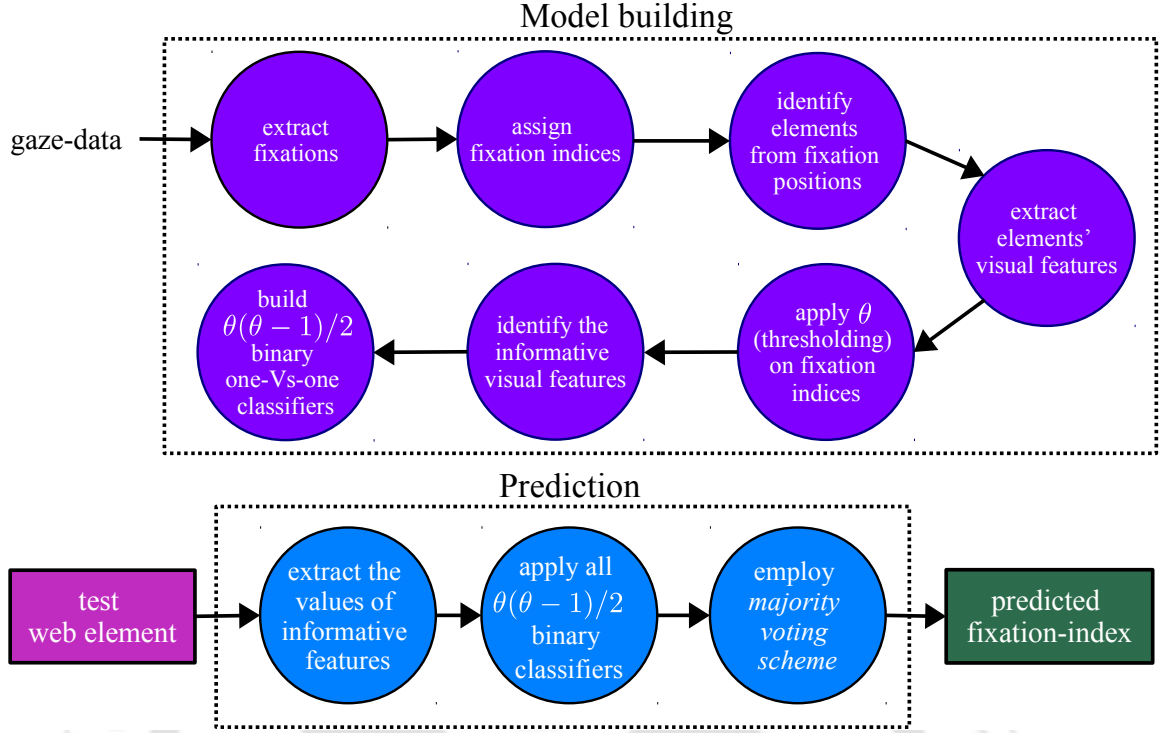
Figure 4.6: Ordinal visual attention prediction procedure
