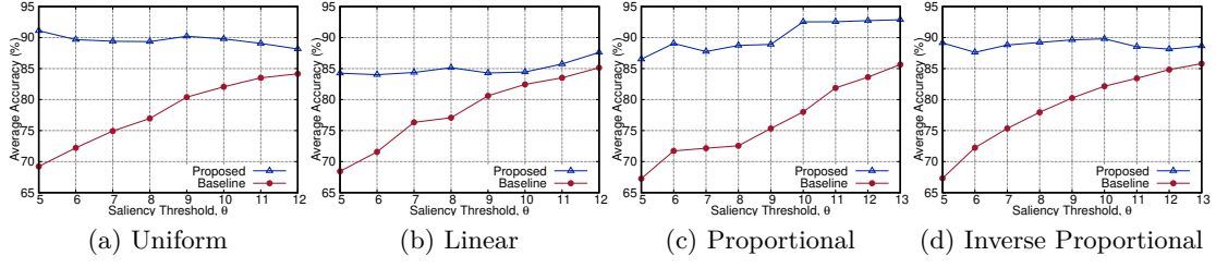
Figure 4.15: Average accuracies of four weighting strategies compared with the baseline for varying \theta
