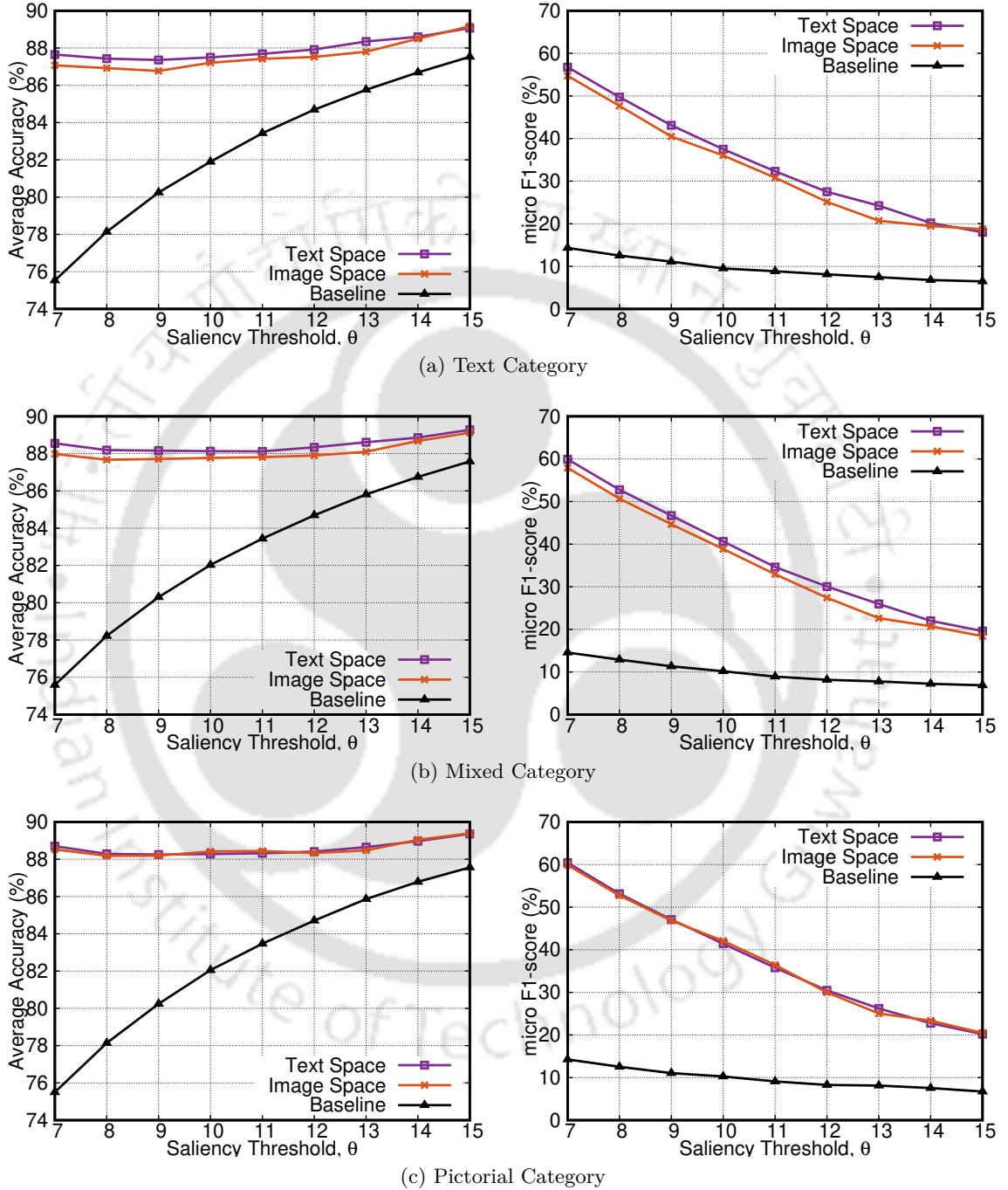
Figure 6.8: Experiment-III: Prediction performance metrics with variation in \theta
