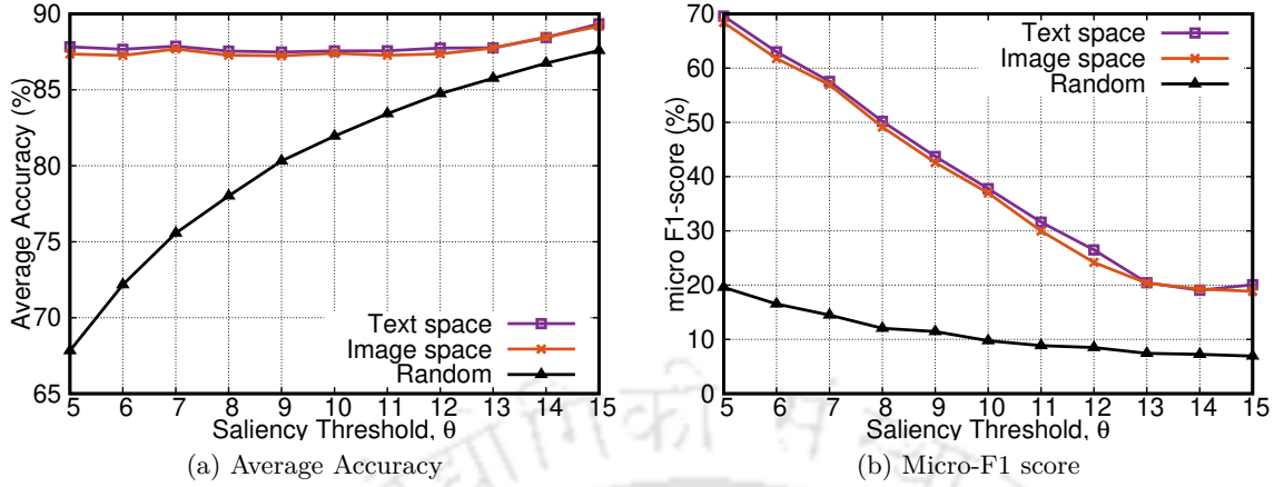
Figure 6.7: Experiment-I: Prediction performance metrics with variation in \theta
