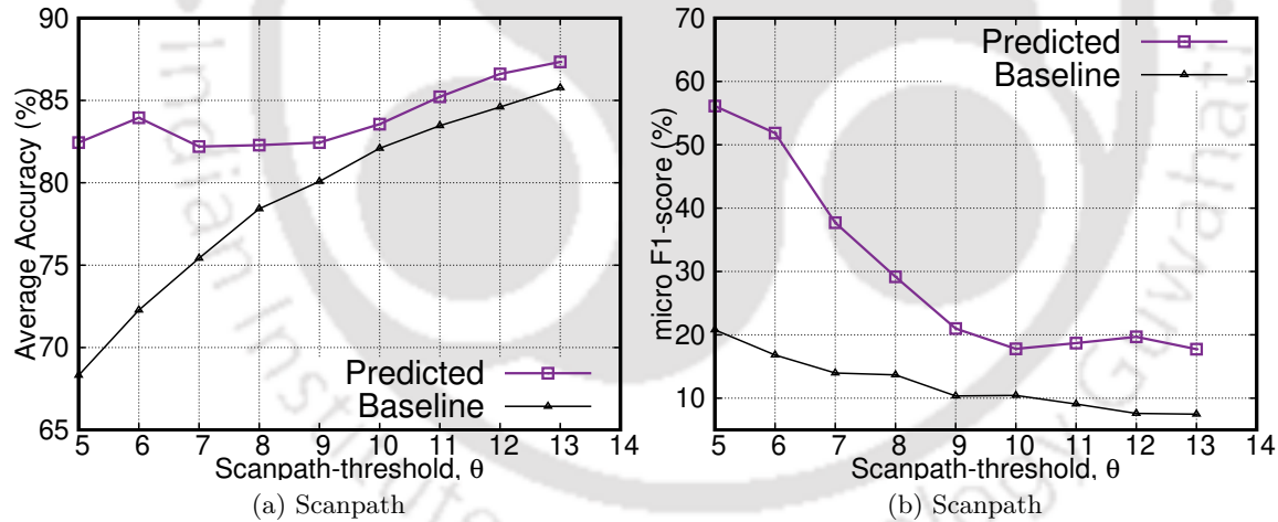
Figure 7.5: Experiment-II prediction performance with variation in thresholded value
