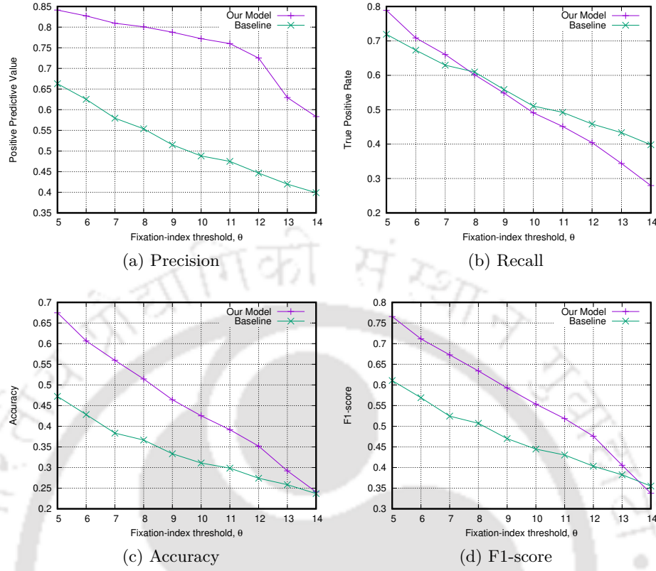
Figure 4.24: Performance metrics with variation in fixation-index threshold
