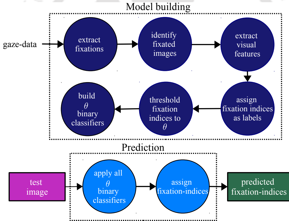
Figure 4.19: Proposed model flow-diagram
