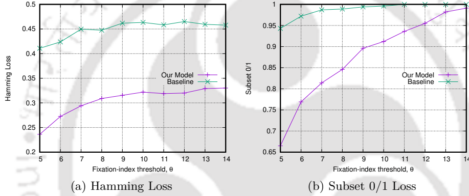
Figure 4.23: Loss metrics with variation in fixation-index threshold
