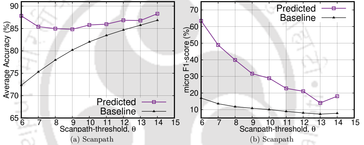
Figure 7.4: Experiment-I prediction performance with variation in thresholded value
