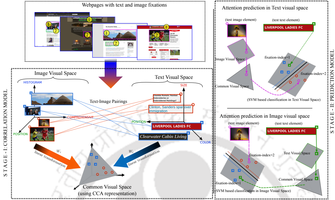
Figure 6.1: WG: Schematic of the proposed web element attention prediction approach. Left) Stage-I: Pair the text and image elements based on shared webpage and fixation-indices, subsequently, learn a maximally correlated Common Visual Space for both the natural visual spaces. Right) Stage-II: Project all cross-modal elements into either of natural visual space through the achieved Common Visual Space and employ SVM based classification for attention prediction.
