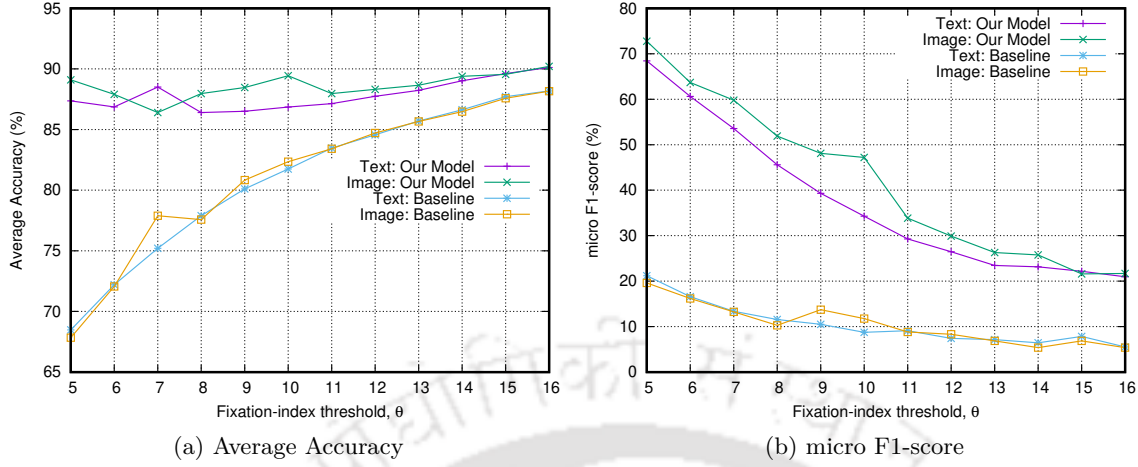
Figure 4.7: Prediction performance of informative intrinsic visual features with variation in \theta
