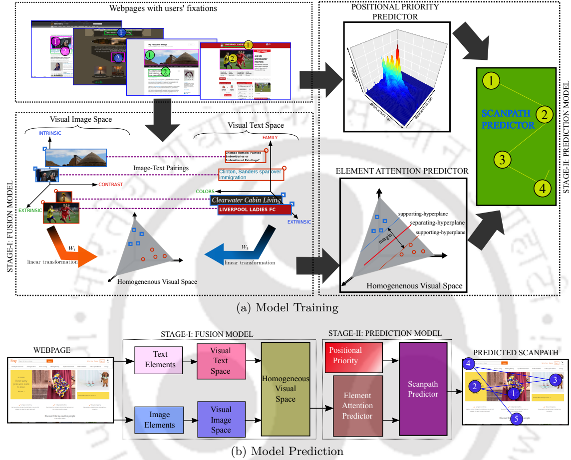
Figure 7.7: WUG: Schematic of the proposed approach. FUSION MODEL employs canonical correlation analysis (CCA) to achieve the homogeneous representation for text and images. ELEMENT ATTENTION PREDICTOR applies multiclass classification on the achieved homogeneous representation to predict the user attention on web elements. SCANPATH PREDICTOR ordiates the scanpath sequence through zero-sum rule where the positional-preference capturing POSITIONAL PRIORITY PREDICTOR is utilized towards resolving the conflicts among elements.
