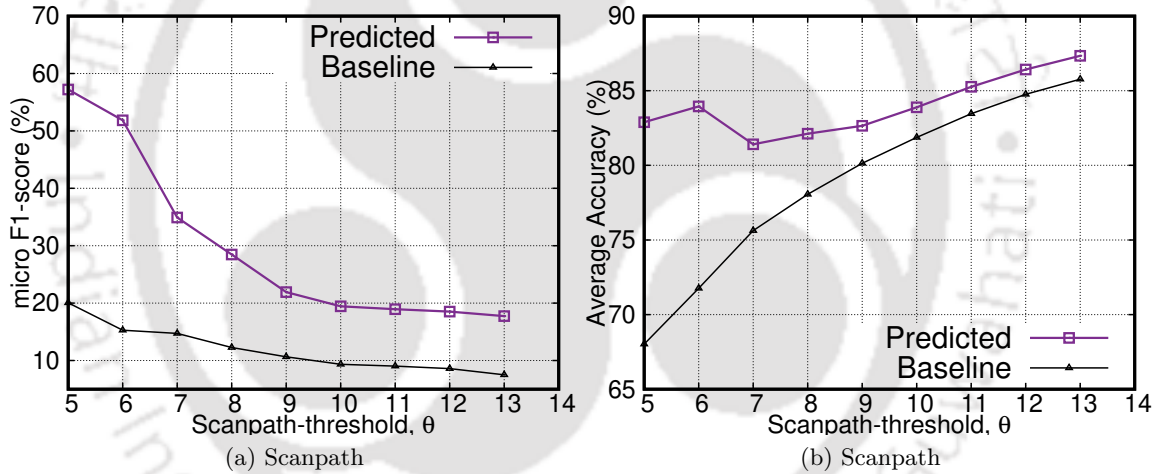
Figure 7.9: Experiment-II prediction performance with variation in scanpath-threshold \theta
