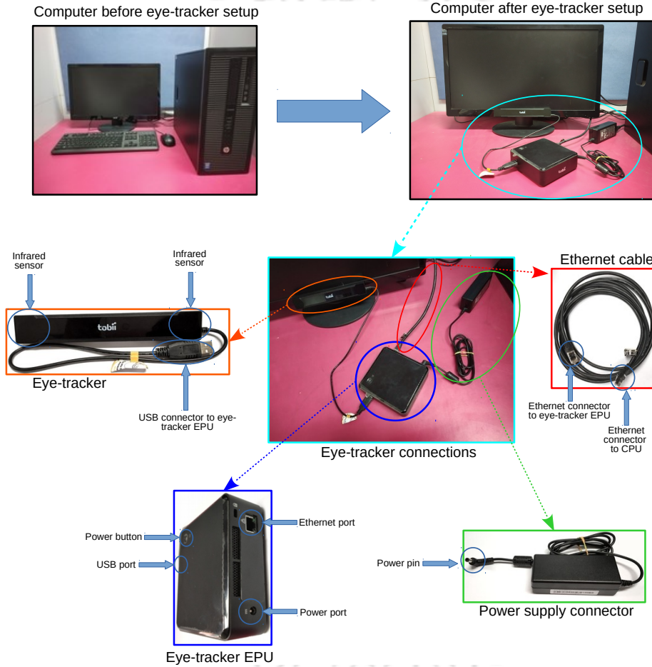
Figure 3.1: Eye-tracker setup used for collecting the gaze-data
