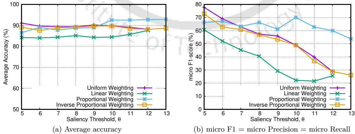
Figure 4.14: Average Accuracy and micro F1-scores with variation in \theta
