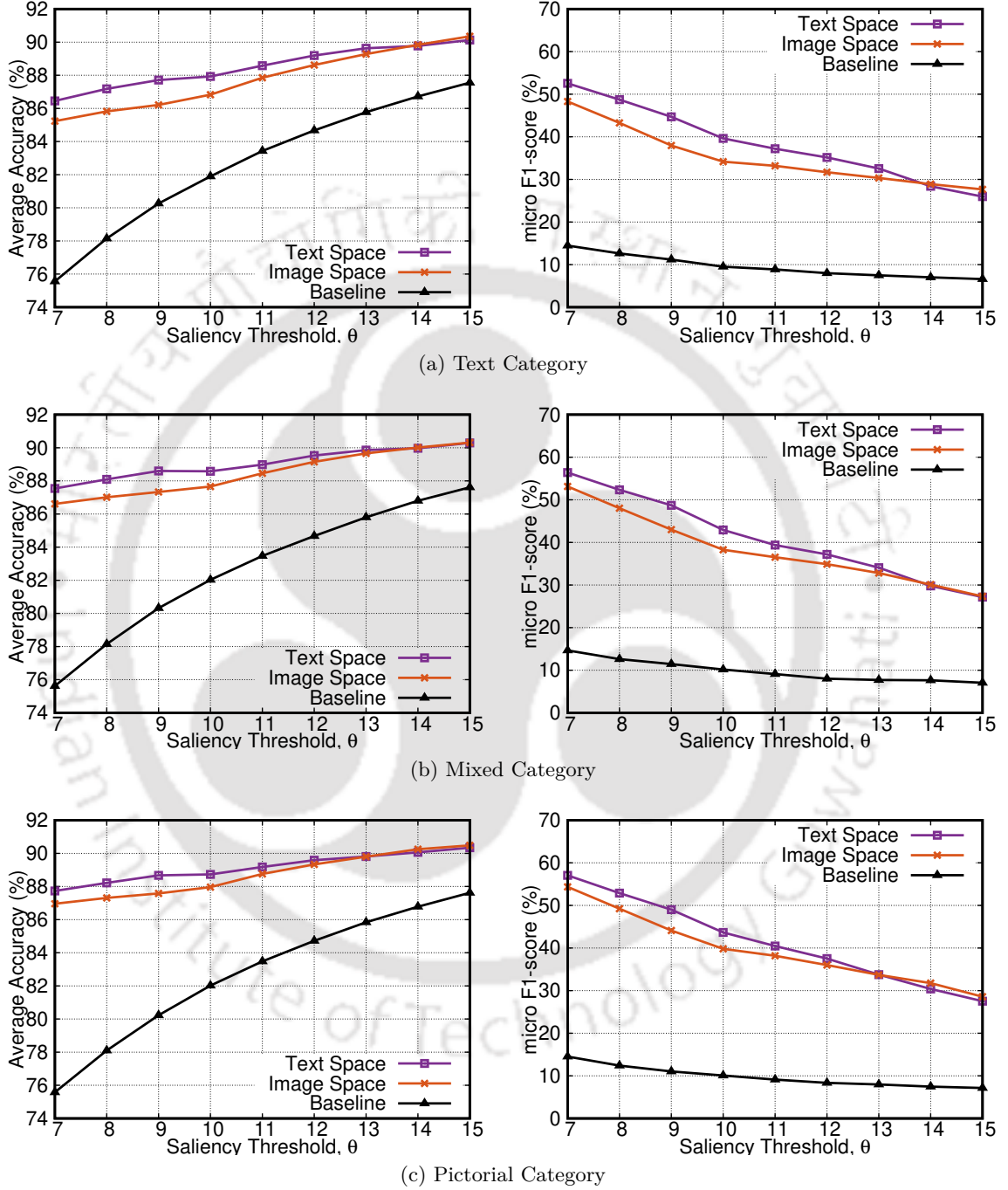
Figure 6.4: Experiment-III: Prediction performance metrics with variation in \theta
