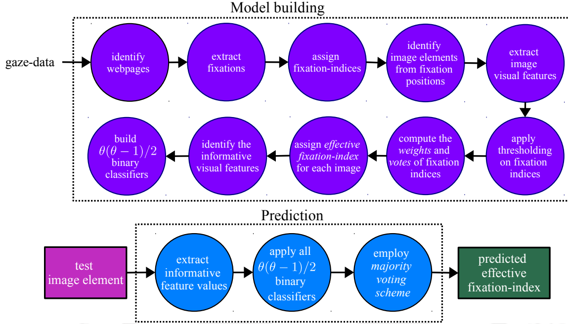
Figure 4.12: Proposed model flow-diagram
