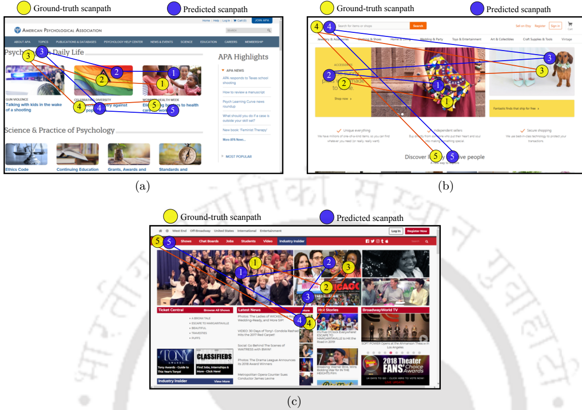
Figure 7.10: Example scanpath predictions
