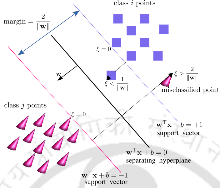
Figure 2.7: Linear SVM illustration for binary classification of classes i and j
