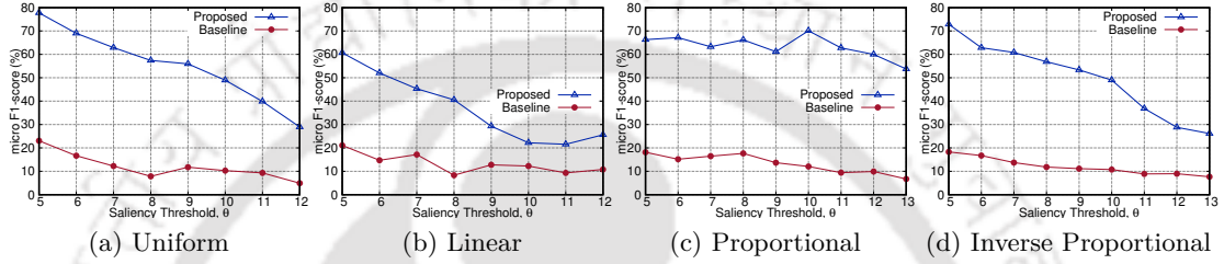
Figure 4.16: Micro F1-scores of four weighting strategies compared with the baseline for varying \theta
