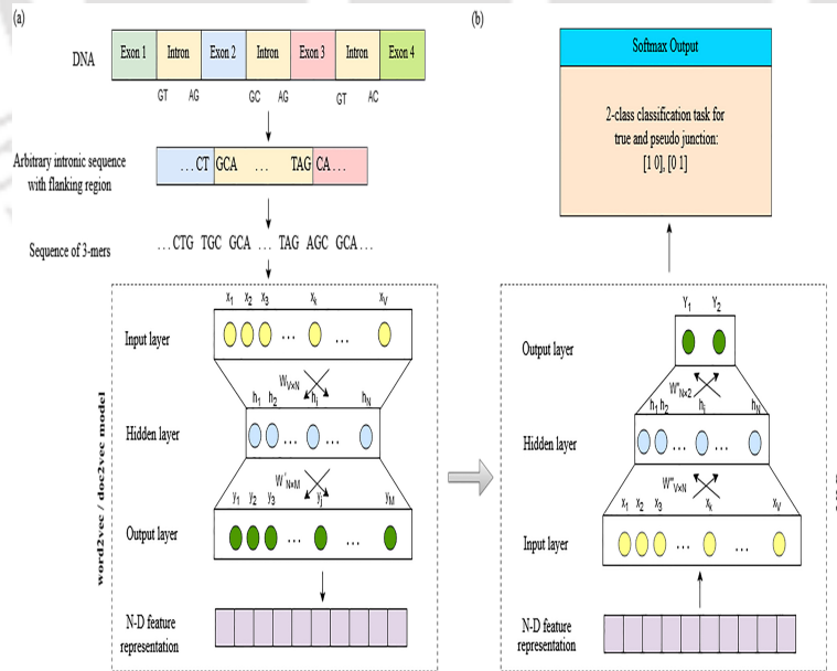
Figure 4.1: Proposed approach: (a) feature representation; (b) splice junction classification.
