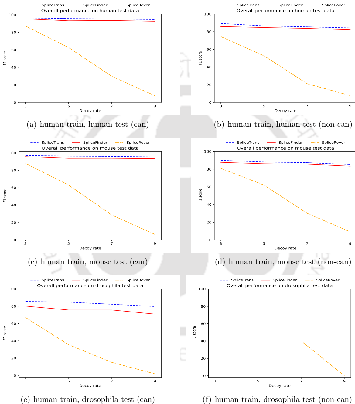
Figure 7.3: F1-score (in percentage) obtained by SpliceTrans, SpliceFinder and SpliceRover in the identification of splice junctions with imbalanced training data.
