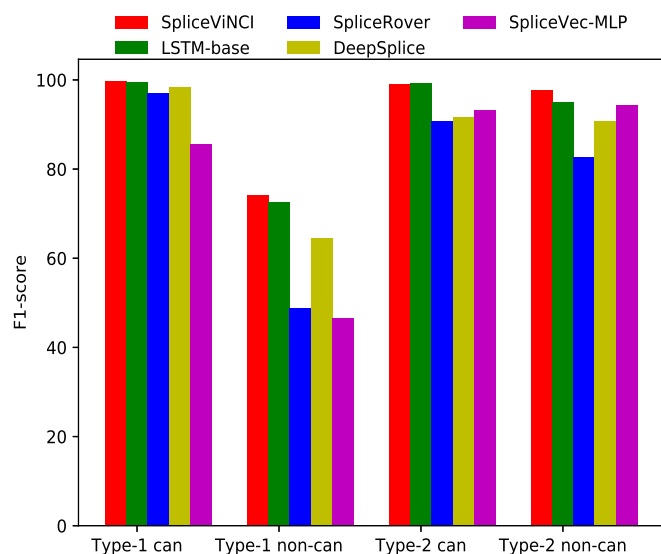
Figure 6.3: Performance of various state-of-the-art models. The performance is measured in terms of F1-score for canonical ( can ) and non-canonical ( non-can ) splice junctions from both Type-1 and Type-2 dataset. F1-score is computed in percentage.
