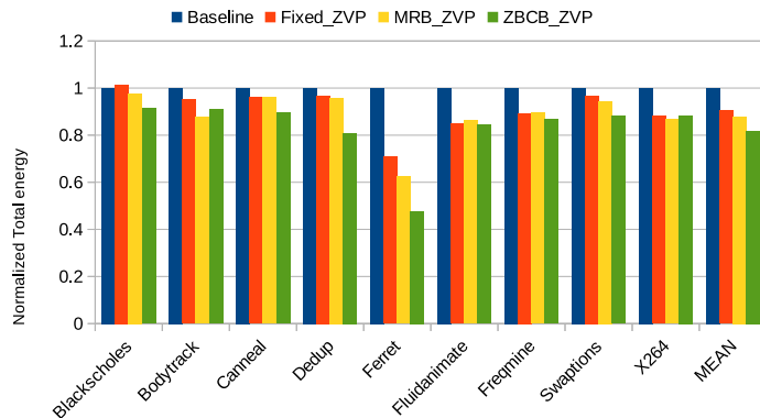
Fig. 3.22 Normalized Total Energy for 2MB LLC at 40µs w.r.t baseline
