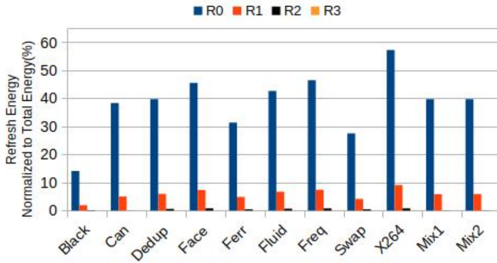
Fig. 6.5 Refresh energy percentage for different retention regions
