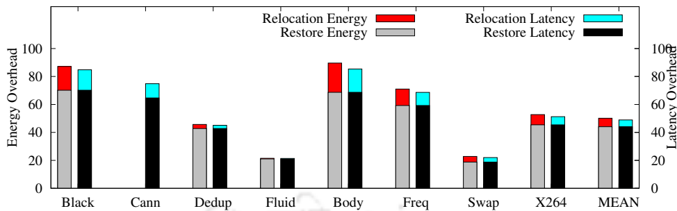
Fig. 5.21 Percentage of energy overhead and latency overhead of CORIDOR(P4) policy over the baseline (HCRR).
