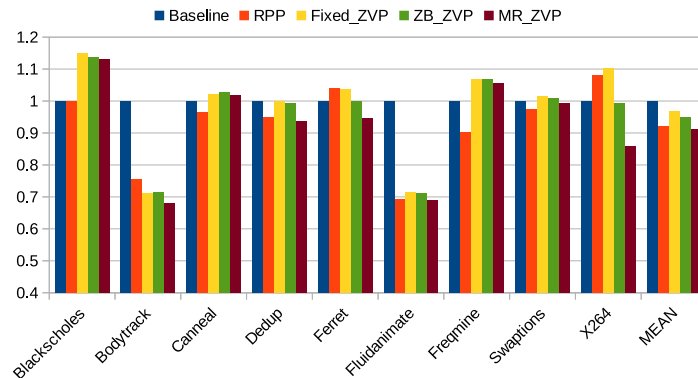
Fig. 3.14 Normalized CPI of proposed policies for 4MB LLC w.r.t baseline and existing RPP policy with 40\mu s retention time
