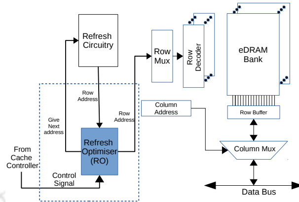
Fig. 4.4 Proposed eDRAM Architecture
