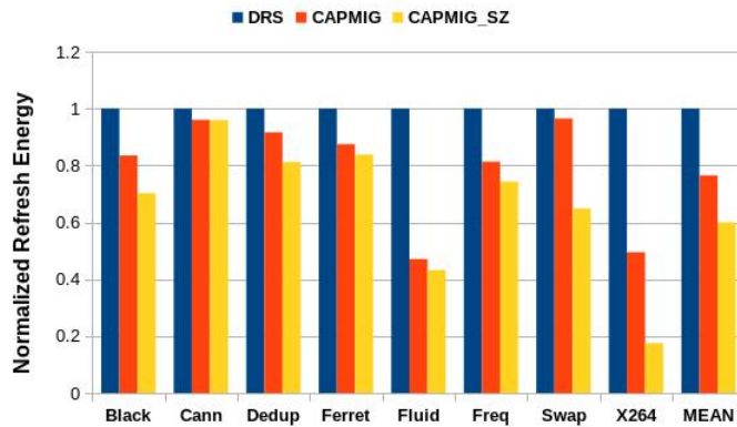
Fig. 6.17 Normalized Refresh Energy for proposed policy w.r.t DRS(lesser is better)
