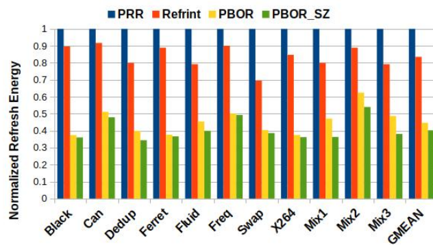
Fig. 4.7 Normalized Refresh Energy of proposed PBOR over PRR
