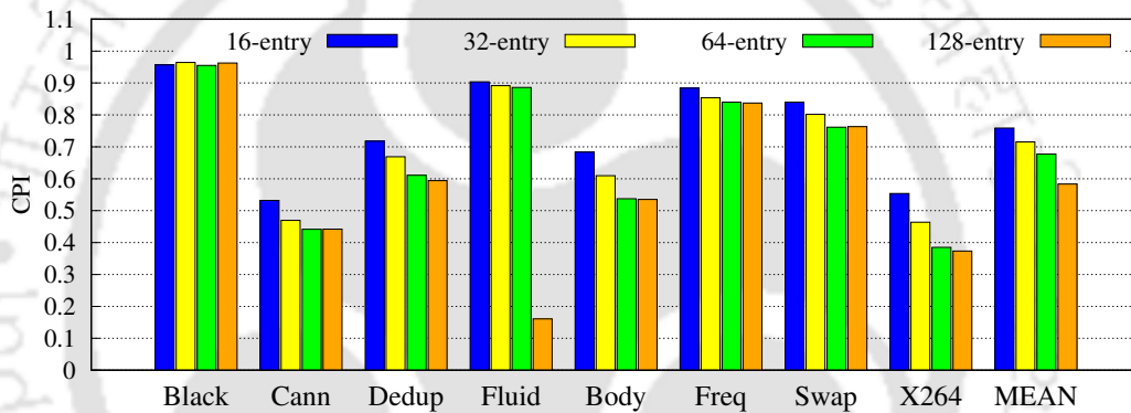
Fig. 5.17 Relative CPI values over different buffer sizes, normalized to HCRR for RD_BUF policy (lower is better).
