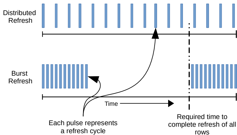
Fig. 2.6 Representation of Distributed and Burst Refresh Mode
