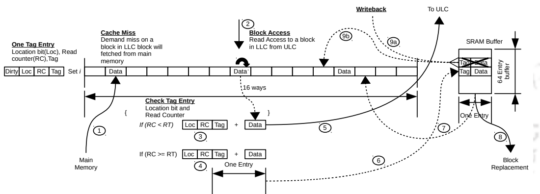
Fig. 5.5 Working Example of RD_BUF policy.
