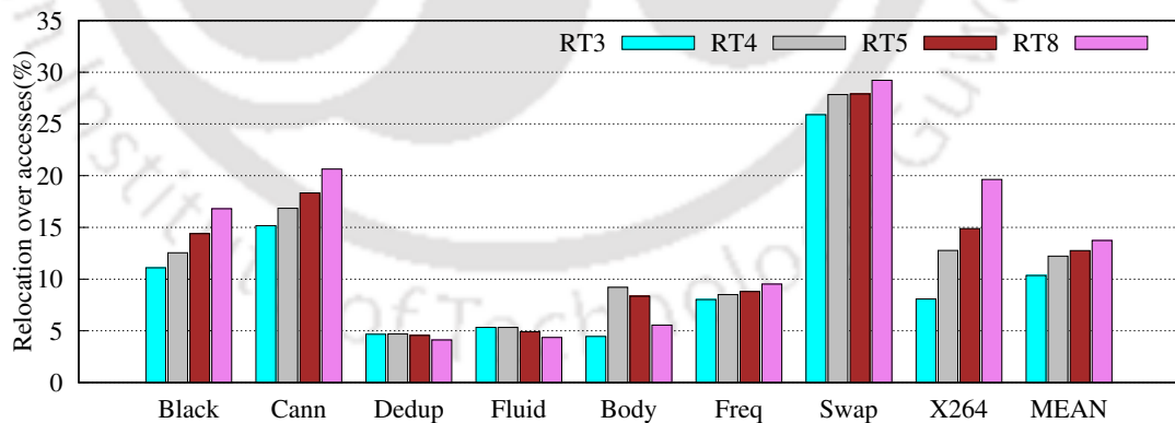
Fig. 5.11 Percentage of read-hits served by read-buffer for different RT values for RD_BUF policy (higher is better).
