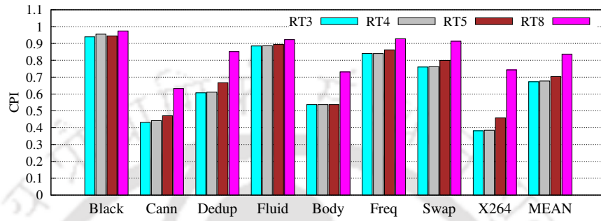
Fig. 5.13 Relative CPI values over different read-threshold values, normalized to HCRR for RD_BUF policy(lower is better).
