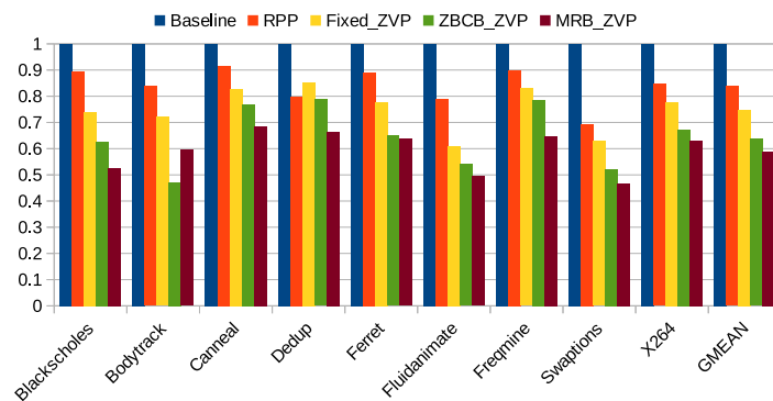
Fig. 3.13 Normalized Refresh Count for 4MB LLC proposed policies w.r.t baseline and Existing RPP policy with 40\mu s retention time
