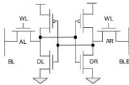
Fig. 2.1 6T SRAM cell schematic.
