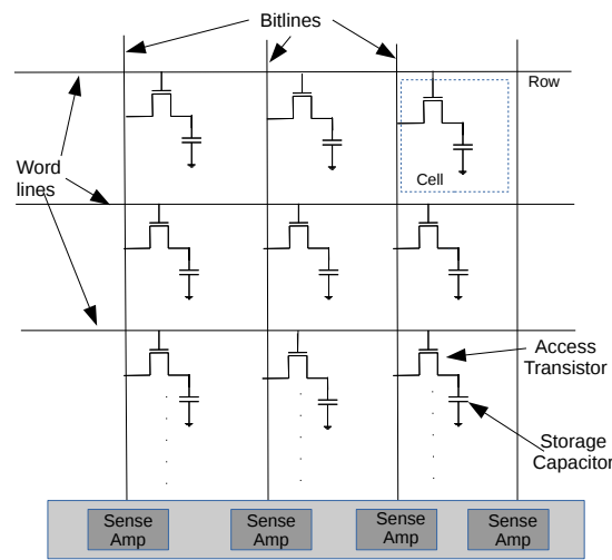
Fig. 2.4 Representational View of eDRAM bank
