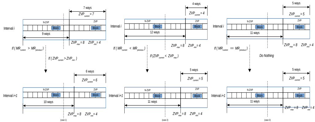
Fig. 3.9 Working example of Miss Rate Based Reconfiguration with different cases.
