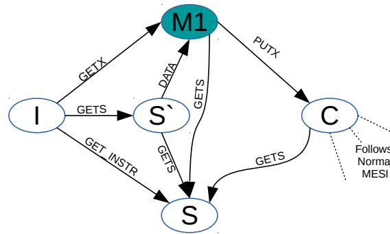
Fig. 4.3 State Diagram showing transitions of states in eDRAM according to the MESI protocol
