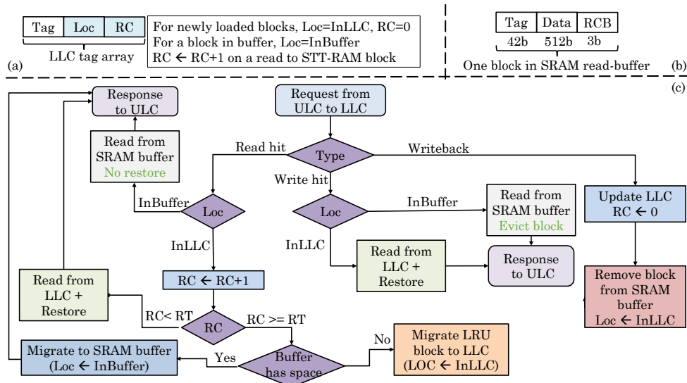
Fig. 5.4 (a) Modified tag array (b) One entry of SRAM buffer (c) Flow-chart of RD_BUF
