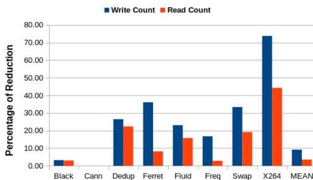
Fig. 6.19 Percentage Reduciton in number of Reads and Writes in CAPMIG_SZ wrt CAPMIG
