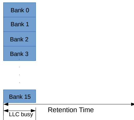
Fig. 2.15 Diagram Representing a LLC containing 16 banks and all the banks triggers refresh operation in burst mode.
