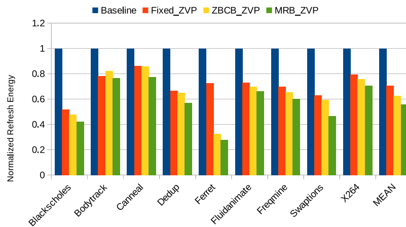
Fig. 3.21 Normalised Refresh Energy for 2MB LLC w.r.t baseline with 40\mu s
