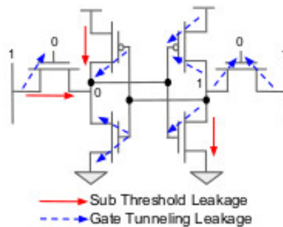
Fig. 2.2 SRAM leakage paths.
