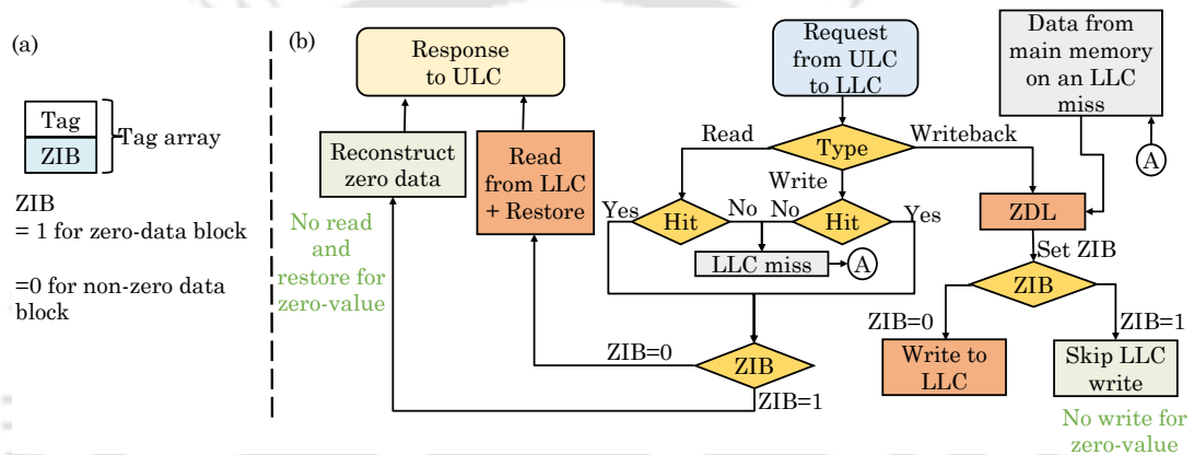
Fig. 5.7 (a) Modification to the tag array (b) Flow-chart for the SKIP_ZERO policy.
