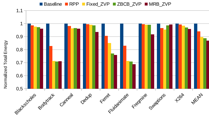
Fig. 3.15 Total energy consumption of 4MB LLC of proposed policies w.r.t baseline with 40\mu s retention time
