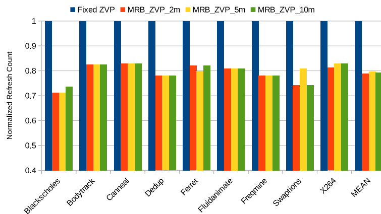
Fig. 3.17 Normalized Refresh Count for different interval for 4MB LLC in Miss Rate Based Policy
