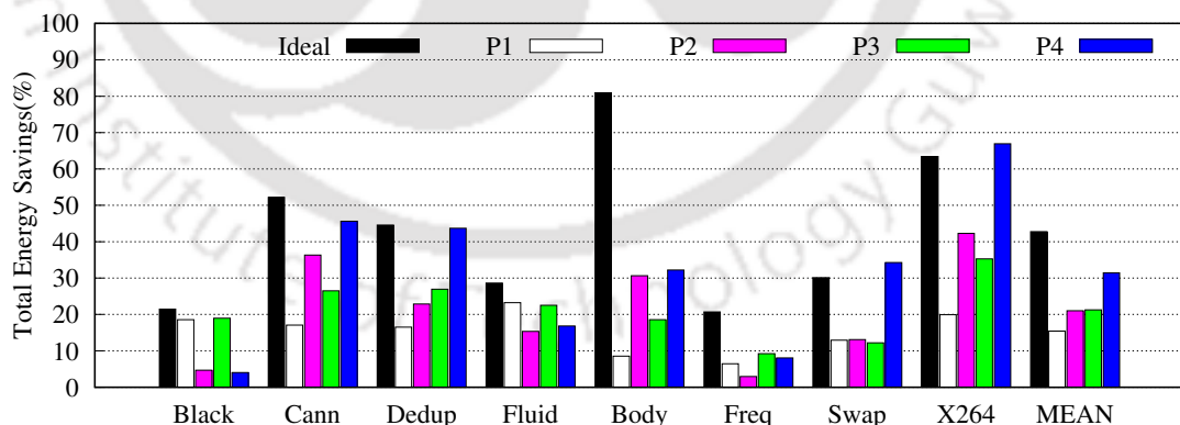
Fig. 5.8 Total energy savings for different benchmarks over the HCRR policy (higher is better)
