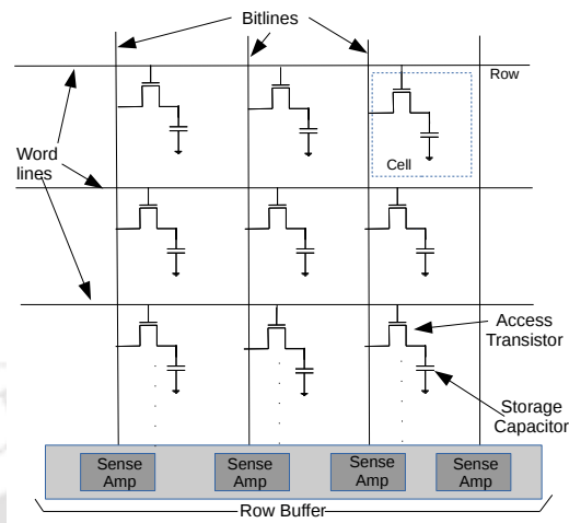
Fig. 3.2 Abstract Diagram of an eDRAM bank
