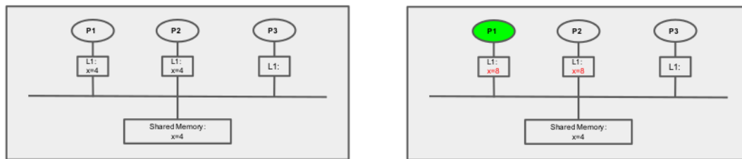
Fig. 2.10 Write-Update Policy After condition
