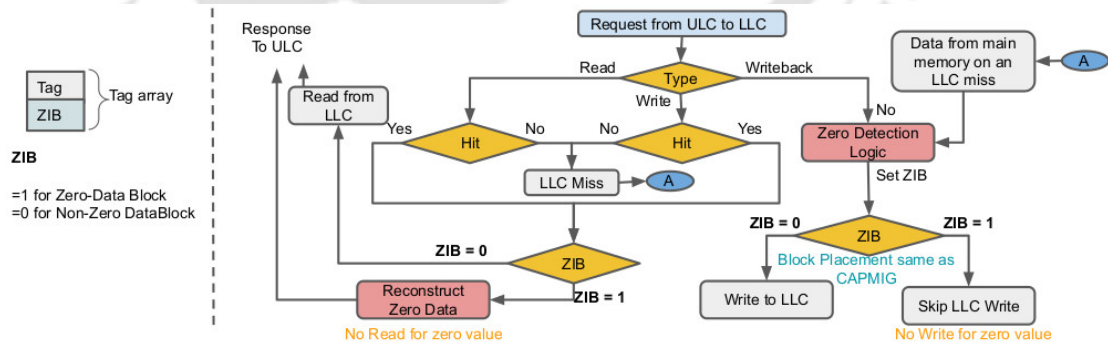
Fig. 6.13 Flow-chart for the CAPMIG_SZ policy. We can see additional modification to the tag array(at bottom).
