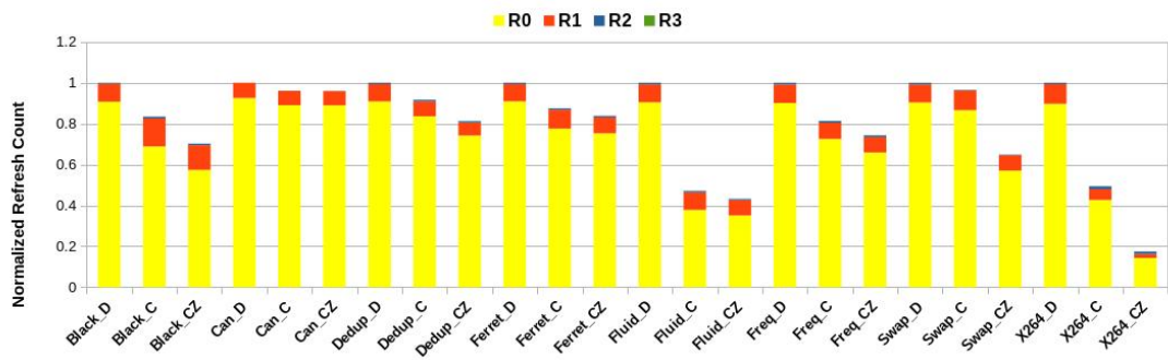
Fig. 6.16 Region wise normalised Refresh Counts for proposed policy CAPMIG (_C) and CAPMIG_SZ (_CZ) w.r.t DRS with random allocation. (_D).
