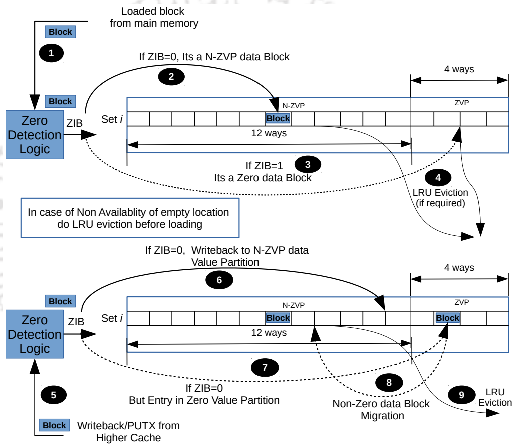
Fig. 3.6 Working Example of Fixed Zero Value Partition Refreshing
