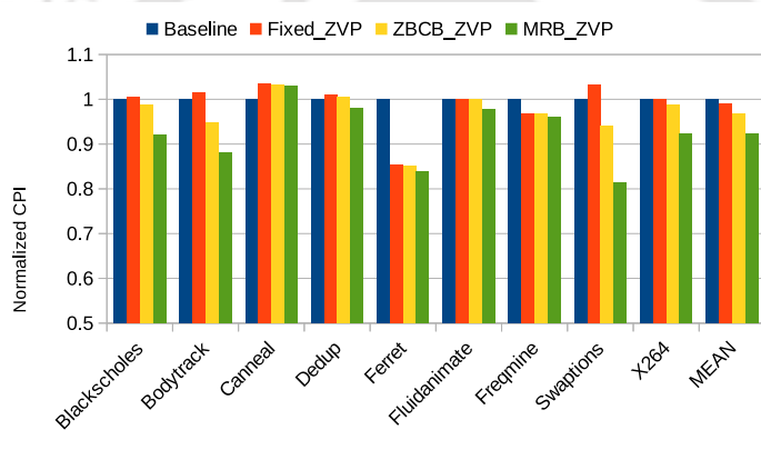
Fig. 3.23 Normalized CPI for 4MB LLC with 50µs Retention time
