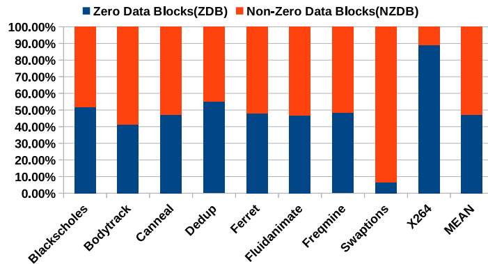
Fig. 3.1 Percentage of Zero Data Blocks and Non-Zero Data blocks for various benchmarks
