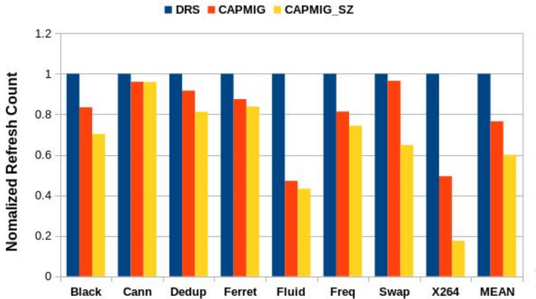
Fig. 6.14 Refresh count of CAPMIG policy normalized w.r.t. random placement policy.(lesser is better)
