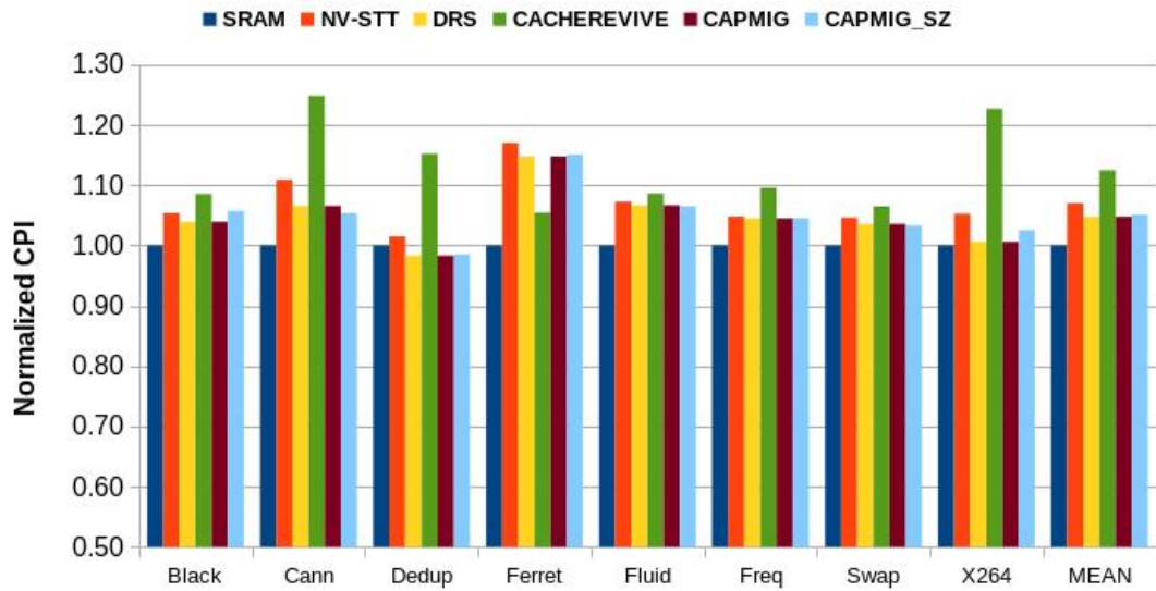
Fig. 6.15 Performance of various policies normalised with baseline SRAM (lesser is better).
