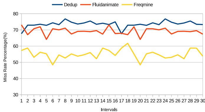
Fig. 3.7 Variation of miss rate during execution. Here Y-axis shows the overall miss rate for the application during execution after a specific interval. X-axis represents different intervals.
