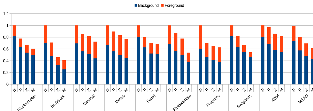
Fig. 3.19 Normalized Refresh Count for 4MB LLC with 50µs retention time
