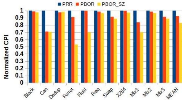
Fig. 4.6 Normalized CPI for PRR and PBOR
