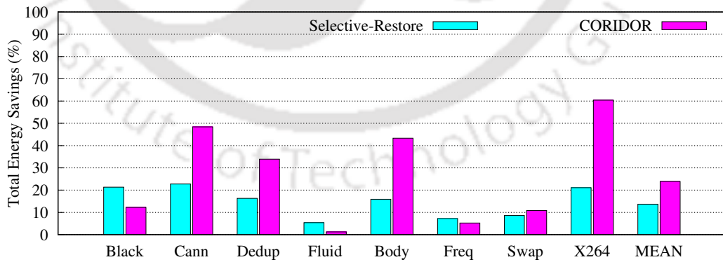
Fig. 5.20 Total energy savings of “selective restore” and CORIDOR normalized to HCCR policy (higher is better).
