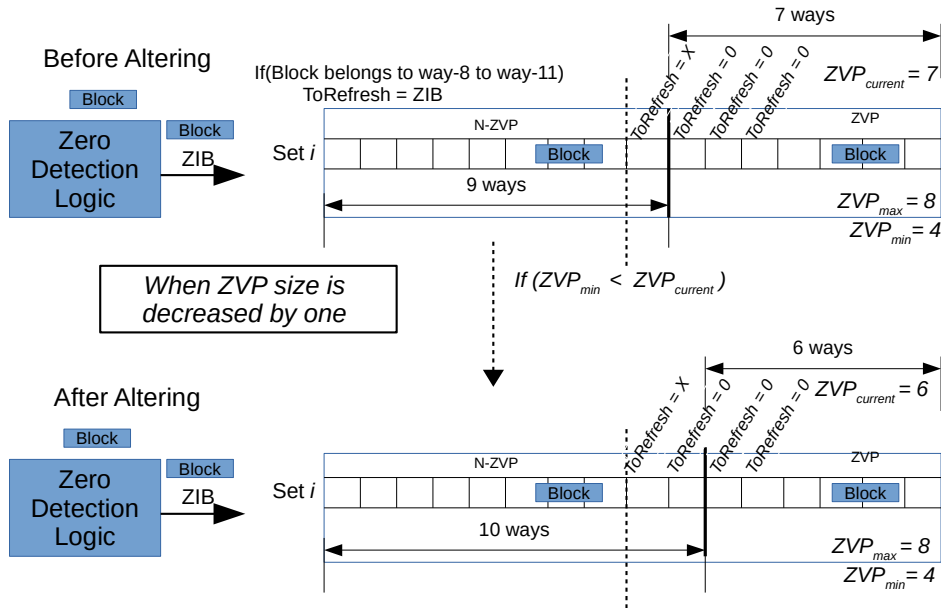
Fig. 3.11 Altering of ZVP when size decreases
