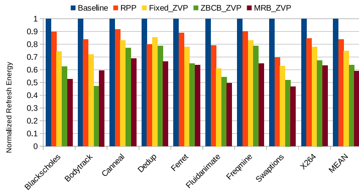
Fig. 3.16 Normalised Refresh Energy for 4MB LLC w.r.t baseline and existing RPP policy with 40\mu s
