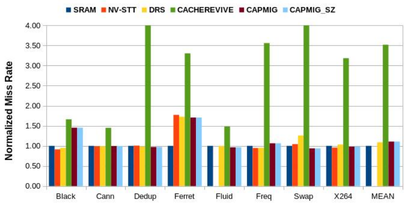
Fig. 6.18 Miss Rate of proposed policy normalized w.r.t SRAM
