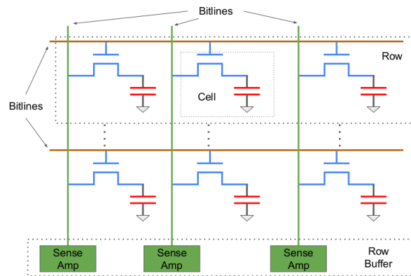
Fig. 2.3 DRAM bank structure
