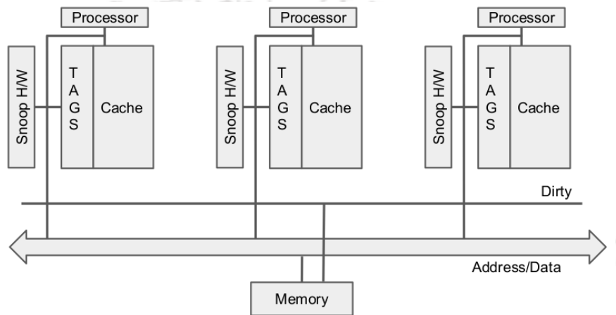
Fig. 2.13 Snoopy Protocol
