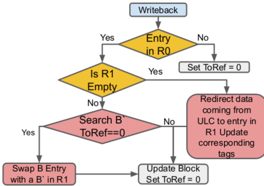
Fig. 6.9 Flow Chart of operations performed on writeback.
