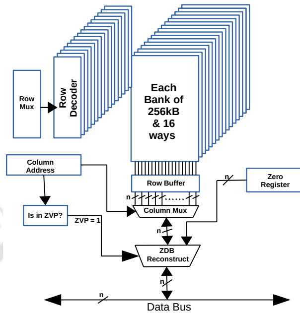
Fig. 3.5 High-level Diagram of the proposed architecture.
