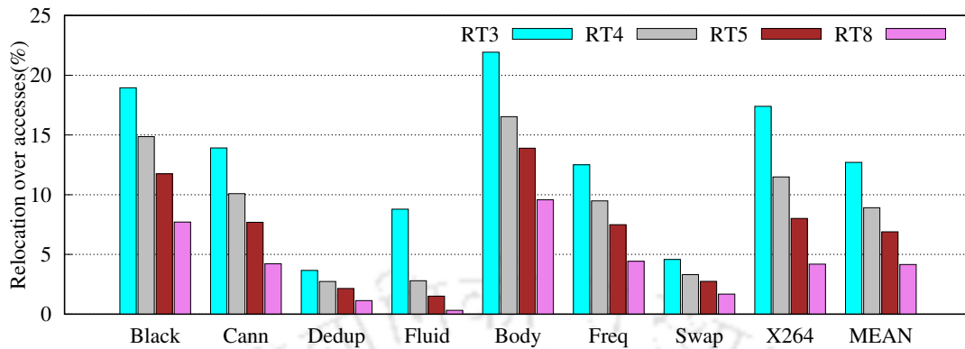
Fig. 5.12 Percentage of migration to the read-buffer over total accesses for RD_BUF policy (higher is better).
