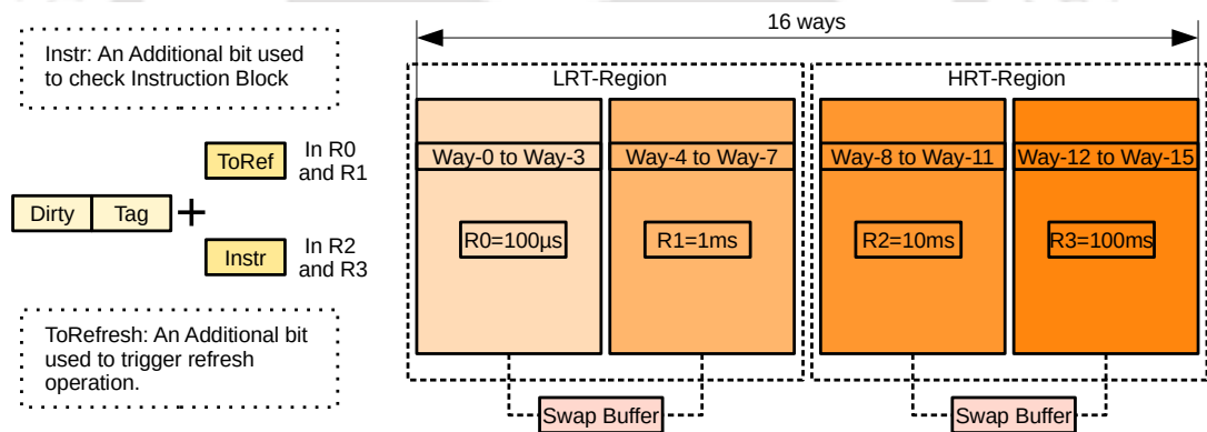
Fig. 6.6 CAPMIG: Proposed multi-retention based LLC Cache Architecture
