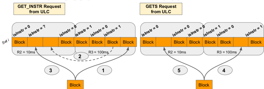
Fig. 6.10 Operations performed on GETS and GET_INSTR request from ULC.
