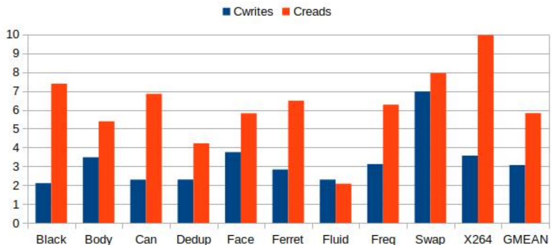
Fig. 6.4 The average consecutive reads (CReads) and consecutive writes (CWrites) on the blocks in a bank for different benchmarks.
