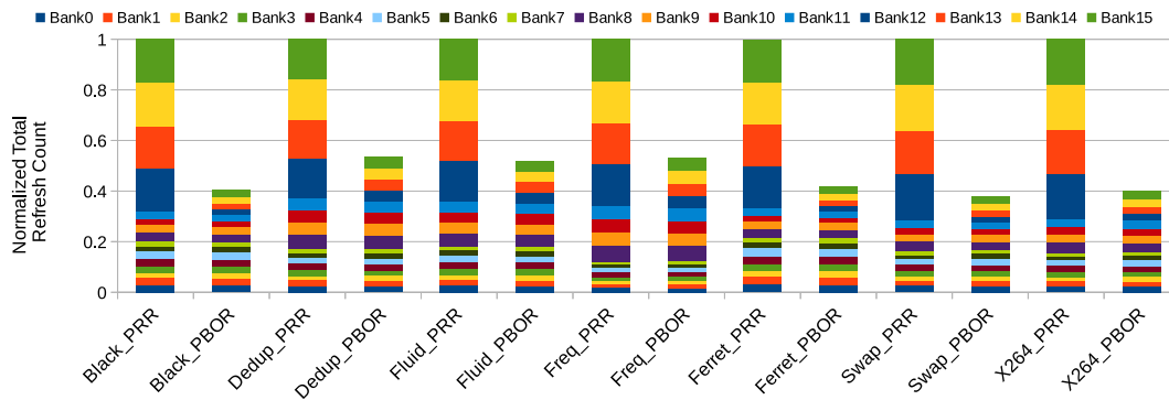
Fig. 4.8 Bankwise Normalized Refresh Counts of PBOR and PRR
