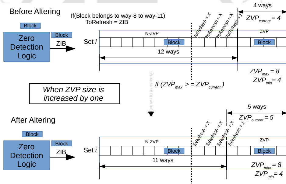
Fig. 3.10 Reconfiguration of ZVP when size increases
