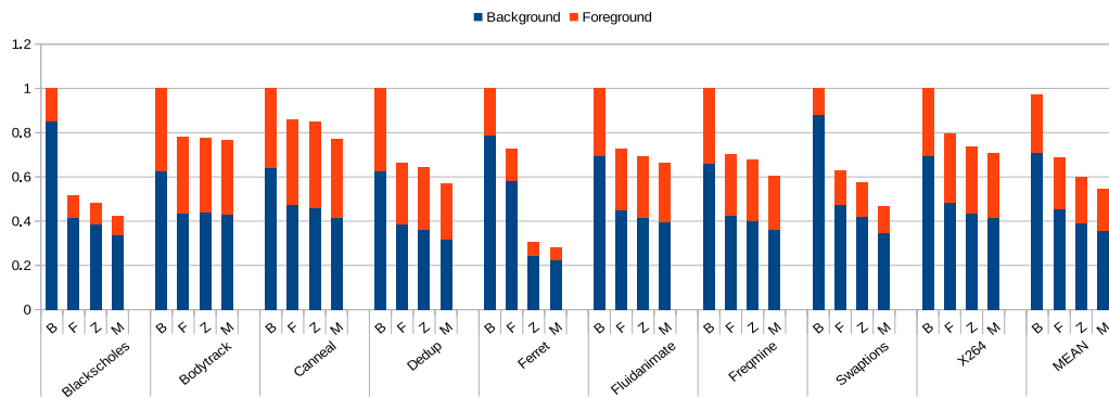
Fig. 3.20 Normalized Refresh Count for 2MB LLC at 40\mu s
