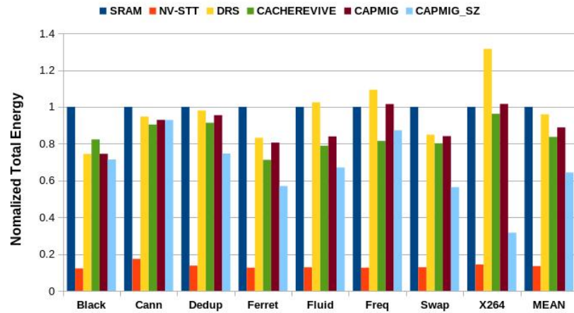
Fig. 6.20 Total Energy normalized to baseline
