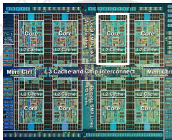
Fig. 1.2 IBM POWER7 CPU with eDRAM
