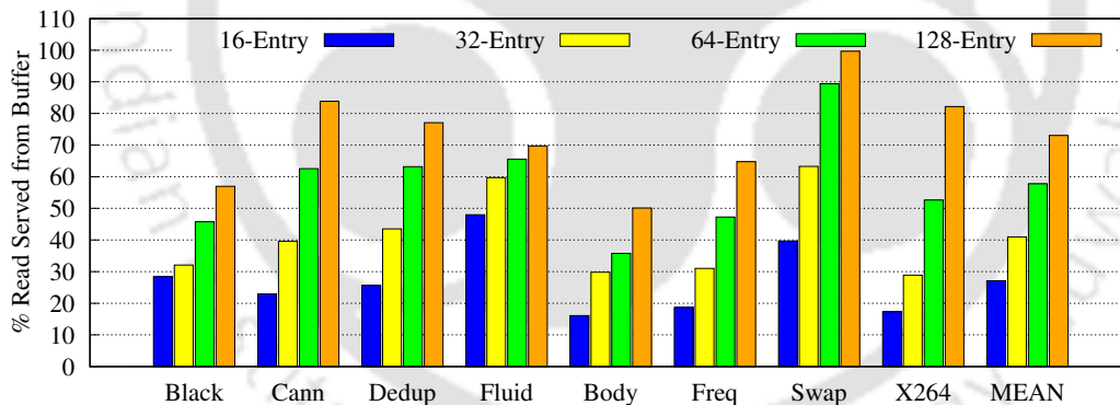
Fig. 5.15 Percentage of reads served by the read buffer for different buffer sizes for RD_BUF policy.
