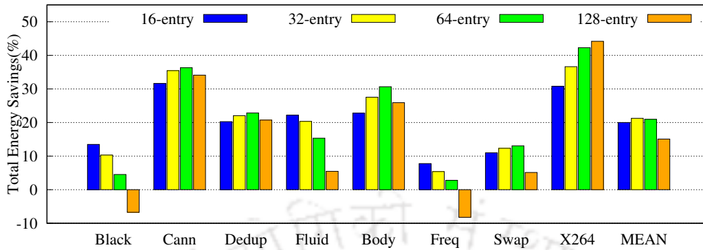
Fig. 5.18 Total energy savings for different benchmarks over various Buffer Sizes normalized to HCRR policy for RD_BUF (higher is better)
