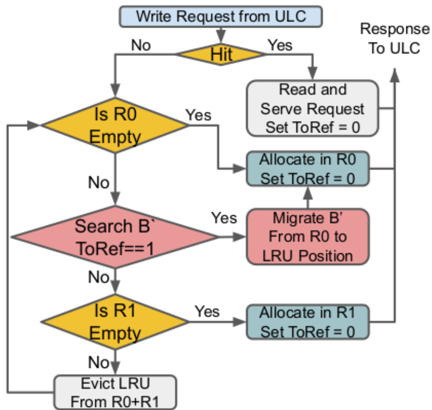
Fig. 6.8 Flow chart of operations performed on Write Request
