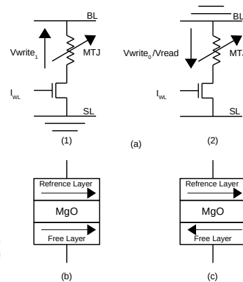
Fig. 2.5 Overview of STT-RAM cell (a) Schematic STT view with (1) Write '1' operation (2) Write '0' and Read operation (b) Parallel low resistance, representing '0' state (c) Anti-parallel high resistance, representing '1' state
