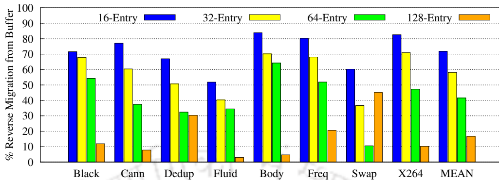
Fig. 5.16 Percentage of reverse migrations (block eviction) from the read buffer for different buffer sizes for RD_BUF policy.
