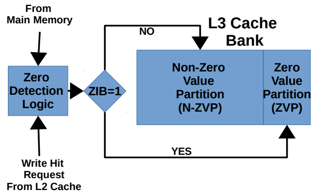
Fig. 3.4 Diagram of Fixed Zero Value Partition Based Refresh Technique
