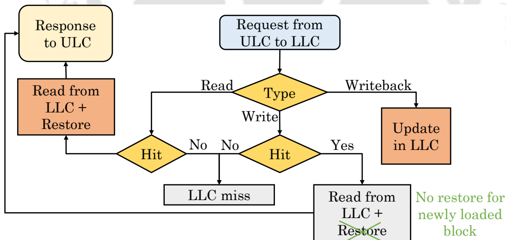
Fig. 5.2 Flow-chart of SKIP_WH
