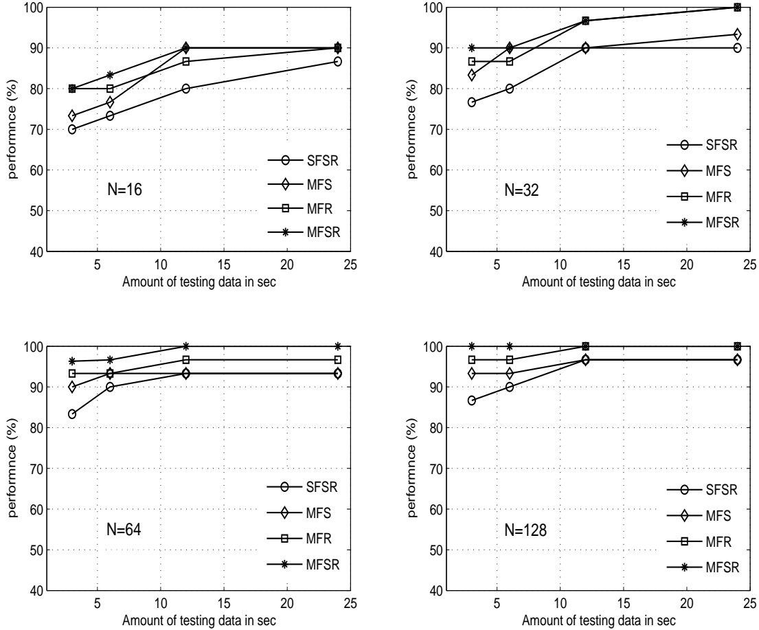
Figure 3.7: Performance of the speaker recognition system based on SFSR and MFSR analysis techniques for different sizes of testing data for the first 30 speakers taken from the YOHO database. The amount of training data is 25 sec in all cases.
