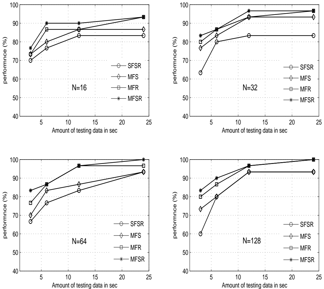
Figure 3.10: Performance of the speaker recognition system based on SFSR and MFSR analysis techniques for different sizes of testing data for 30 speakers taken from the YOHO database. MFS trained model is used for testing.
