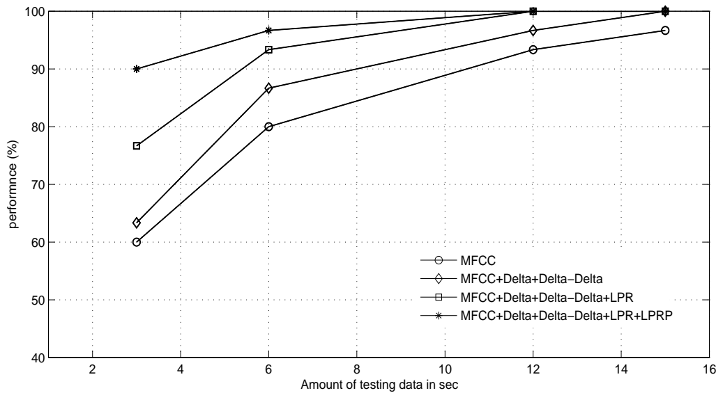
Figure 4.5: Performance of the speaker recognition system for MFCC and different combined system for different sizes of training and testing data for the first 30 speakers taken from the TIMIT database.
