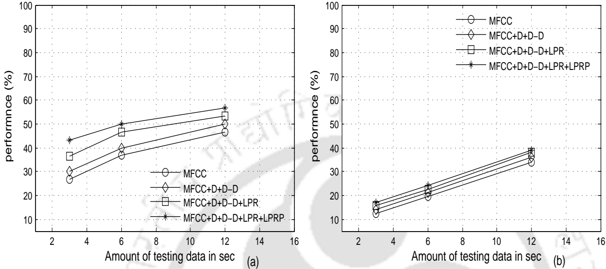
Figure D.2: Performance of the individual and combination of features speaker recognition system for (a) the first 30 speakers (b) the 138 speakers taken from the NIST-SRE-2003 database.
