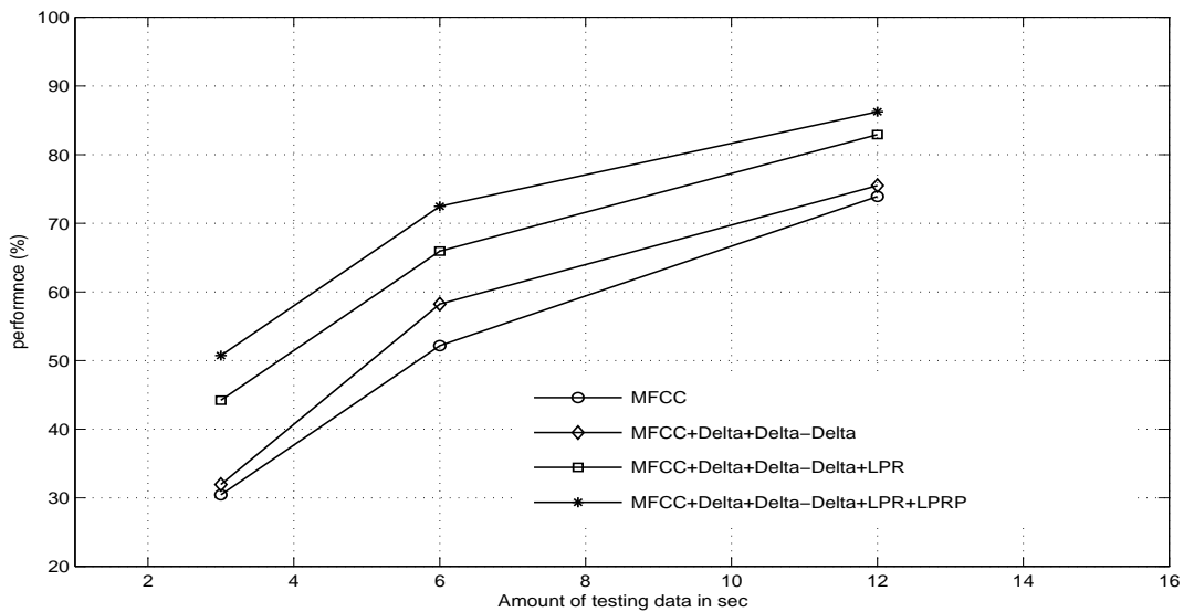
Figure 4.6: Performance of the speaker recognition system for MFCC and different combined system for different sizes of training and testing data for the first 138 speakers taken from the TIMIT database.
