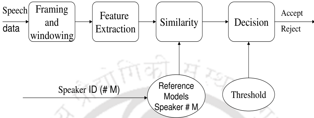
Figure 1.3: Block diagram of speaker verification system.
