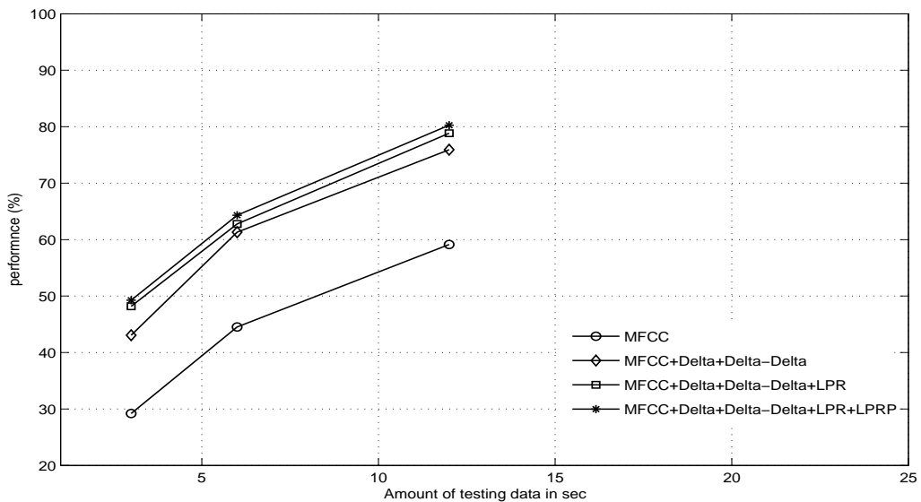
Figure 4.4: Performance of the speaker recognition system for MFCC and different combined system for different sizes of training and testing data for 138 speakers taken from the YOHO database.
