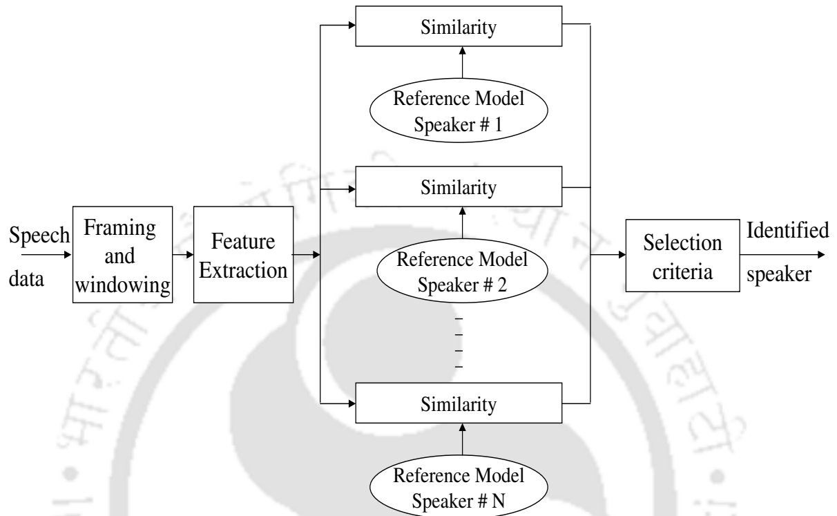
Figure 1.1: Block diagram of closed-set speaker identification system.
