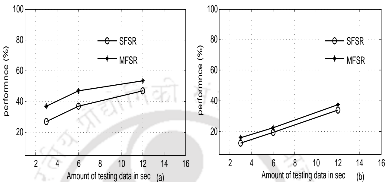
Figure D.1: Performance of the SFSR and MFSR analysis techniques speaker recognition system for (a) the first 30 speakers (b) the 138 speakers taken from the NIST-SRE-2003 database.
