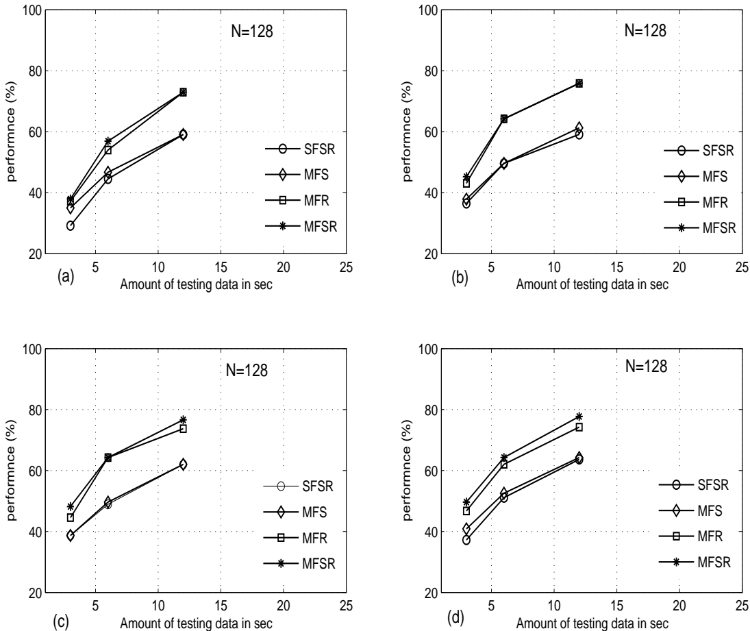
Figure 3.13: Performance of the speaker recognition system based on SFSR and MFSR analysis techniques for different sizes of testing data for 138 speakers. (a) SFSR trained model is used for testing (b) MFS trained model is used for testing (c) MFR trained model is used for testing and (d) MFSR trained model is used for testing.
