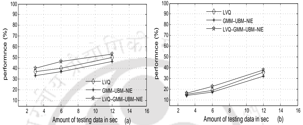
Figure D.3: Performance of the individual and combined modelling techniques speaker recognition system for (a) the first 30 speakers (b) the 138 speakers taken from the NIST-SRE-2003 database.
