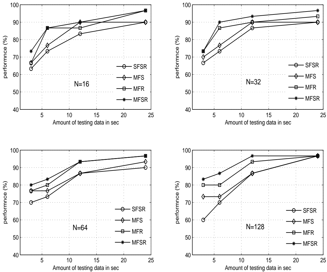
Figure 3.9: Performance of the speaker recognition system based on SF SR and MFSR analysis techniques for different sizes of testing data for the first 30 speakers taken from the YOHO database. SF SR trained model is used for testing.
