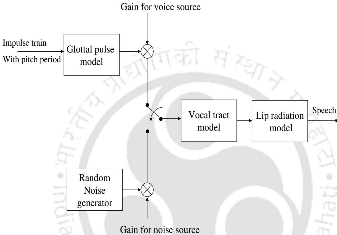
Figure A.2: The representation of the speech production mechanism.
