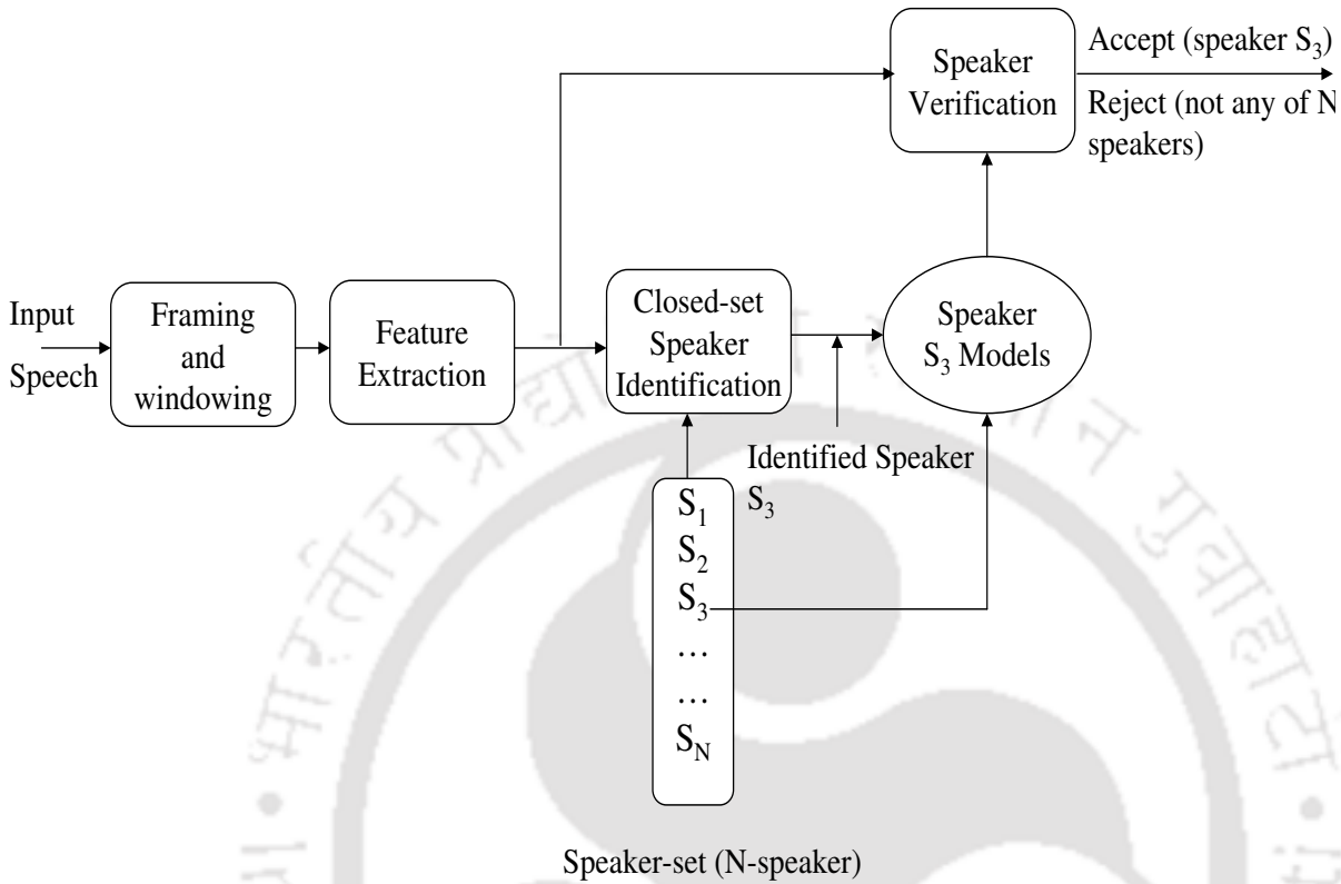
Figure 1.2: Block diagram of open-set speaker identification system.
