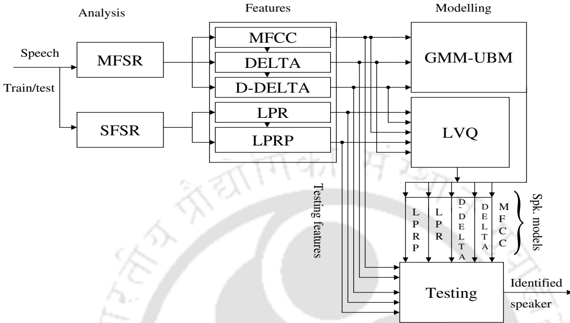
Figure 6.1: Block diagram of integrated systems based speaker recognition for limited data condition.
