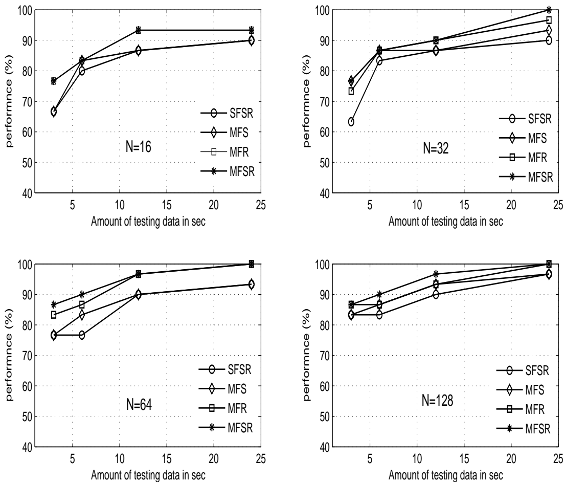
Figure 3.11: Performance of the speaker recognition system based on SFSR and MFSR analysis techniques for different sizes of testing data for 30 speakers taken from the YOHO database. MFR trained model is used for testing.
