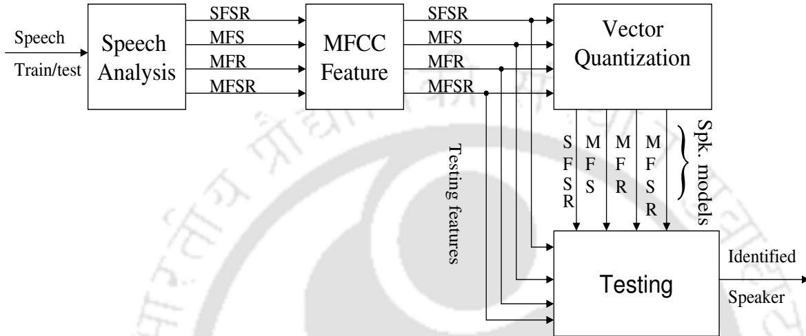
Figure 3.4: The SFSR and proposed MFSR based speaker recognition system for limited data condition
