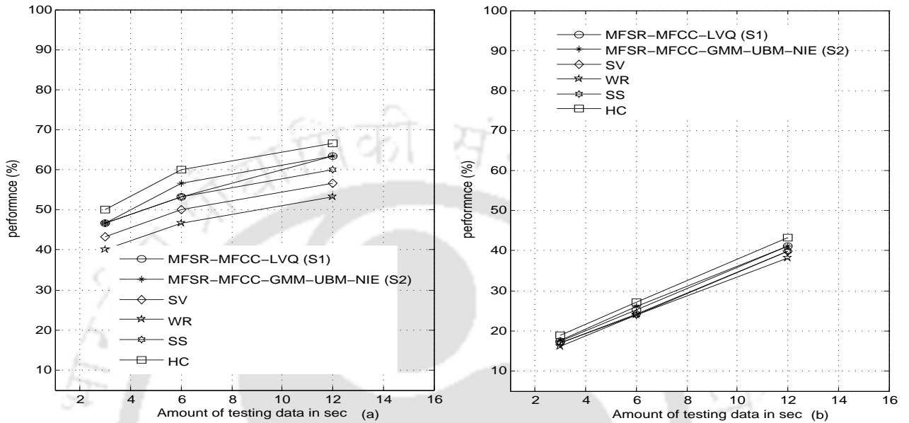
Figure D.5: Performance of the integrated and combination techniques speaker recognition systems for (a) the first 30 speakers (b) the 138 speakers taken from the NIST-SRE-2003 database.
