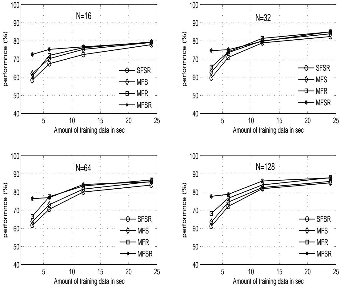
Figure 3.5: Performance of the speaker recognition system based on SFSR and MFSR analysis techniques for different sizes of training data for the first 30 speakers taken from the YOHO database. The amount of test data is about 80 sec in all cases.
