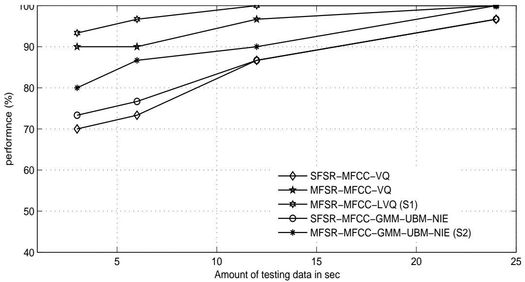
Figure 6.2: Speaker recognition performance for the baseline, individual and integrated systems for different sizes of training and testing data for the first 30 speakers taken from the YOHO database.
