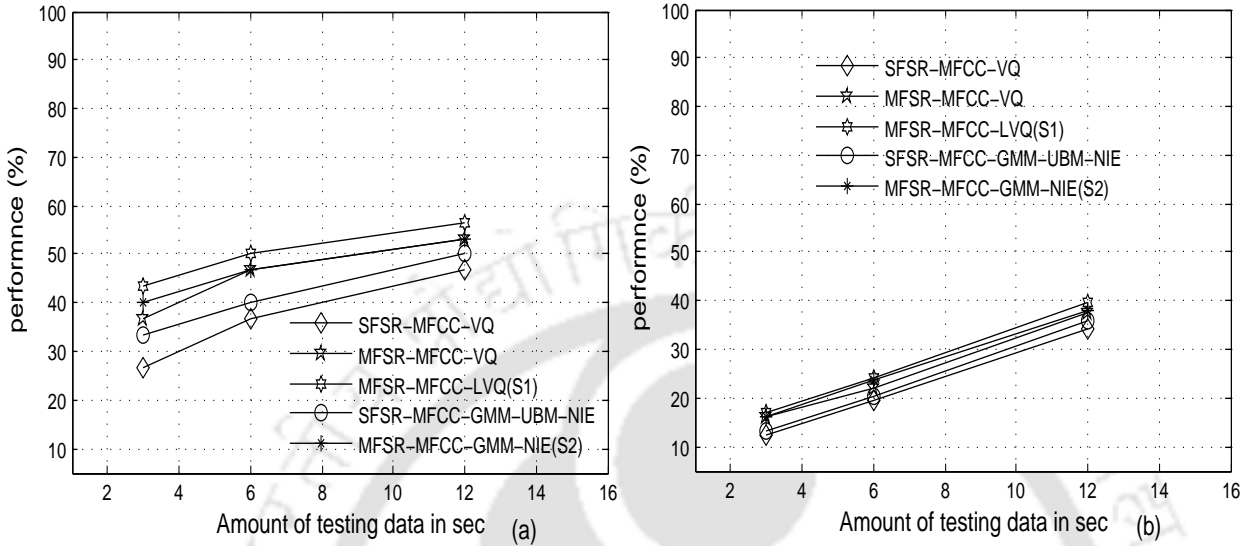
Figure D.4: Performance of the integrated speaker recognition systems for (a) the first 30 speakers (b) the 138 speakers taken from the NIST-SRE-2003 database.
