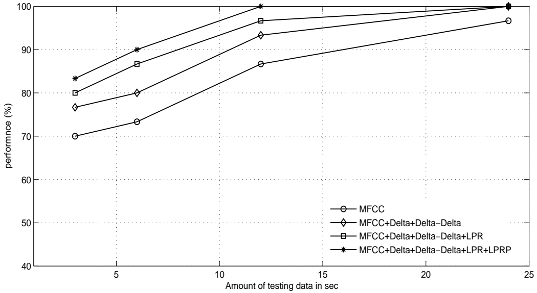
Figure 4.3: Performance of the speaker recognition system for MFCC and different combined system for different sizes of training and testing data for the first 30 speakers taken from the YOHO database.
