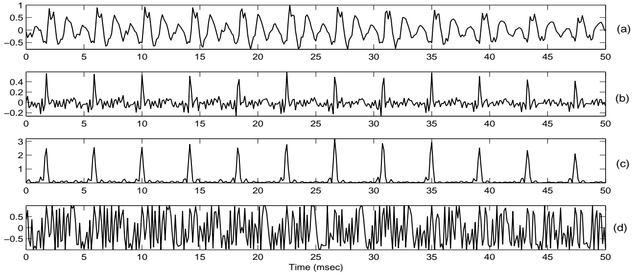
Figure 4.2: Difference between LPR and LPRP: (a) a segment of speech signal, (b) corresponding LP residual, (c) Hilbert envelope (HE) of LP residual and (d) corresponding LP residual phase.
