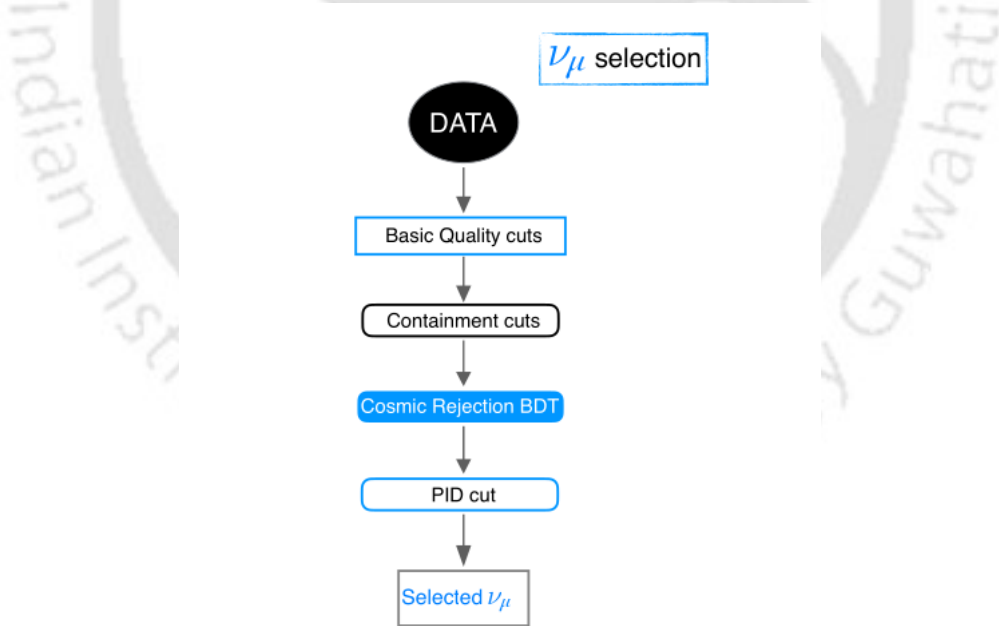
Figure 5.20: Flowchart showing the cut flow for the \nu_\mu -selection.
