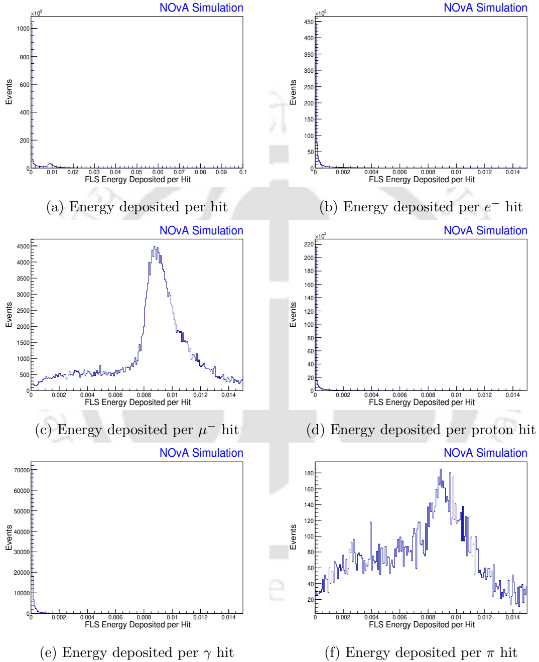
Figure 4.13: FLS hit energy deposition distributions for different particles
