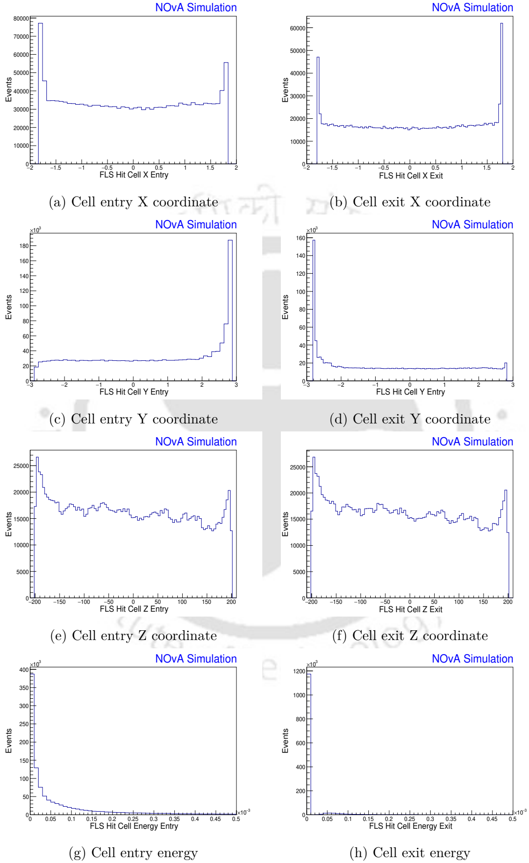
Figure 4.14: Entry and exit distributions of the particles from the cell in the detector.
