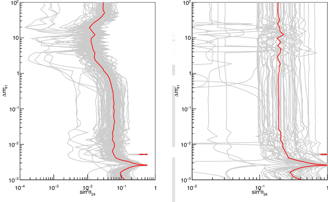
Figure 7.9: Median sensitivities at 90% CL (red) with individual pseudoexperiment sensitivity contours at 90% CL (grey). Left: \sin^2 \theta_{24} vs \Delta m_{41}^2 , Right: \sin^2 \theta_{34} vs \Delta m_{41}^2 .
