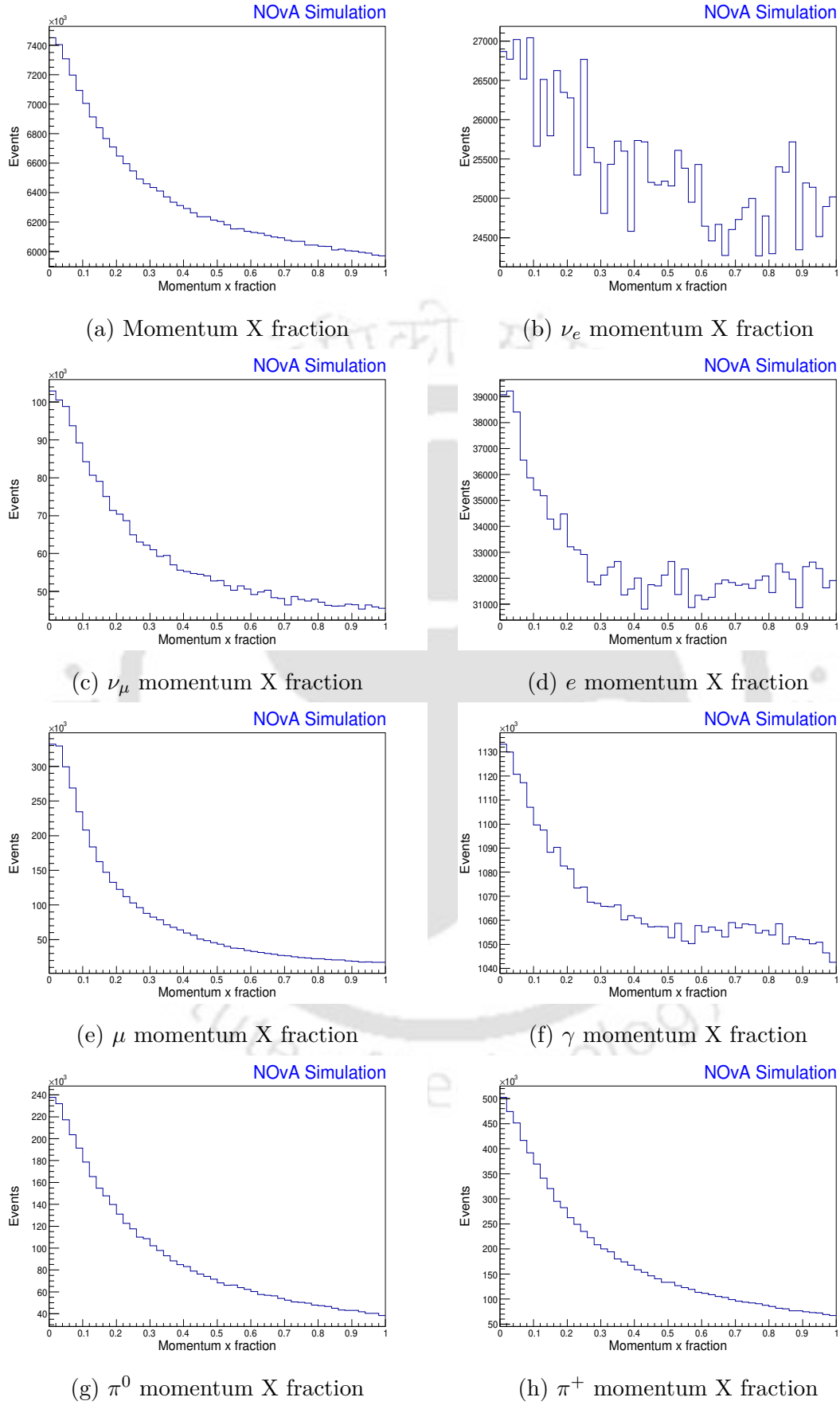
Figure 4.9: Geant4 X momentum distributions
