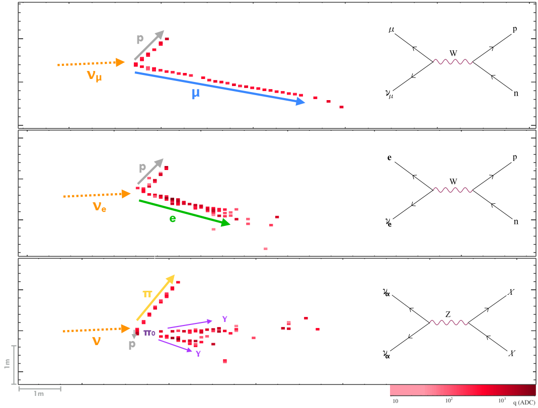
Figure 5.2: Topologies of different neutrino events from NOvA data at ND. At the top, we have \nu_\mu -CC interaction producing a straight long track representing the outgoing muon. In the middle is the \nu_e -CC interaction, producing a short, fuzzy track characterising the outgoing electron. At the bottom is \nu -NC interaction resulting in the production of a \pi^0 , which further decays into two photons. [66]
