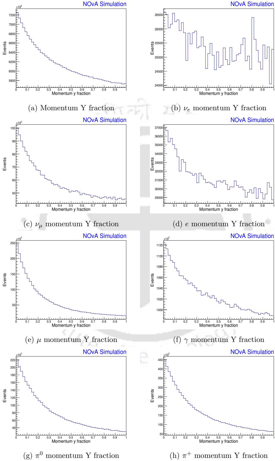
Figure 4.10: Geant4 Y momentum distributions
