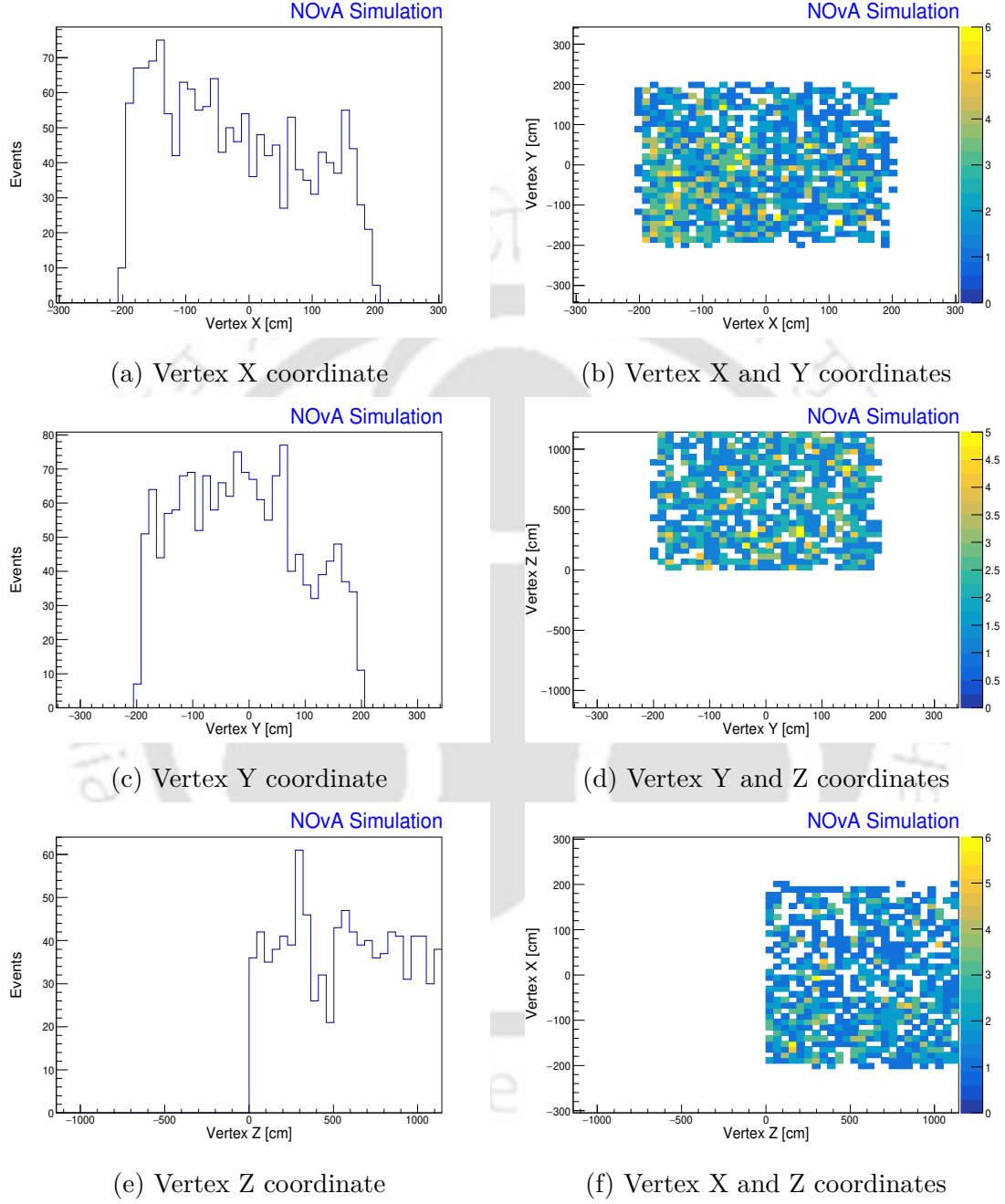
Figure 4.3: 1D vertex distribution showing the event distribution for the MC simulated particles and 2D vertex distributions showing the distribution of MC particles.
