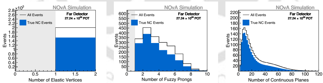
Figure 5.12: Distributions for the Quality Selection Variables for the FHC ( \nu ) mode. The true NC events are highlighted in blue, and the proposed regions to remove are shown as grey boxes.
