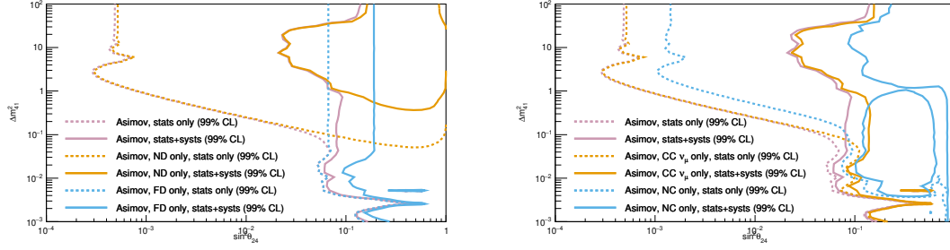
Figure 7.7: Asimov sensitivities for \sin^2 \theta_{24} vs \Delta m^2_{41} at 99% CL with dashed contours representing the stats only and solid ones for stats with systematics. Left: A comparison of the two-detector sensitivity (pink) with the ND-only (orange) and FD-only (blue) sensitivities. Right: A comparison of the full sensitivity (pink) with the \nu_\mu CC-only (orange) and the NC-only (blue) sensitivities.
