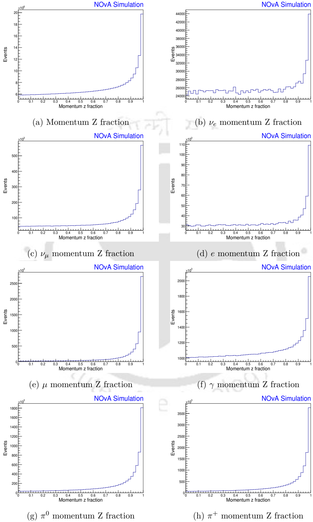
Figure 4.11: Geant4 Z momentum distributions
