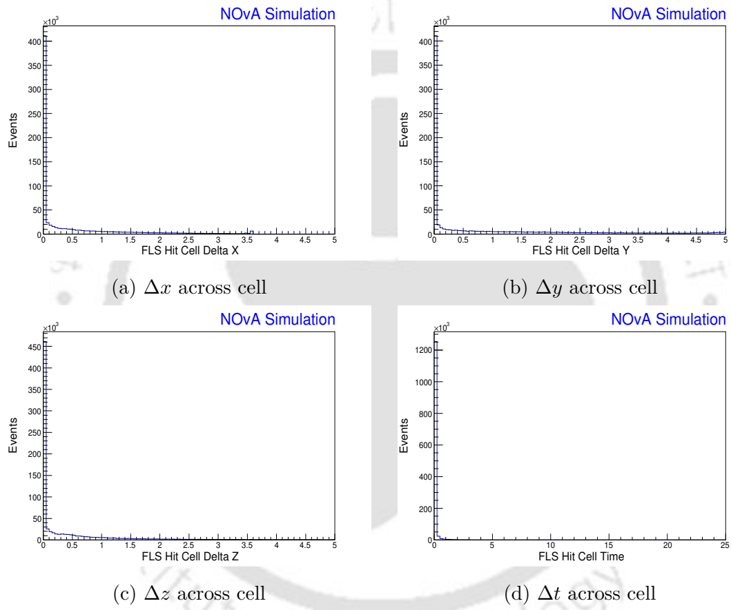
Figure 4.15: FLS hit distance distributions
