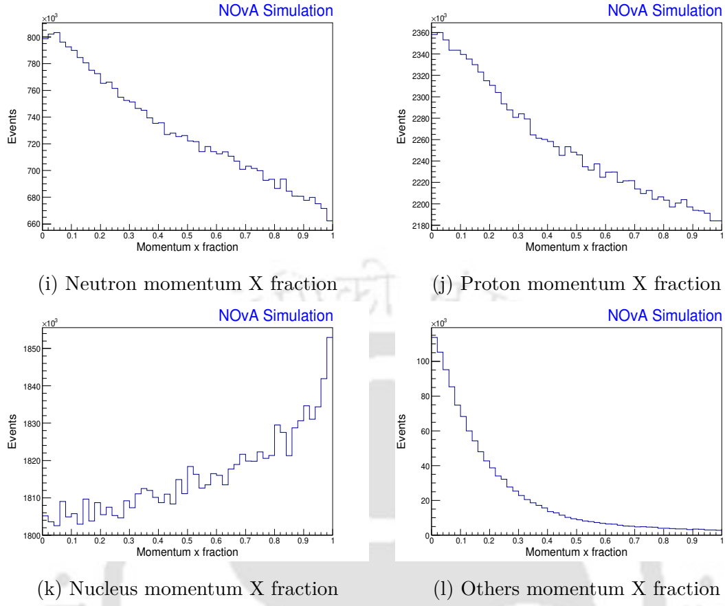
Figure 4.9: X momentum fraction distribution of all the particles processed through GEANT4
