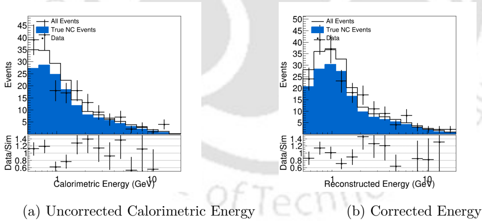
Figure 5.11: Data/simulation comparisons for the uncorrected calorimetric energy on the left and the corrected energy on the right for RHC mode. Here, the true NC events are in blue, and the suggested regions to remove are shown as grey boxes. Note that the simulation has been area-normalised to match the data. In these plots, the quality requirements (Sec. 5.3.2.1), vertex (Sec. 5.3.2.3), fiducial (Sec. 5.3.2.4) volume, and CVN (Sec. 5.3.2.5) criteria have been applied.
