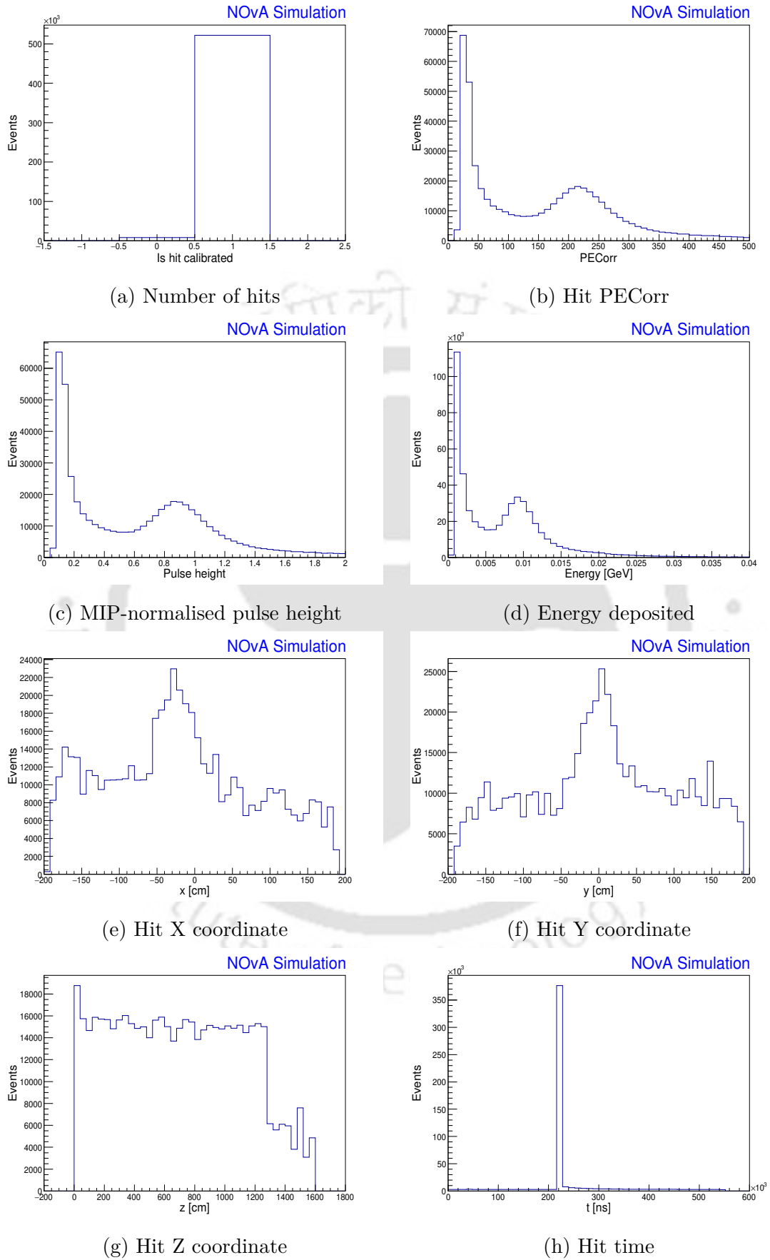
Figure 4.19: Reco hit distributions
