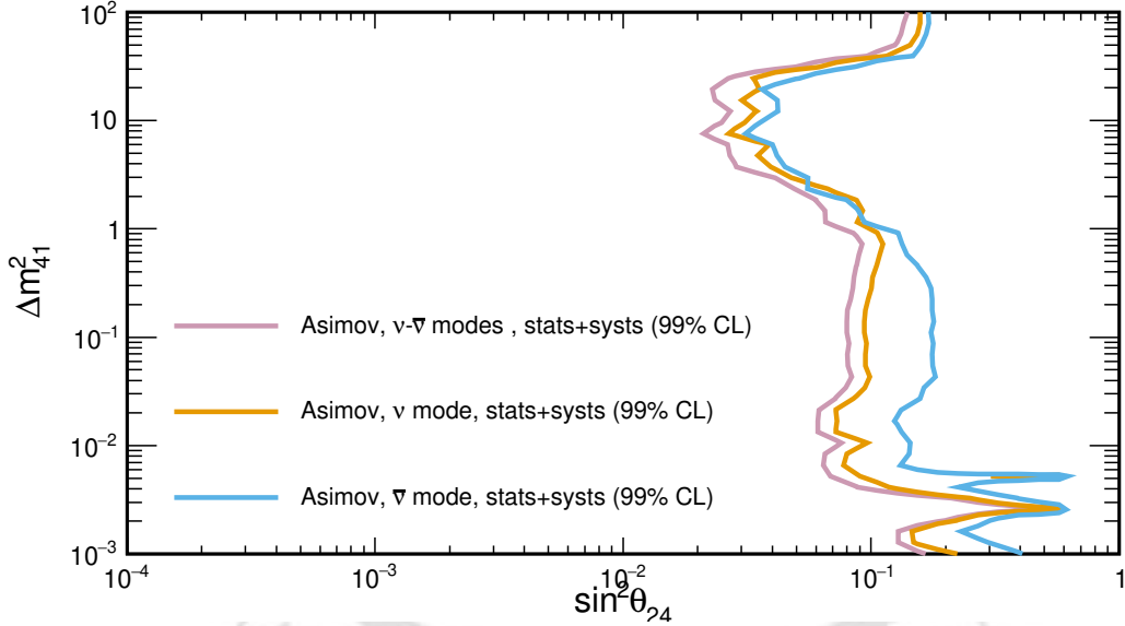
Figure 7.8: Asimov sensitivities for \sin^2 \theta_{24} vs \Delta m^2_{41} at 99% CL. A comparison of the full sensitivity (pink) with the FHC ( \nu ) (orange) and the RHC ( \bar{\nu} ) (blue) sensitivities.
