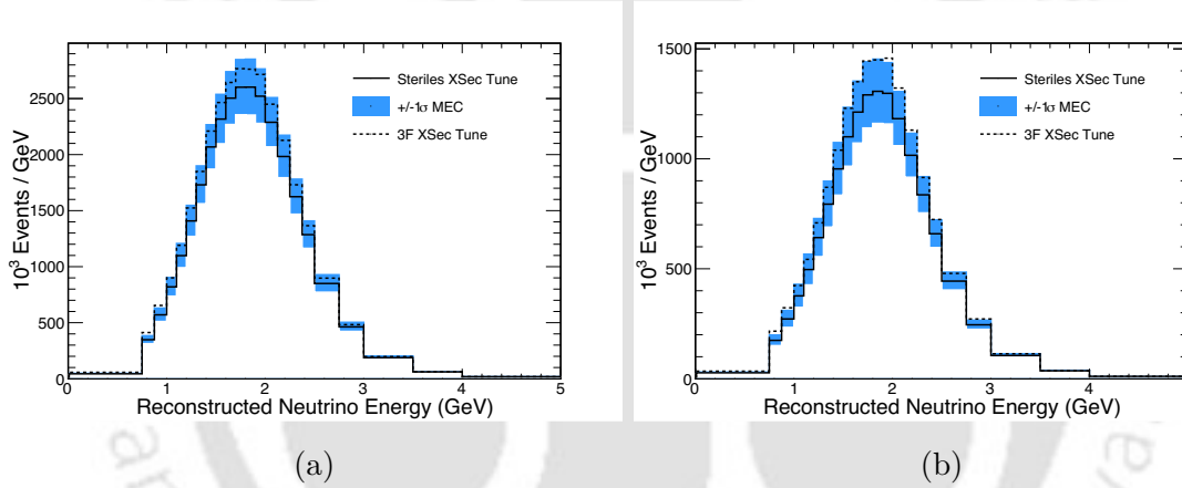
Figure 6.5: This plot shows the 3-flavor cross section tune, including the standard GENIE weights and the 3-flavor MEC weights (dashed), sterile specific XSec tune in solid black, and \pm 1\sigma MEC uncertainty band (in blue). The distribution on the right is RHC, and on the left is for the FHC.
