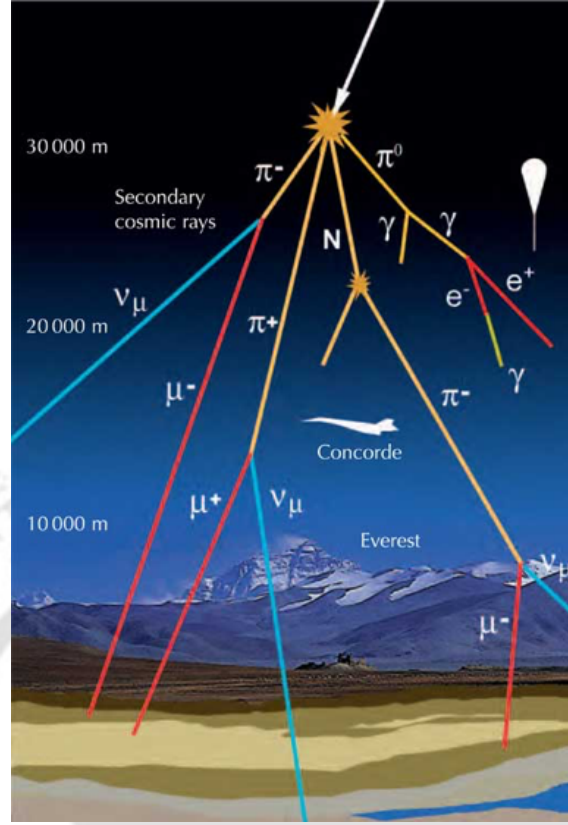
Figure 1.5: Production of atmospheric neutrinos through cosmic-ray interactions in the Earth's atmosphere.
