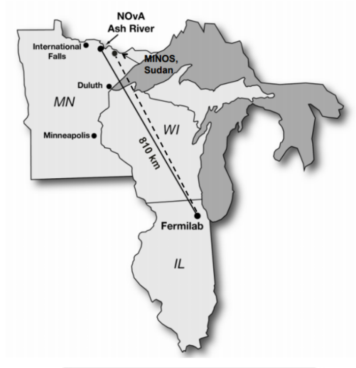
Figure 3.1: Schematic representation of the NOvA's baseline. The neutrino source and the near detector (ND) are based at Fermilab, Illinois, while the far detector (FD) is placed 810 Km away at Ash River, Minnesota.
