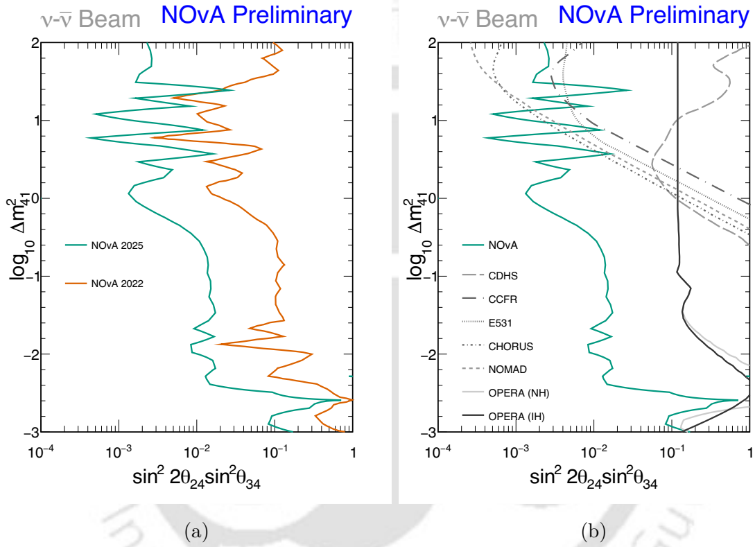
Figure 7.14: NOvA's 90% confidence limits in \sin^2 2\theta_{24} \sin^2 \theta_{34} vs \Delta m^2_{41} space in green on the left compared with the previous analysis and with allowed regions and exclusion contours from other experiments on the right [91, 99, 100, 101, 102]. Regions to the right of the contours are excluded.
