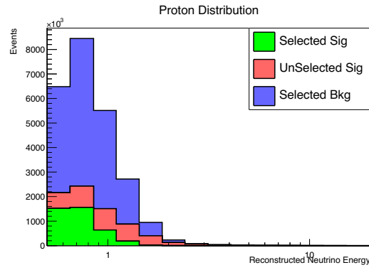
Figure A.1: Signal and Bkg Distribution for single proton sample of this sample Tab. A.1 .
