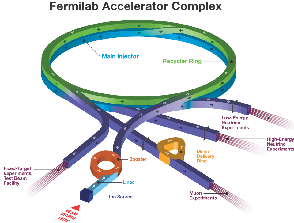
Figure 3.2: Schematic diagram of the Fermilab Accelerator Complex. The beam is followed to the Linac, Booster and main injector from the ion source. The neutrino beam is transferred to various experiments.
