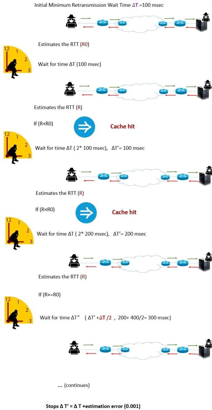
Figure 4.4: Demonstration of estimation of \Delta T
