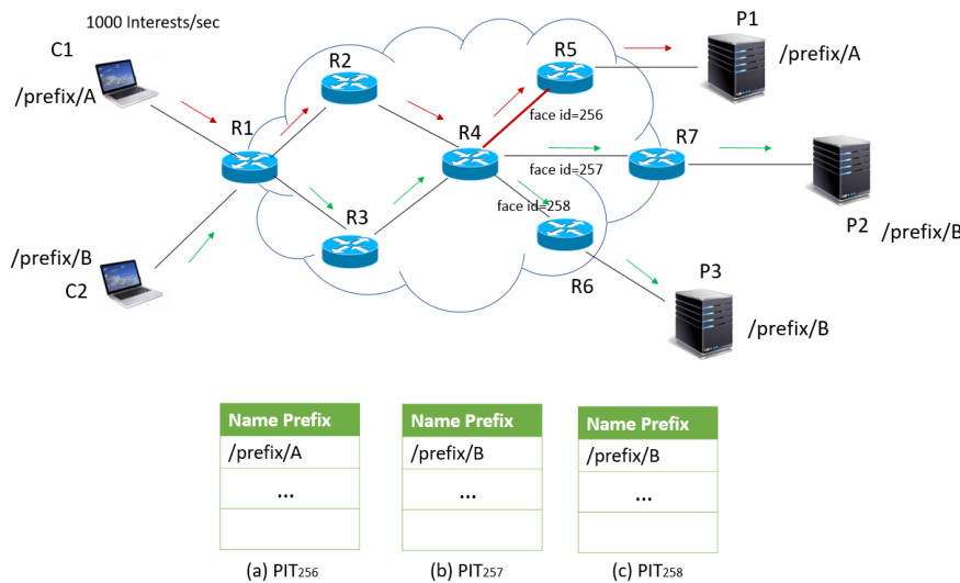
Figure 5.2: Distributed PIT (PIT per outgoing interface)
