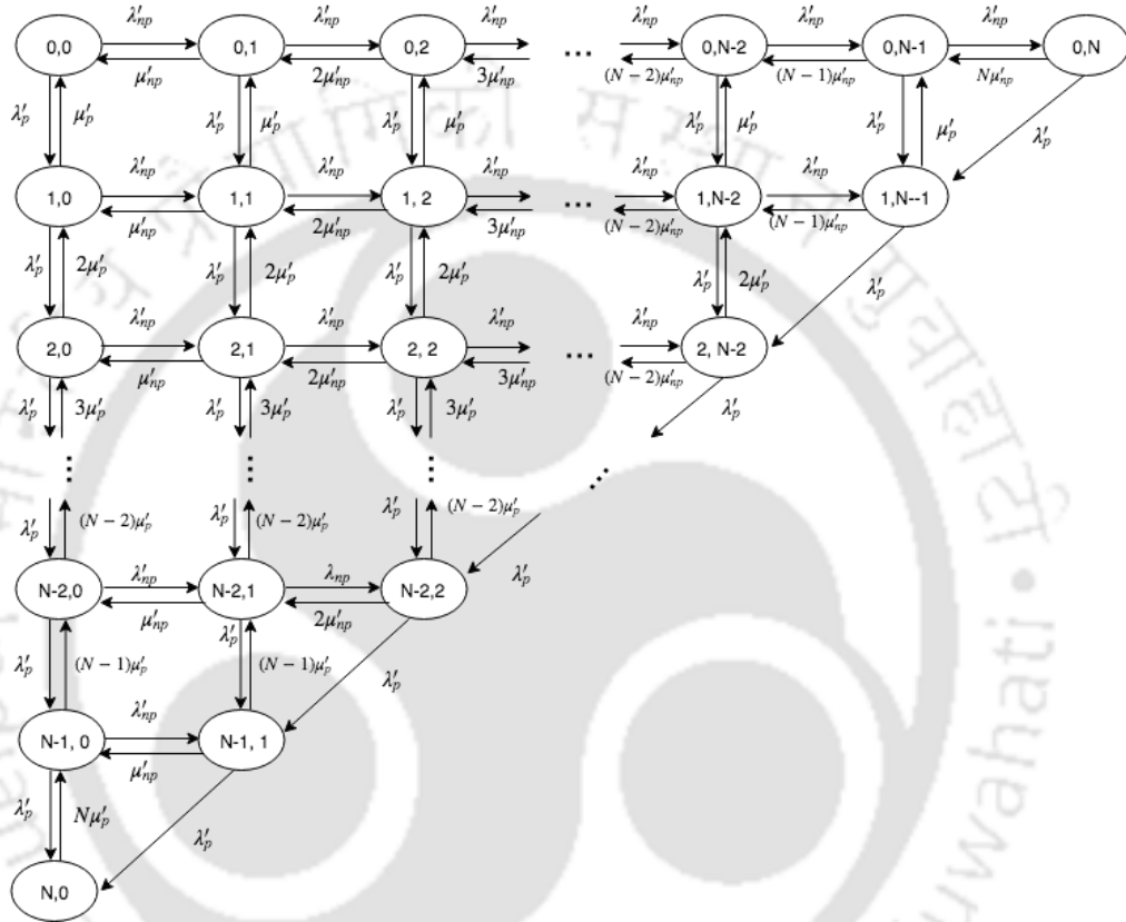
Figure 3.3: Transition rate diagram for PRWR scheme
