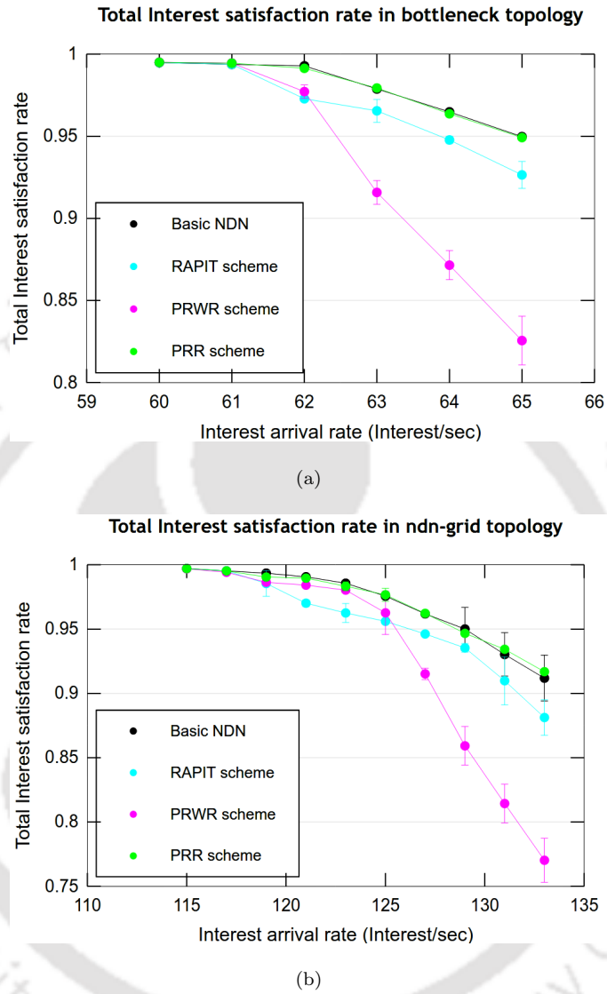
Figure 3.14: Total Interest satisfaction rate vs Interest arrival rate (a) bottleneck topology (b) ndn-grid topology. The error bars in the plot indicate 95% confidence intervals.
