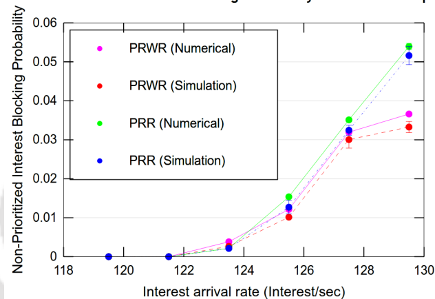
Non-Prioritized Interest Blocking Probability in bottleneck topology
