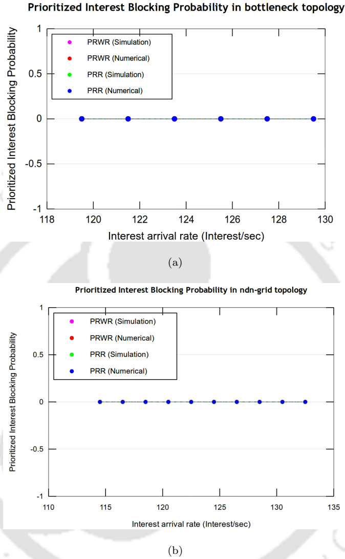
Figure 3.17: Prioritized Interest Blocking probabilities (a) bottleneck topology (b) ndn-grid topology. The error bars in the plot indicate 95% confidence intervals. The simulation results are same both for 30% and 40% prioritized Interests.
