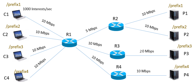
Figure 5.5: Topology
