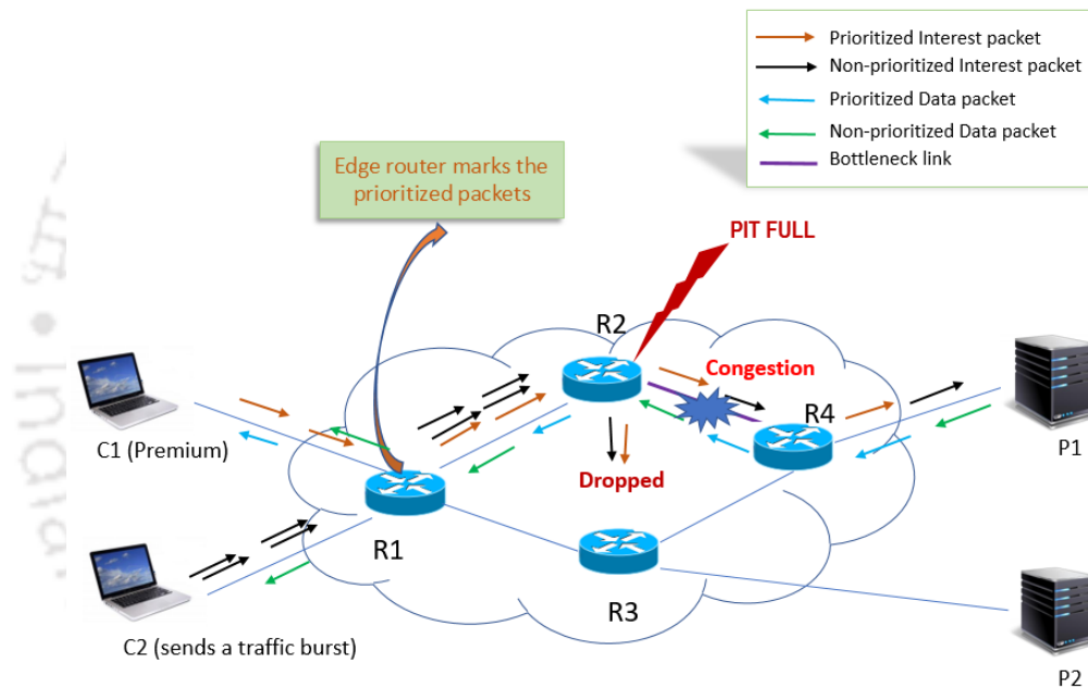
Figure 3.1: System model of EQPR
