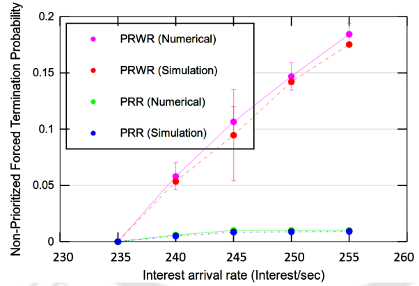
Non-Prioritized Interest Forced Termination Probability in rocketfuel topology
