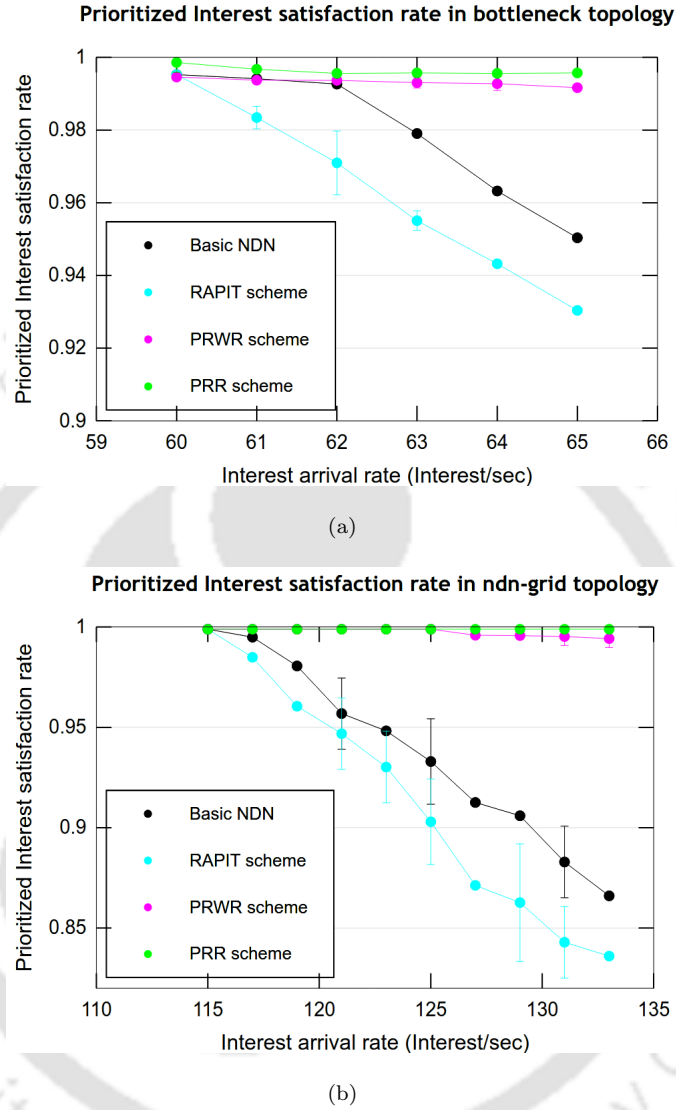
Figure 3.12: Prioritized Interest satisfaction rate vs Interest arrival rate (a) bottleneck topology (b) ndn-grid topology. The error bars in the plot indicate 95% confidence intervals.
