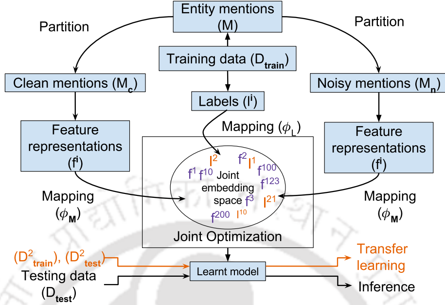
Figure 3.3: The overview of the proposed Fine-ET system.
