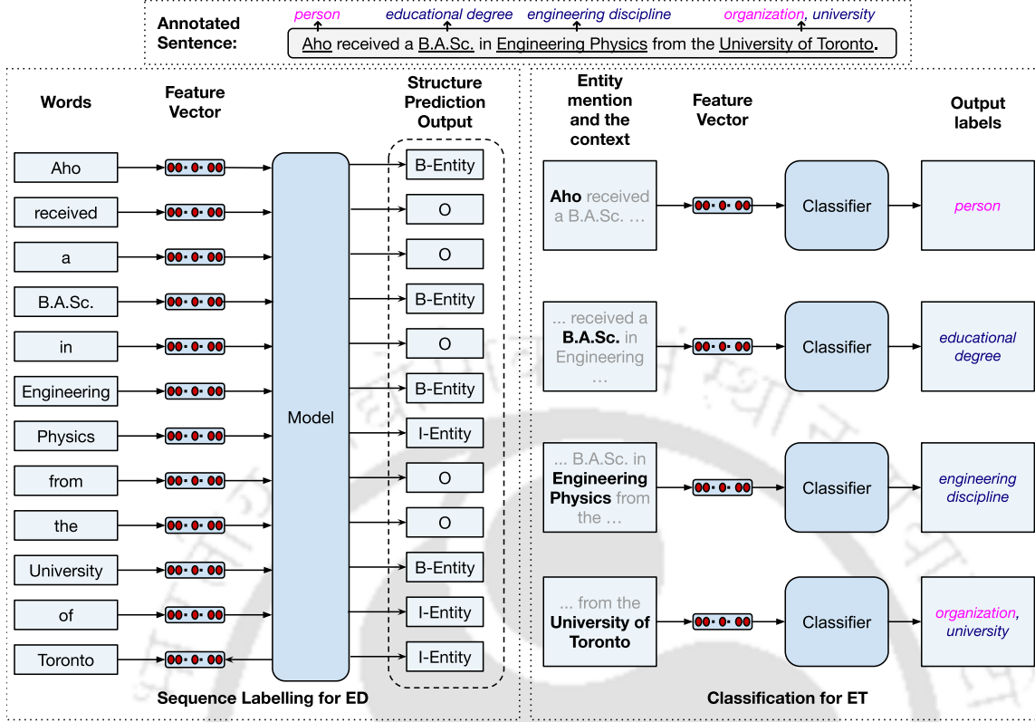
Figure 2.4: In the case of overlapping labels, the ED and ET tasks are modeled independently, as illustrated. For the ED task, a sequence labelling approach is used where the annotated sentence’s multi-label annotations are converted into a binary (entity, non-entity) annotations. For the ET task, a classifier is used to assign labels to the entity mentions present in the sentence independently.
