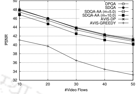
Figure 5.6: \overline{PSNR} Vs. \#Video \text{ Flows}
