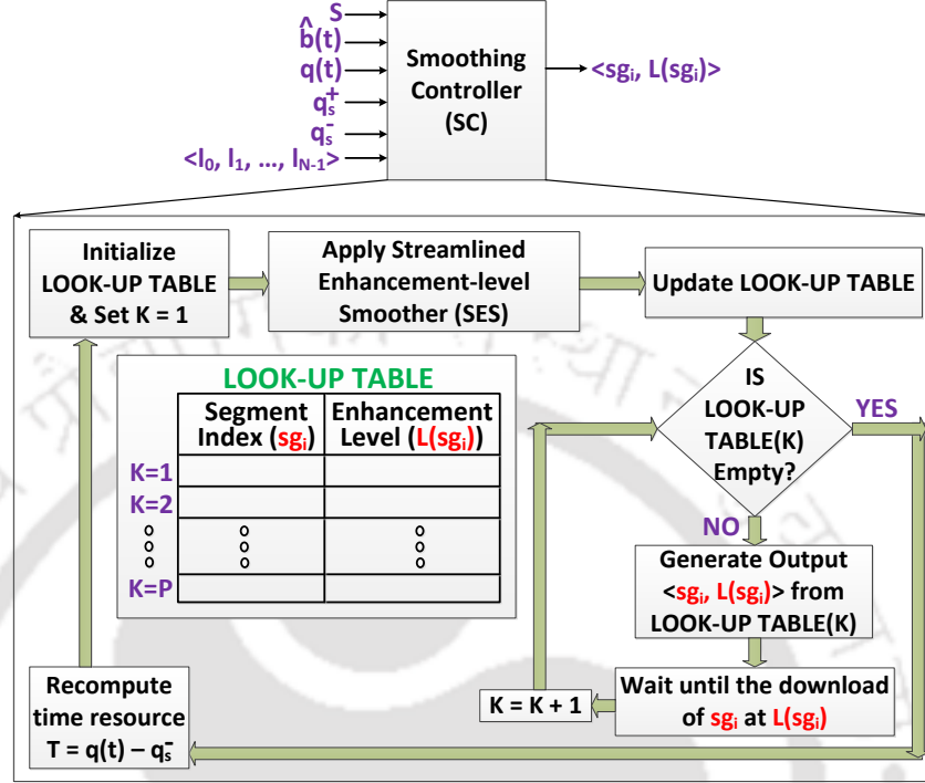
Figure 6.7: Smoothing Controller.
