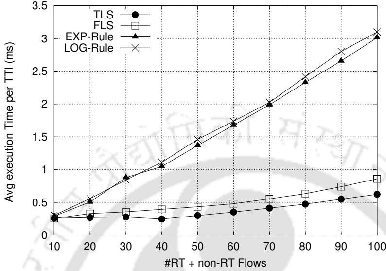
Figure 3.15: Comparative results for average execution time (in milliseconds)
