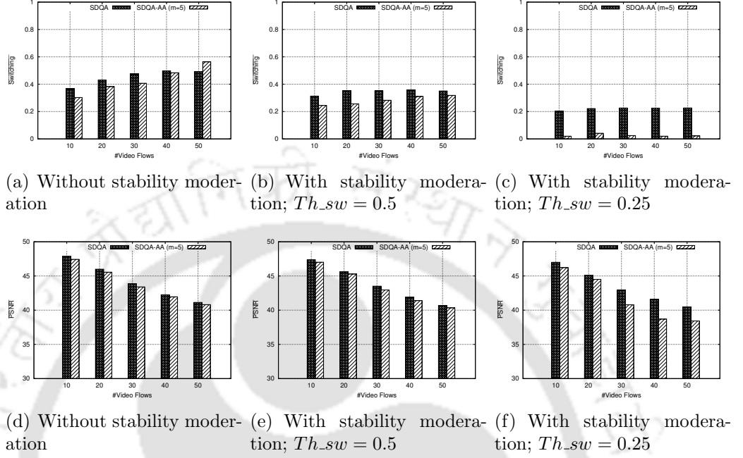
Figure 5.10: Results for \overline{Switching} and \overline{PSNR} without stability moderation and with stability moderation (at Th_{sw} = 0.5, 0.25 )
