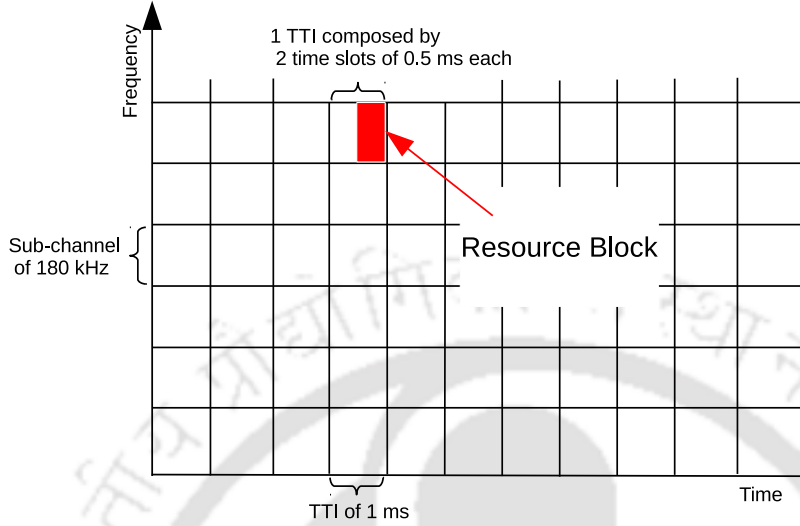
Figure 2.2: Combined time-frequency multiplexed resource abstraction in LTE
