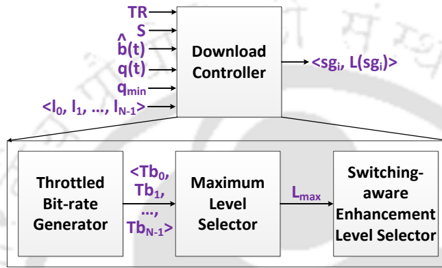
Figure 6.4: Download Controller (DC).
