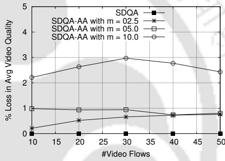
Figure 5.8: % loss in video Quality Vs. #Video Flows
