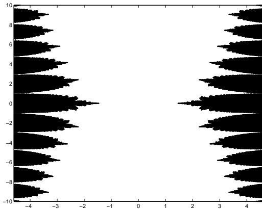
Figure 3.5: Julia set of 0.75 \frac{\sinh^2 z}{z^2}
