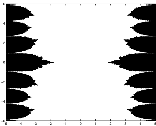
Figure 3.7: Julia set of 0.15(I_0(z) + 1)(I_0(z) + 2)
