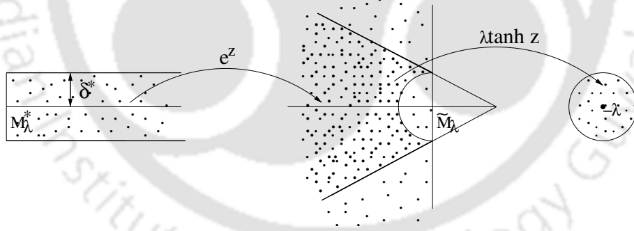
Figure 2.4: Mapping property of \lambda \tanh(e^z) .
