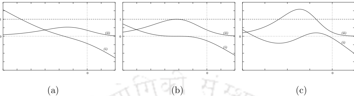
Figure 2.2: Graphs of (i) f_\lambda^2(x) - x and (ii) (f_\lambda^2)'(x) for (a) \lambda > \lambda^* , (b) \lambda = \lambda^* and (c) \lambda < \lambda^* .
