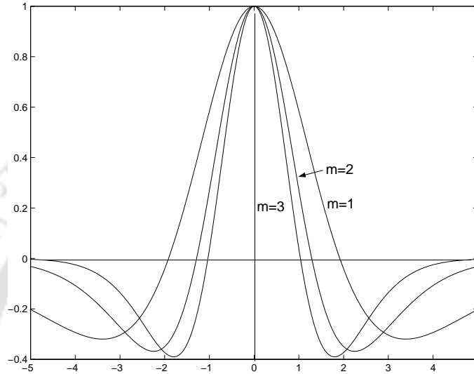
Figure 5.1: Graph of \phi(x) for m = 1 , m = 2 and m = 3 .
