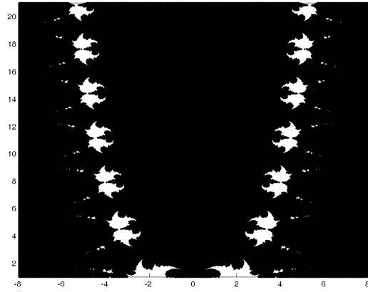
Figure 3.2: Julia set of 2.5291 \frac{I_1(z)}{z}
