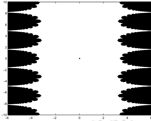
Figure 3.3: Julia set of I_2(z)
