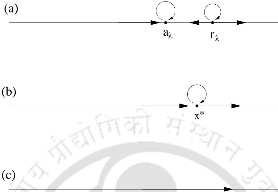
Figure 4.2: Phase portraits of f_\lambda(x) = \lambda J(e^x + 1) for (a) 0 < \lambda < \lambda^* , (b) \lambda = \lambda^* and (c) \lambda > \lambda^* .
