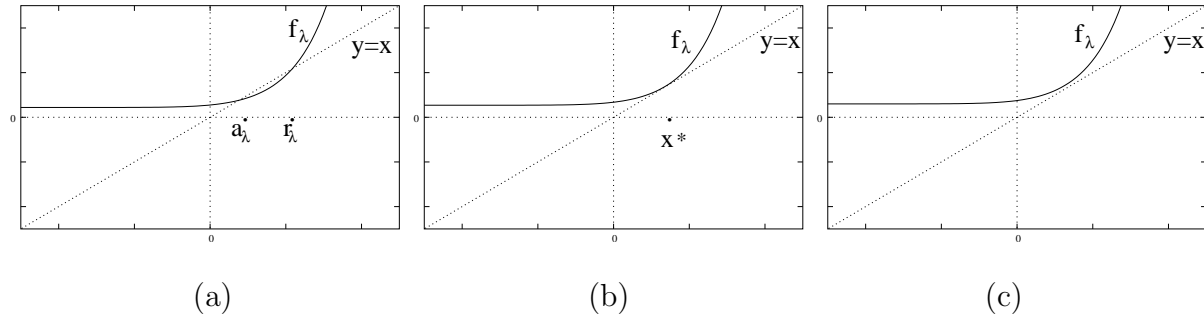
Figure 4.1: Graphs of f_\lambda(x) = \lambda J(e^x + 1) for (a) \lambda < \lambda^* (b) \lambda = \lambda^* and (c) \lambda > \lambda^* .
