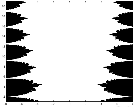
Figure 3.1: Julia set of 2.5 \frac{I_1(z)}{z}
