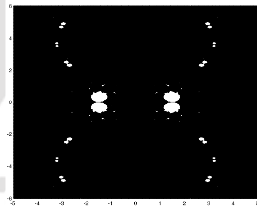
Figure 3.8: Julia set of 0.1556(I_0(z) + 1)(I_0(z) + 2)
