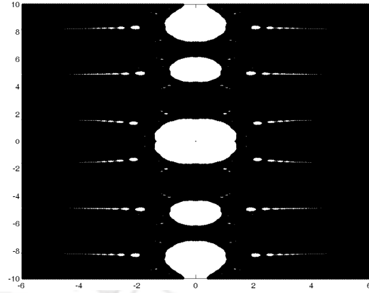
Figure 3.4: Julia set of 5I_2(z)
