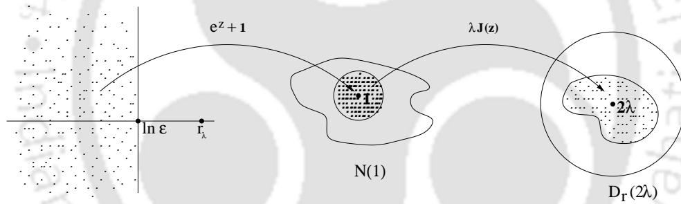
Figure 4.3: Mapping property of f_\lambda(z) = \lambda J(e^z + 1) for 0 < \lambda < \lambda^* .
