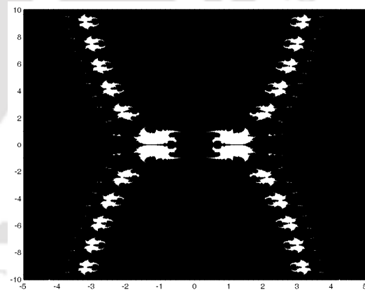
Figure 3.6: Julia set of 0.7619 \frac{\sinh^2 z}{z^2}
