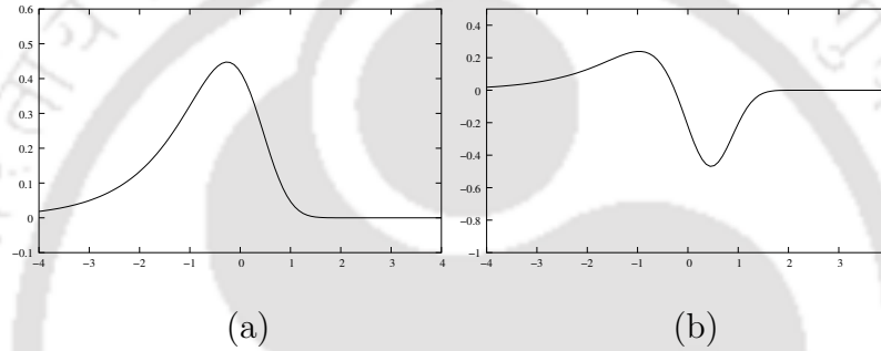
Figure 2.1: Graphs of (a) f'(x) and (b) f''(x) .
