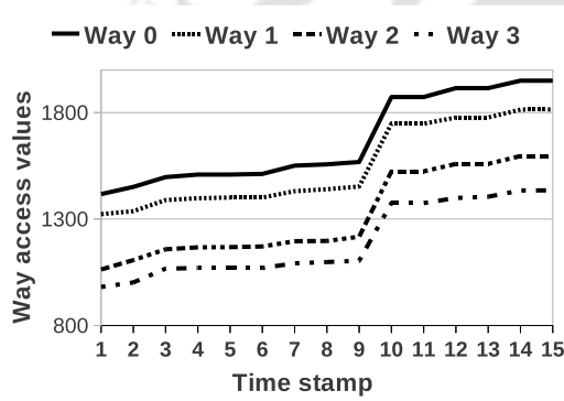
FIGURE 5.2: Way Access pattern in a bank for benchmark: Body16.
