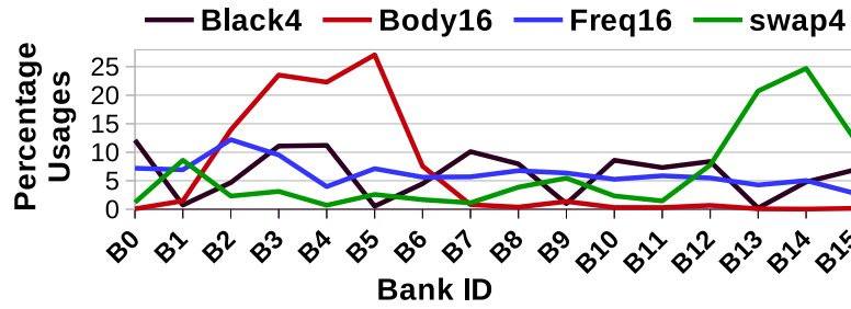
FIGURE 4.2: Variable bank usages across different benchmarks
