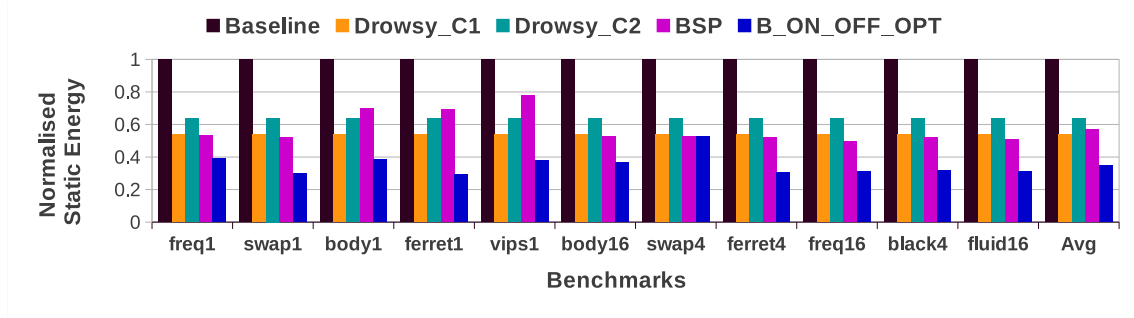
FIGURE 4.13: Normalised static energy consumption for B_ON-OFF-OPT and compared with BSP and Drowsy, with 4MB L2 cache.
