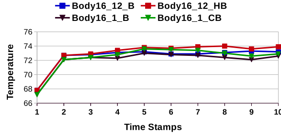
FIGURE 6.5: Thermal status of target banks in HB and CB, for Body16.
