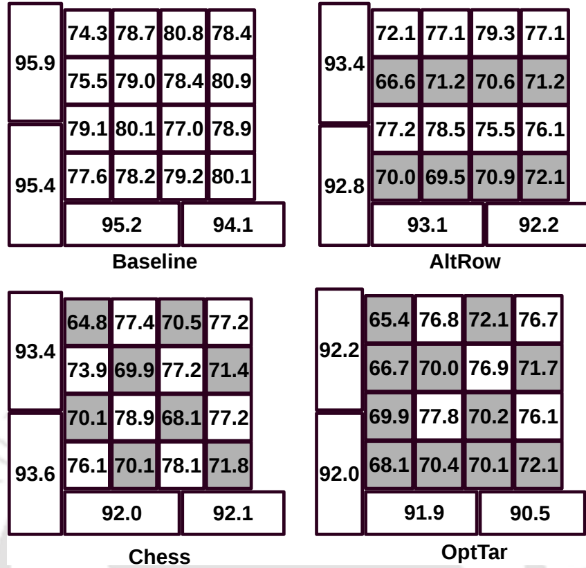
FIGURE 7.17: Temperatures (in °C) of the individual banks during \mathbf{r} , for Fluid16.
