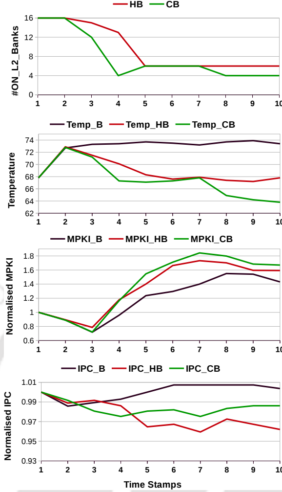
FIGURE 6.4: Temporal effect of cache resizing: body16.
