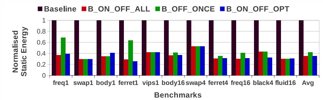
FIGURE 4.17: Normalised static energy value for different benchmark applications IPC degradation threshold = 4, with 4MB L2 cache.
