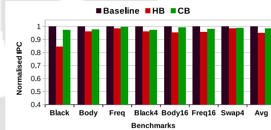
FIGURE 6.9: Change in IPC with respect to baseline.
