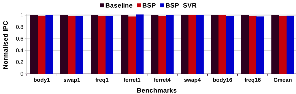
FIGURE 5.7: Change in IPC: BSP vs BSP_SVR.
