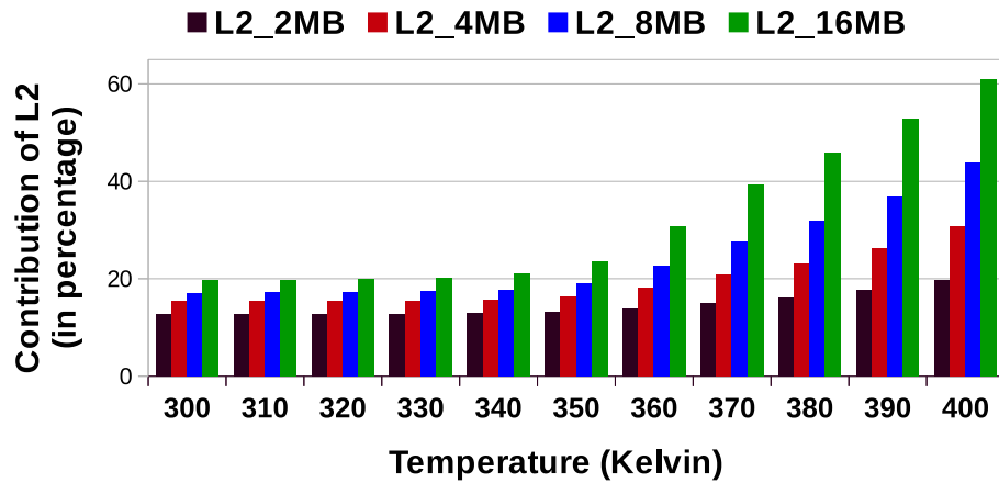
FIGURE 2.7: Contribution of LLCs to the total Chip power consumption.
