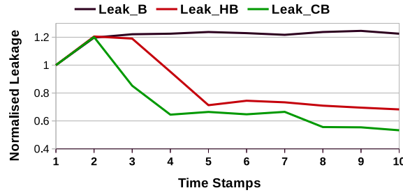
FIGURE 6.6: Change in cache leakage in HB and CB, for Body16.
