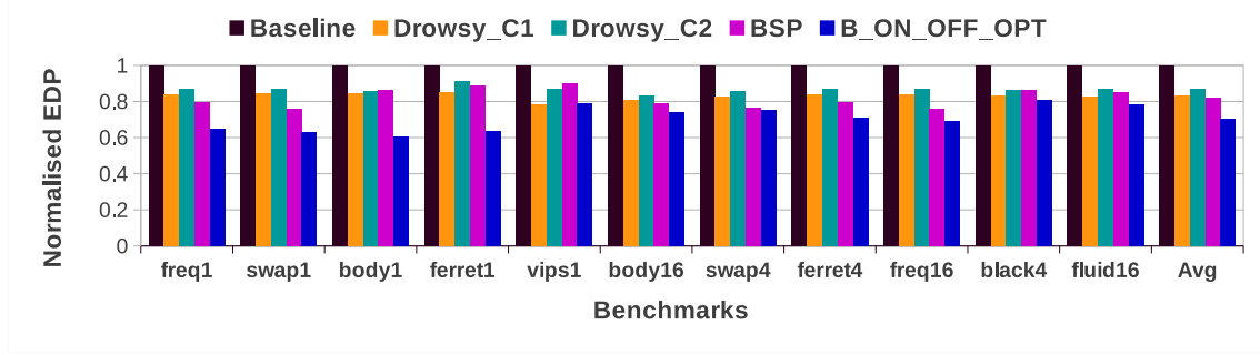
FIGURE 4.12: Energy Delay Product obtained in B_ON-OFF-OPT over BSP and Drowsy, with 4MB L2 cache. A smaller value is better.
