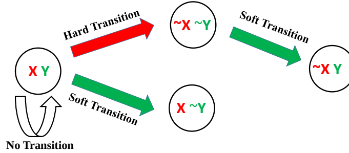
Figure 2.5: Hard and Soft-bit states during different transitions of a MLC STT-RAM cell
