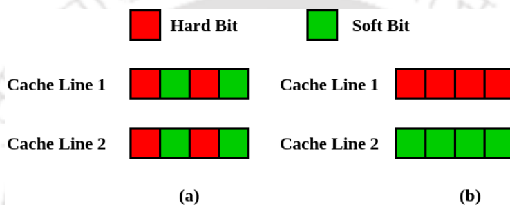
Figure 2.6: 4 bit cache lines in (a) Direct Mapping (b) Cell Split Mapping
