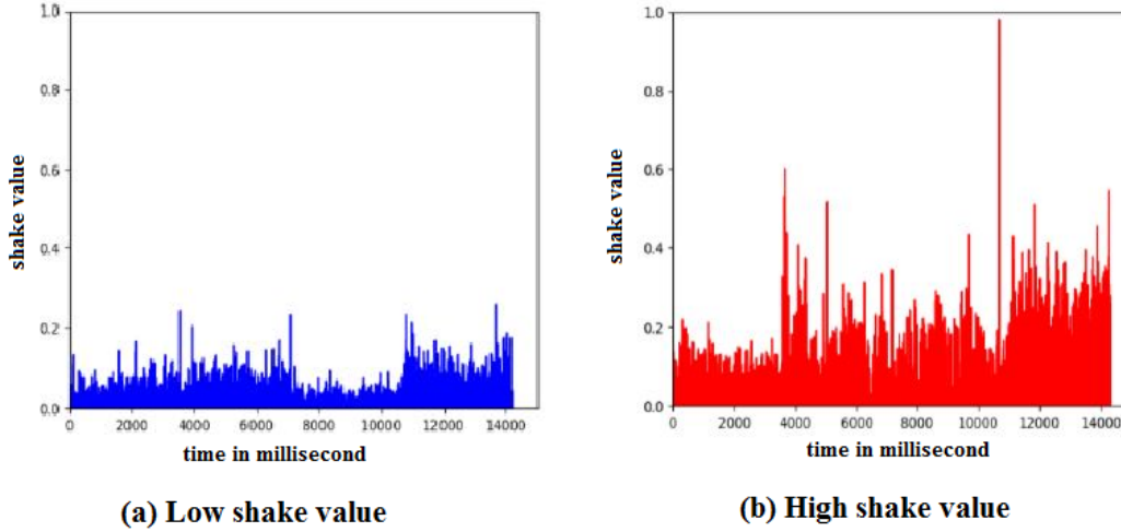
Figure 6.5: Low and high shake value
