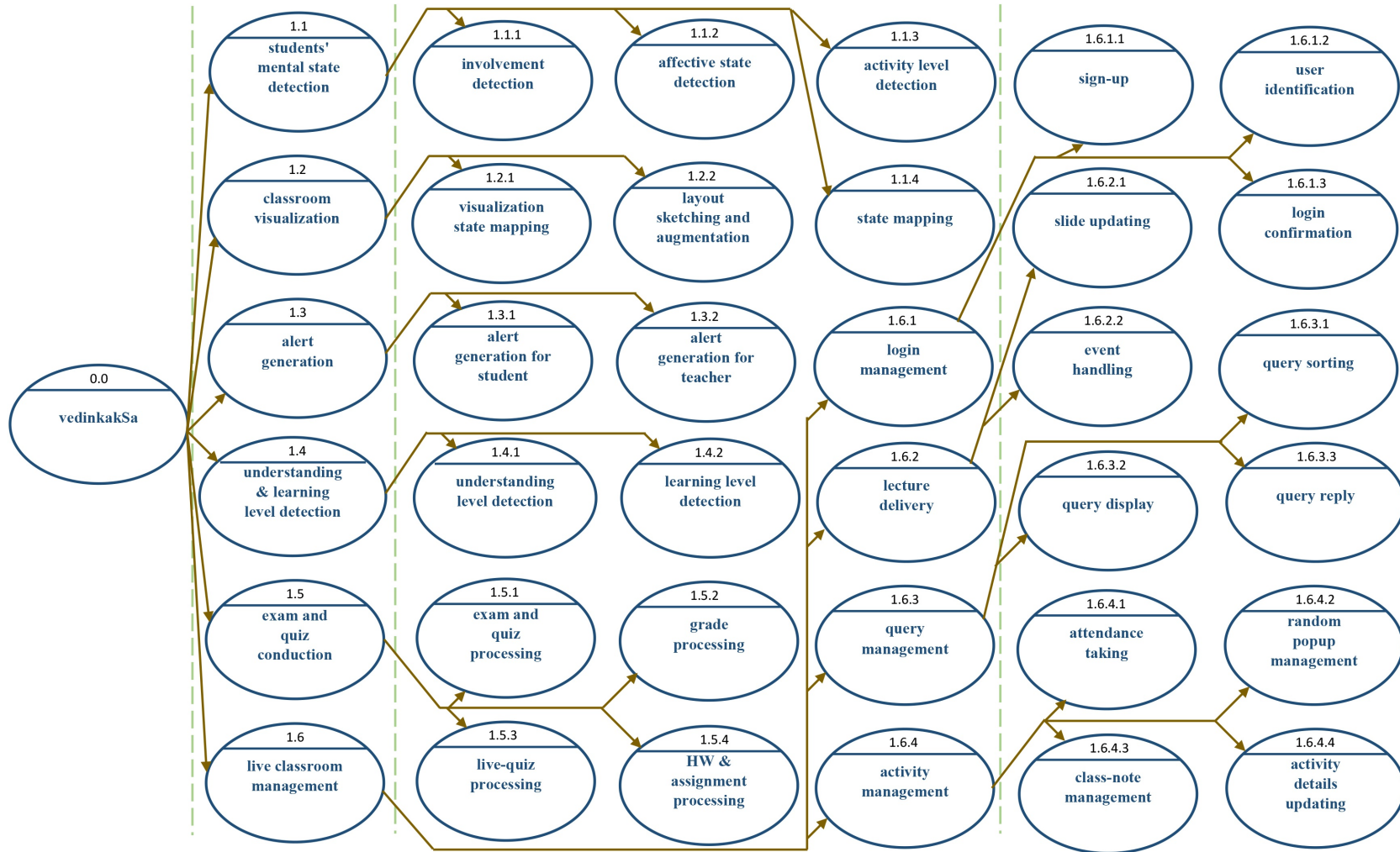
Figure B.13: Process decomposition of the sensitive blended learning system design
