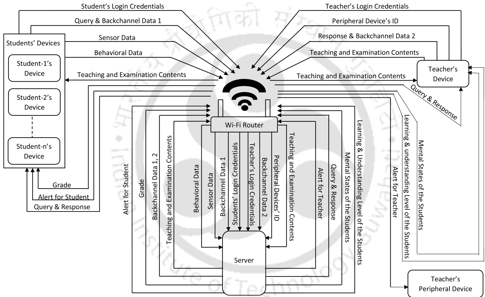
Figure 3.7: System architecture of a sensitive classroom which follows the Vedinkaksha framework
