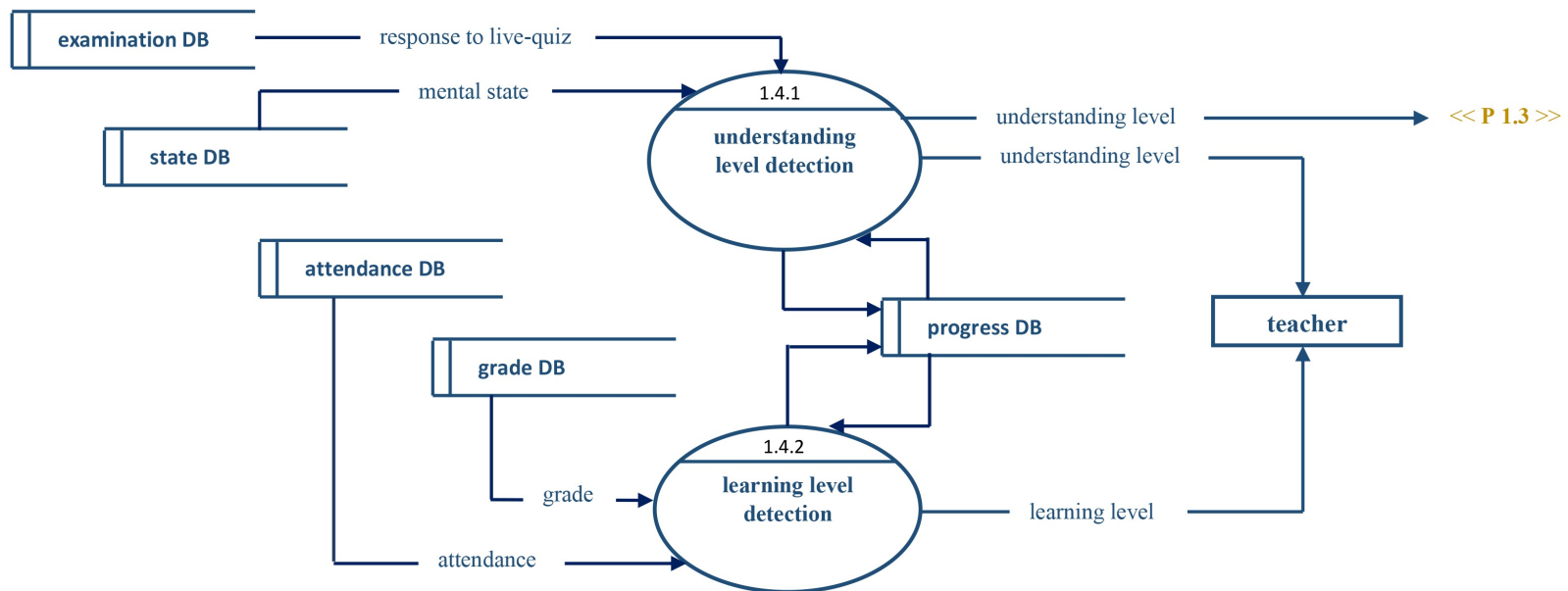
Figure B.6: Level-2 (of Process 1.4) DFD of the sensitive blended learning platform
