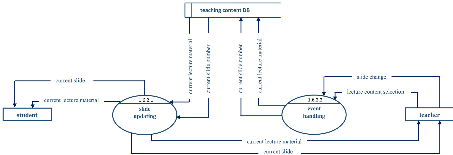
Figure B.10: Level-3 (of Process 1.6.2) DFD of the sensitive blended learning platform
