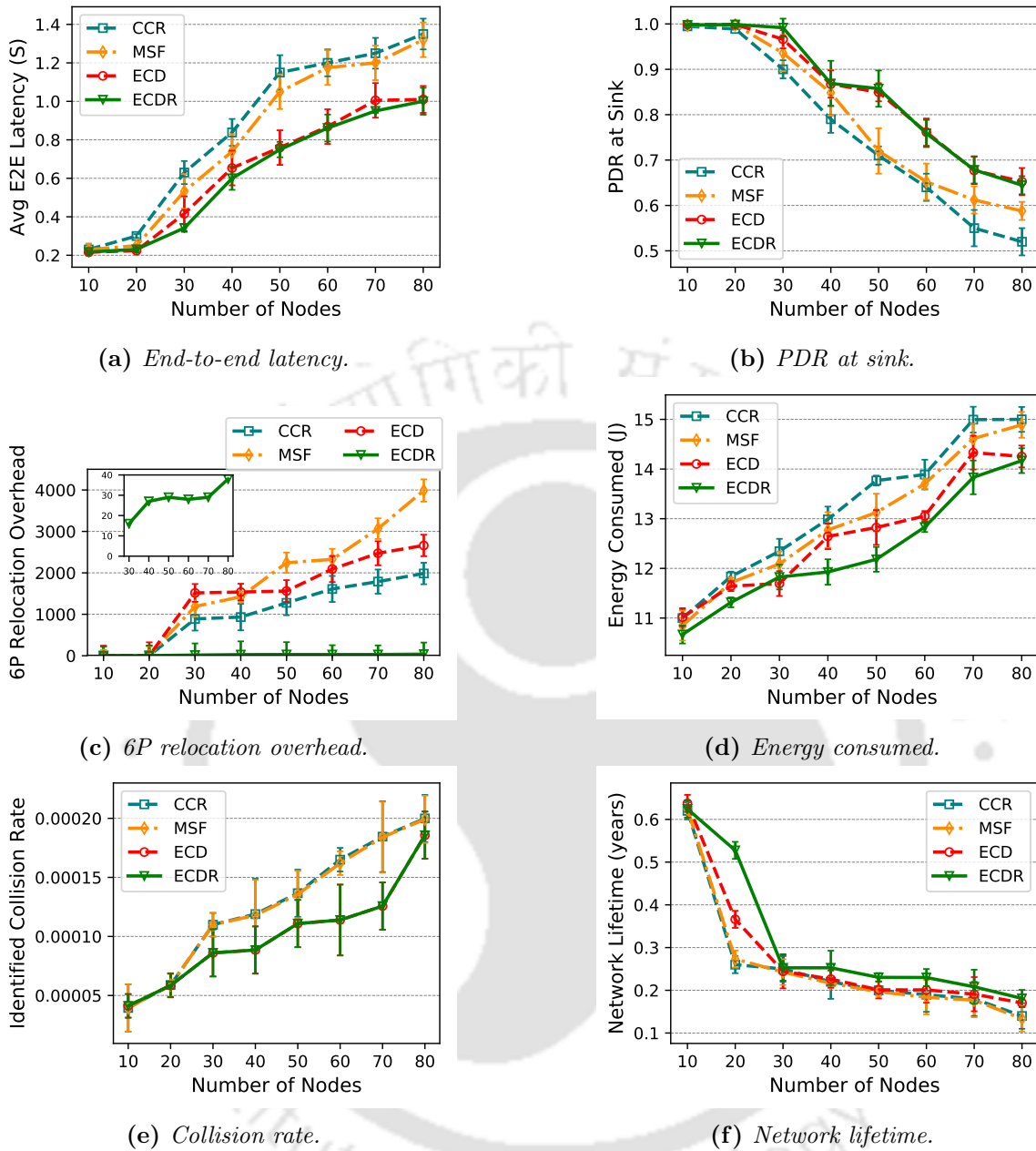
Figure 4.3: Comparison of results under varying network sizes with traffic rate 2P/SF
