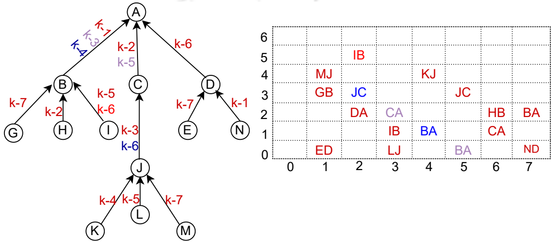
Figure 3.2: An example of a network topology and its corresponding schedule designed by RTDS considering 7 channels and a slotframe with 8 slots, i.e. N_c = 7 , k = 8 . The values shown with the links are selected SlotOffset only.
