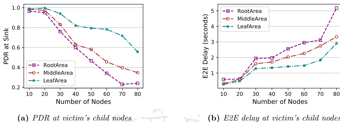
Figure 5.9: Impact of victim's position on PDR and E2E latency at victim's child nodes
