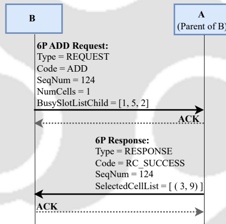
Figure 3.3: Modified 6P with 2P ADD transaction
