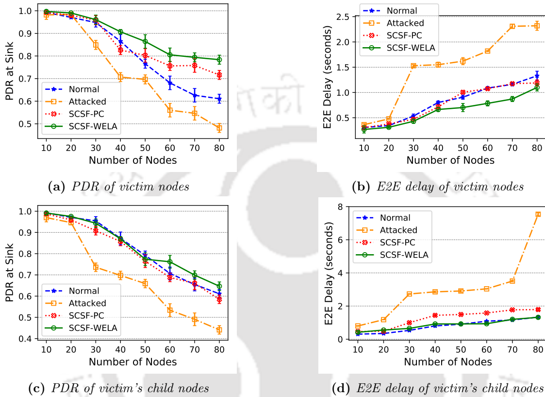
Figure 5.3: PDR and E2E delay of victim and victim’s child nodes under the attack
