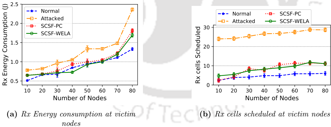
Figure 5.4: Rx energy consumption at victim nodes under varying network sizes
