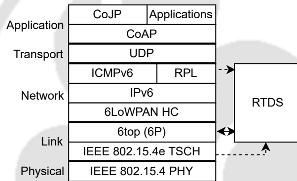
Figure 3.1: The 6TiSCH protocol stack with RTDS.
