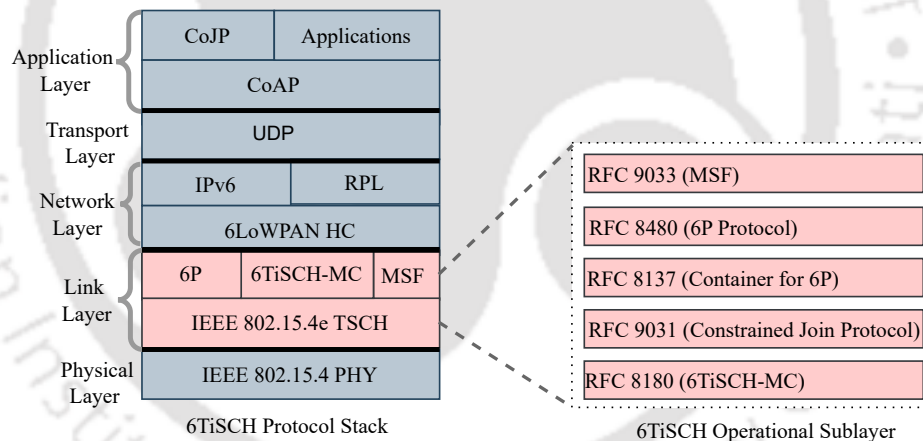
Figure 2.1: The 6TiSCH network protocols stack
