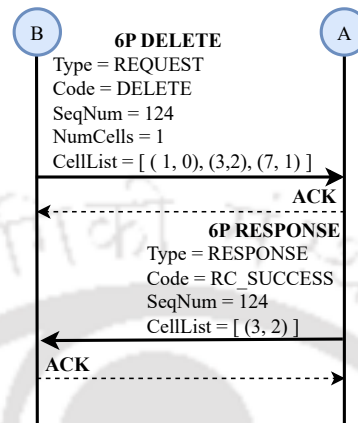
Figure 2.5: An illustration of a cell deletion using 6P protocol, where node B requests node A to delete a cell providing the list of scheduled cells. Node A responds by randomly selecting a cell for deletion
