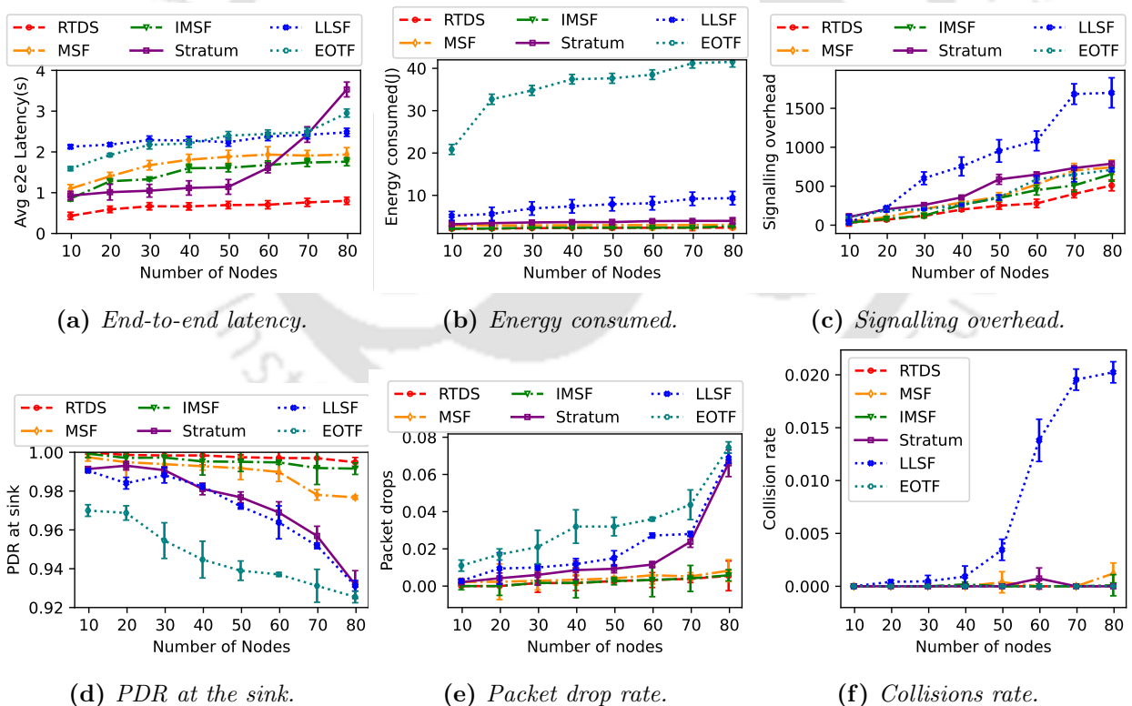
Figure 3.6: Comparison of results under varying network sizes with low traffic rate (e.g.: 1P/20SF)
