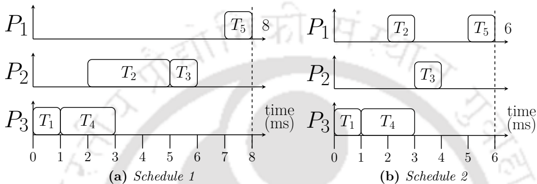
Figure 2.10: Gantt chart: PTG (Figure 2.7) with tasks (Table 2.5) and message (Table 2.3) nodes; Heterogeneous processors; Fully-connected
