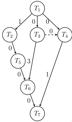
Figure 5.3: Assignment PTG G' obtained from PTG G and the PEFT schedule Table 5.2: PEFT schedule of the PTG in Figure 5.2
