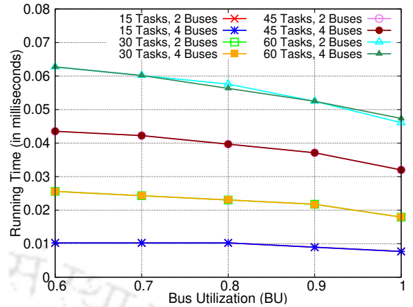
Figure 3.7: ALOLA: Bus Utilization (BU) Vs. Running Time
