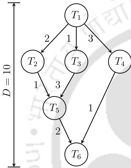
Figure 4.2: Example of a PTG G
