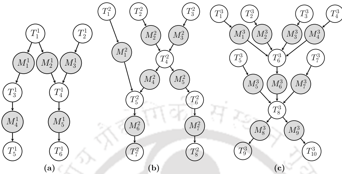
Figure 7.11: PTG representation: (a) Electric Power Steering (EPS), (b) Adaptive Cruise Controller (ACC), (c) Traction Controller (TC)
