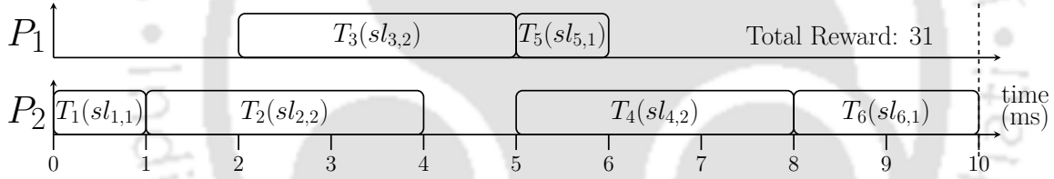
Figure 4.4: ILP-SANC: Schedule for G (in Figure 4.2) depicted as a gantt chart
