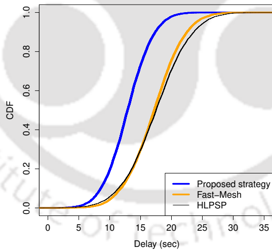
(c) CDF of Startup Delay
