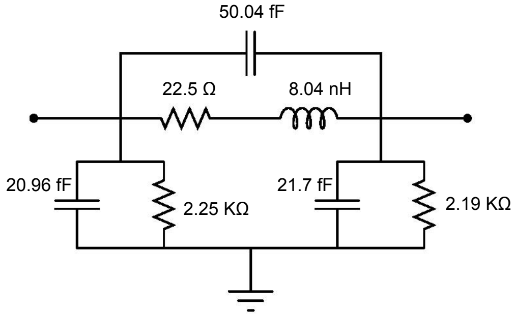
Figure 4.3: Parameters of the \pi model of the tank MPS inductor extracted at 2.4 GHz.
