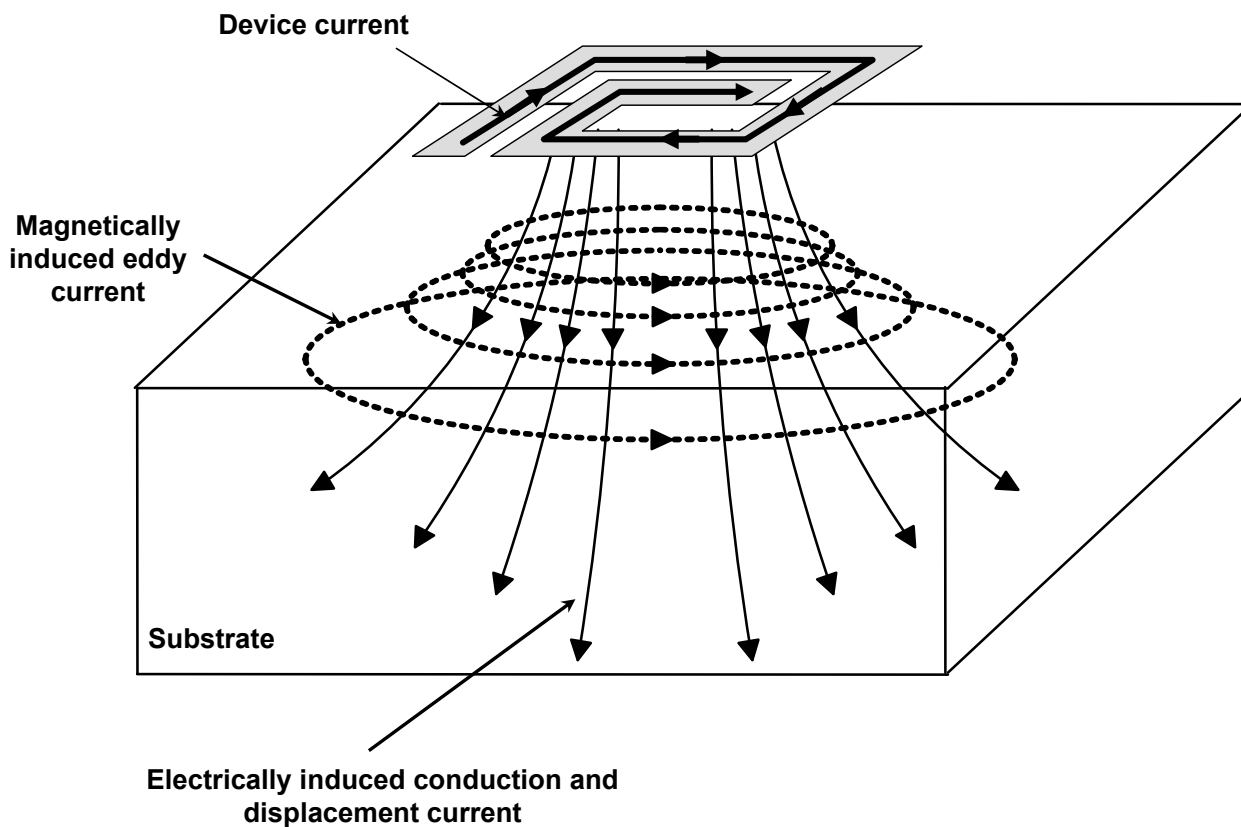
Figure 1.7: Representation of the substrate currents in a spiral inductor. The solid lines represents the electrically induced currents and the dashed lines represent the eddy current [2].
