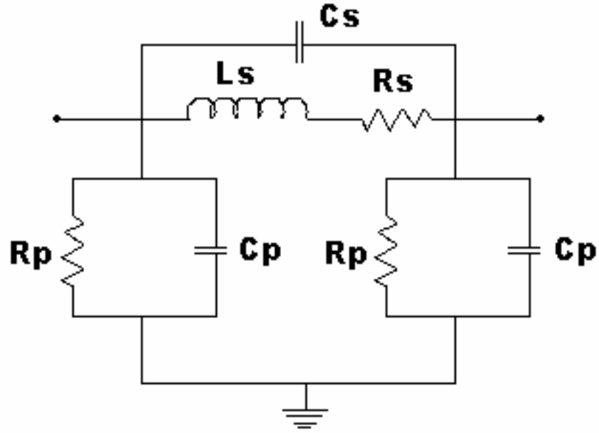
Figure 2.14: Simplified lumped element model of on-chip spiral inductor on silicon.
