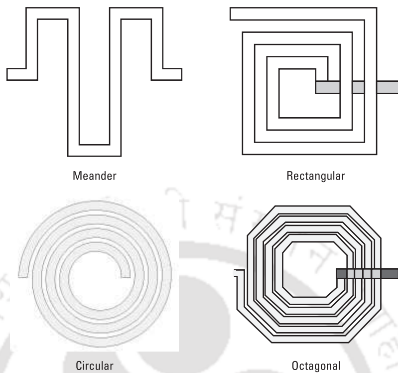
Figure 1.2: Planar inductor structures [1].
