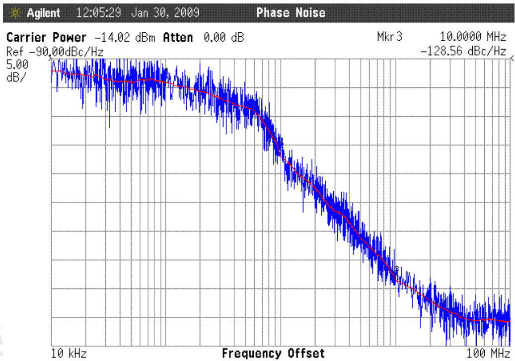
Figure 4.16: Measured phase noise of the VCO.
