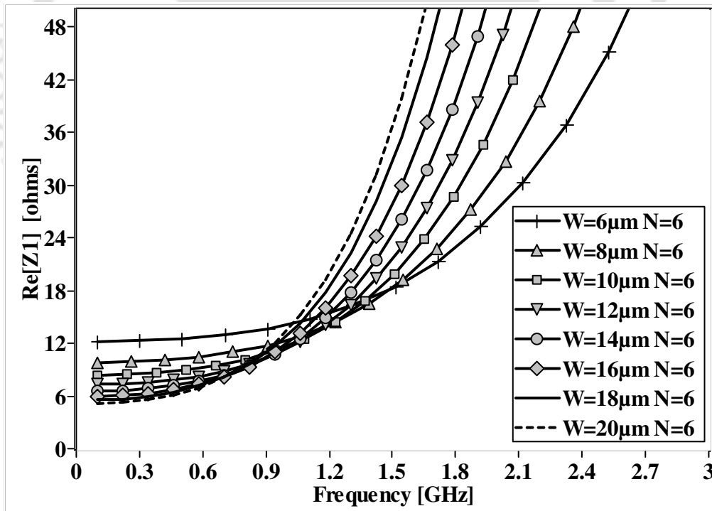
Figure 2.11: Parasitic series resistance for 10 nH inductors designed with different width of 6 \mu\text{m} , 8 \mu\text{m} , 10 \mu\text{m} , 12 \mu\text{m} , 14 \mu\text{m} , 16 \mu\text{m} , 18 \mu\text{m} and 20 \mu\text{m} .
