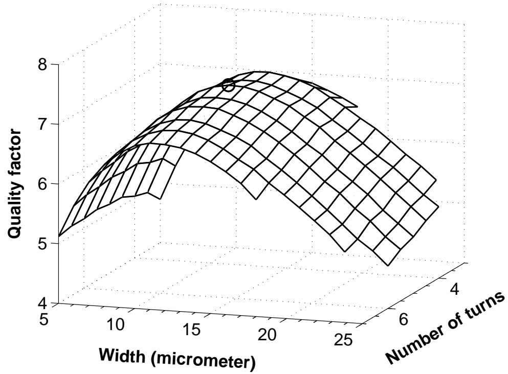
Figure 2.15: Quality factors for 6 nH inductors as a function of width and number of turns.
