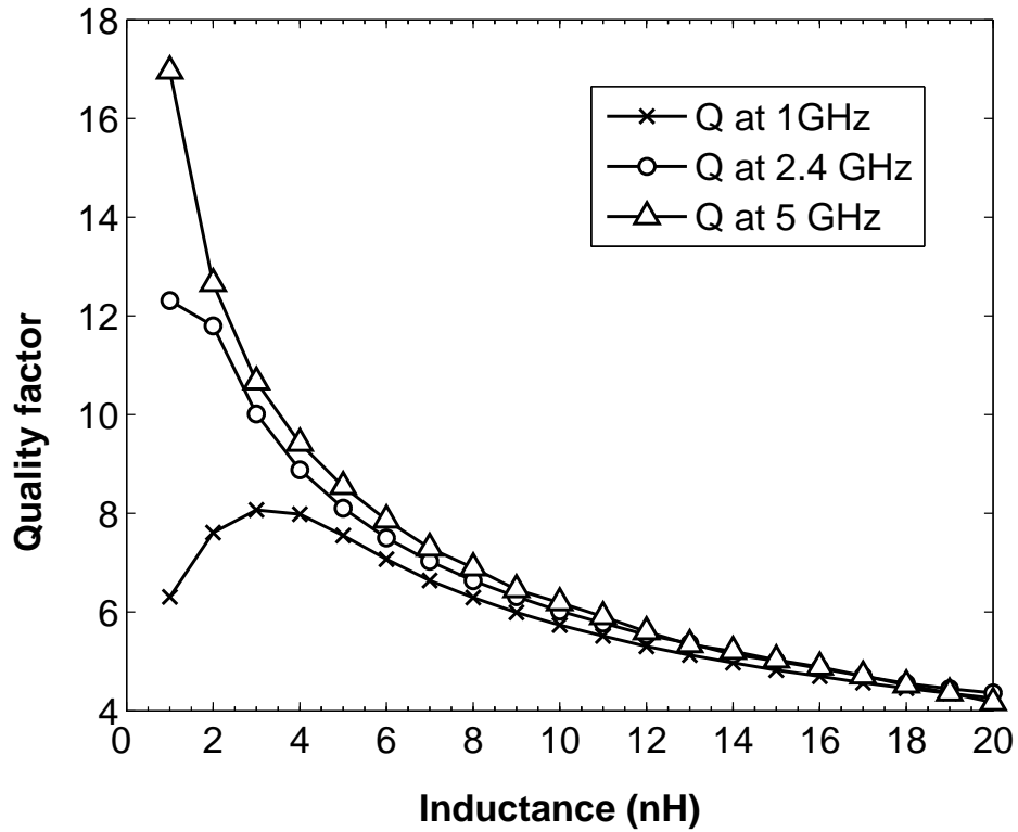
Figure 2.20: Global optimal quality factor and inductance trade off curves at 1 GHz, 2.4 GHz and 5 GHz.
