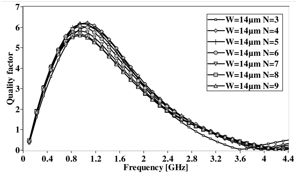
Figure 2.8: Quality factor for 10 nH inductors designed with number of turns 3, 4, 5, 6, 7, 8 and 9 and the width and spacing fixed at 14 μm and 2 μm respectively.
