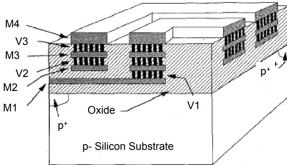
Figure 1.8: Cross sectional view of a spiral inductor showing the shunting of metal layers M2, M3 and M4 in a four metal layer process and the metal underpass in metal layer M1 [3].
