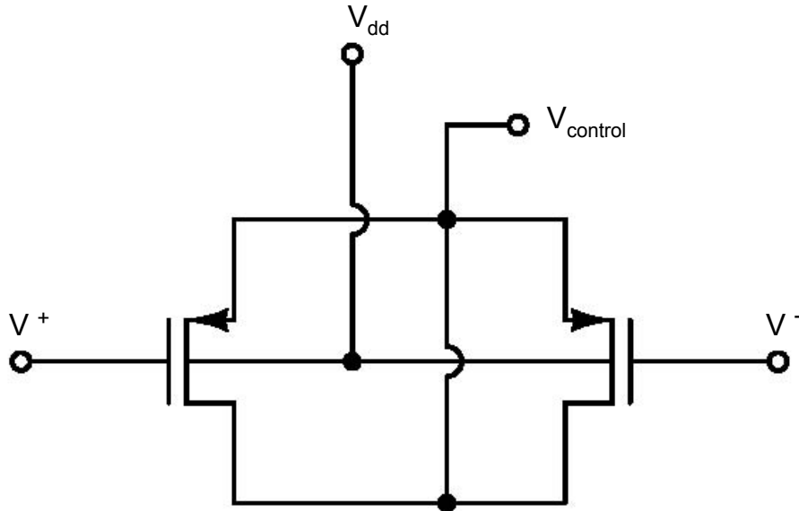
Figure 4.4: Schematic of the PMOS varactor.
