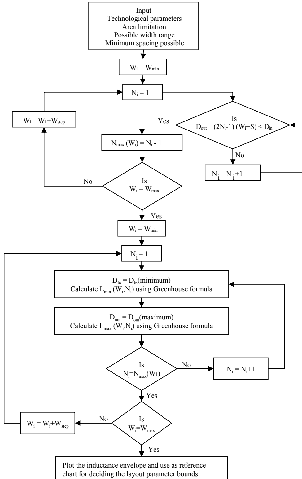
Figure 2.1: Flowchart to determine the layout parameter bounds of spiral inductor.
