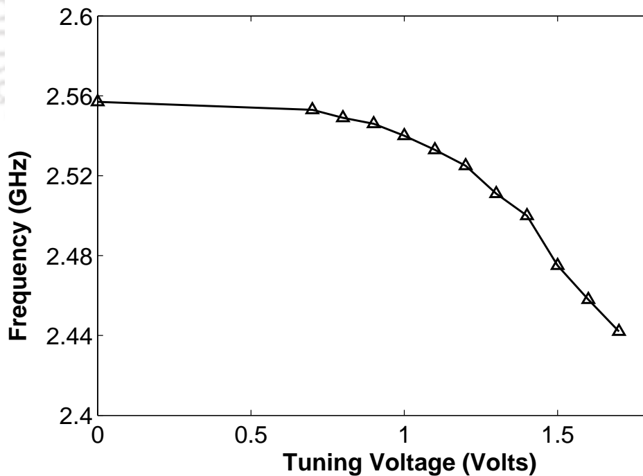
Figure 4.17: Measured tuning characteristics of the VCO.
