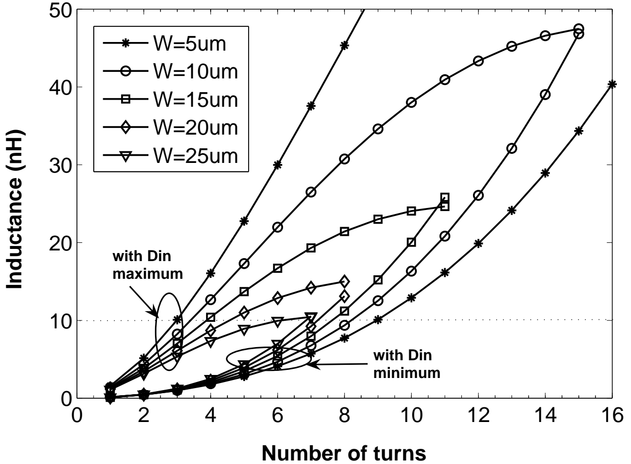
Figure 2.4: Layout parameter bound curves of possible inductances by varying D_{in} from minimum to maximum for all combination of number of turns and width that satisfies the area 400 \mu\text{m} \times 400 \mu\text{m} . Spacing fixed at 2 \mu\text{m} .
