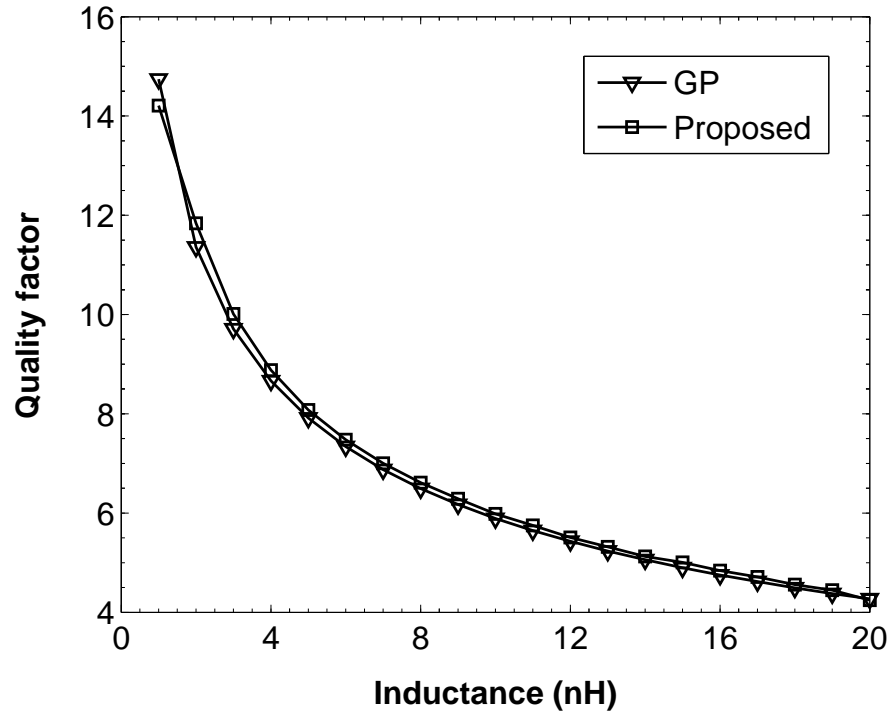
Figure 2.19: Comparison of global optimal trade off curves for inductance range 1 nH - 20 nH at 2.4 GHz (GP - geometric programming).
