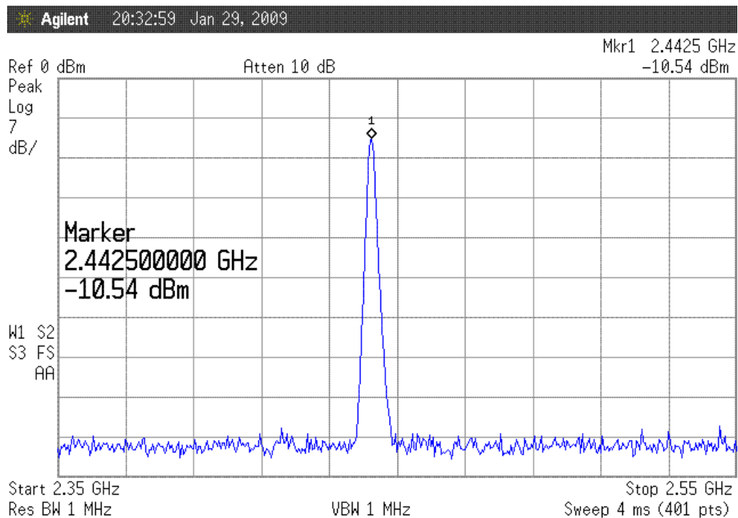
Figure 4.15: Measured output power spectrum of the VCO.
