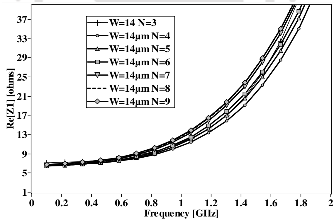
Figure 2.9: Parasitic series resistance for 10 nH inductors designed with number of turns 3,4,5,6,7,8 and 9 and the width and spacing fixed at 14 μm and 2 μm respectively.
