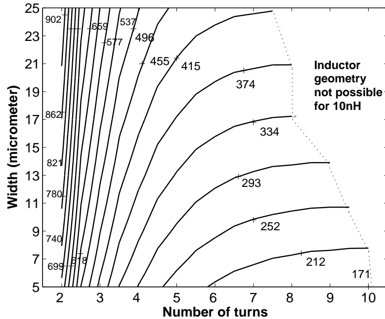
Figure 2.5: Contour plots of outer diameter (with labels in \mu\text{m} ) as a function of width and turns for a 10 nH inductor with spacing 2 \mu\text{m} .
