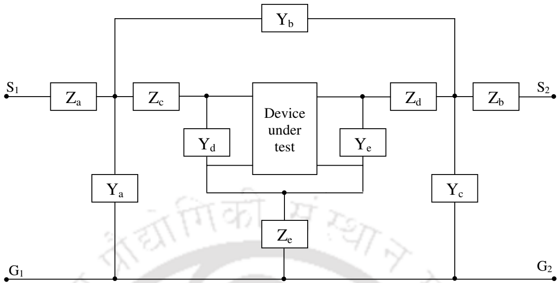
Figure 3.13: An equivalent model of the DUT with the series and parallel parasitics originating from the probe pads and metal interconnect.
