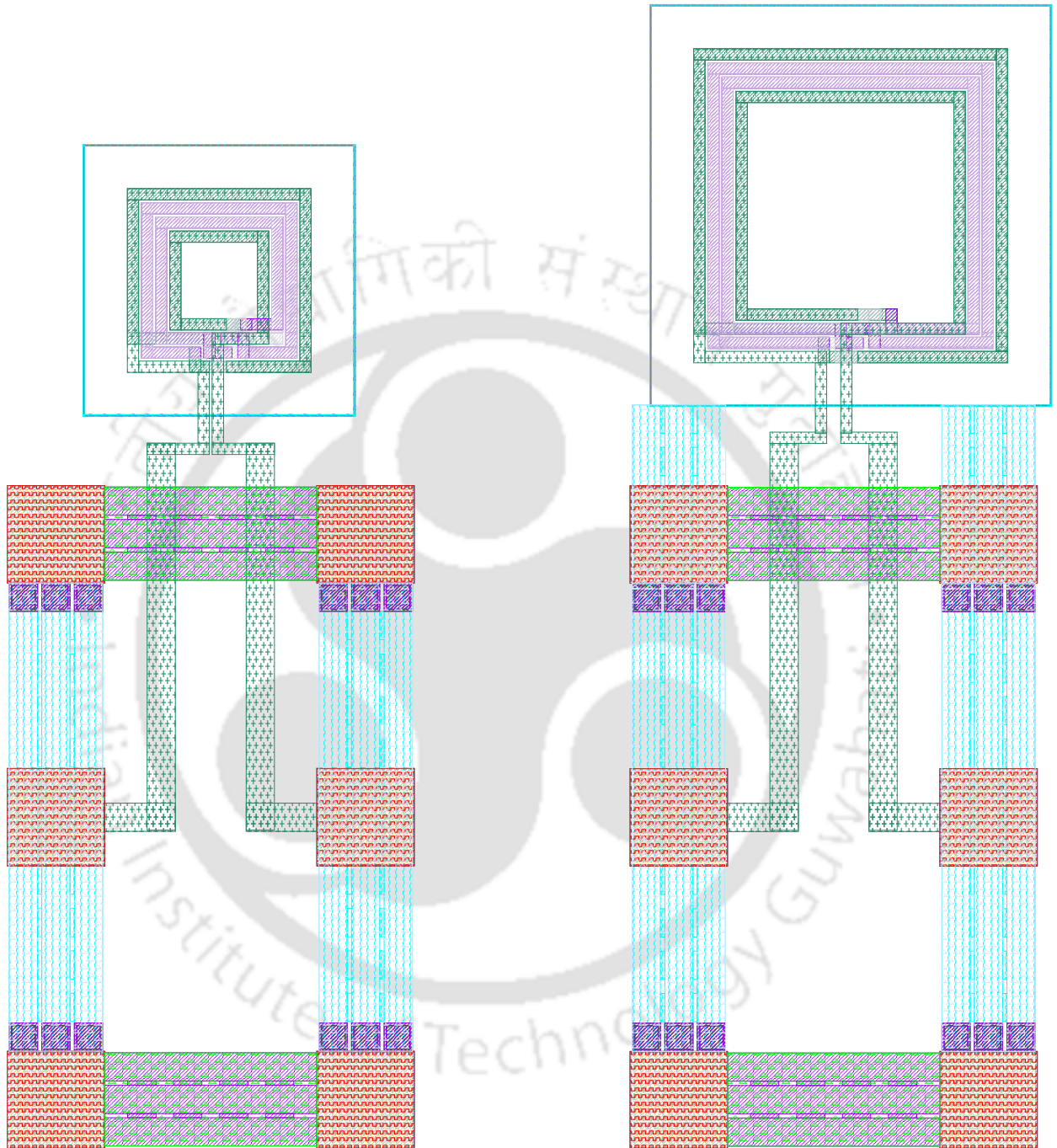
Figure 3.11: Layout of MPS test inductors W8_Dout130 (left) and W8_Dout222 (right) in GSG configuration for on wafer measurement.
