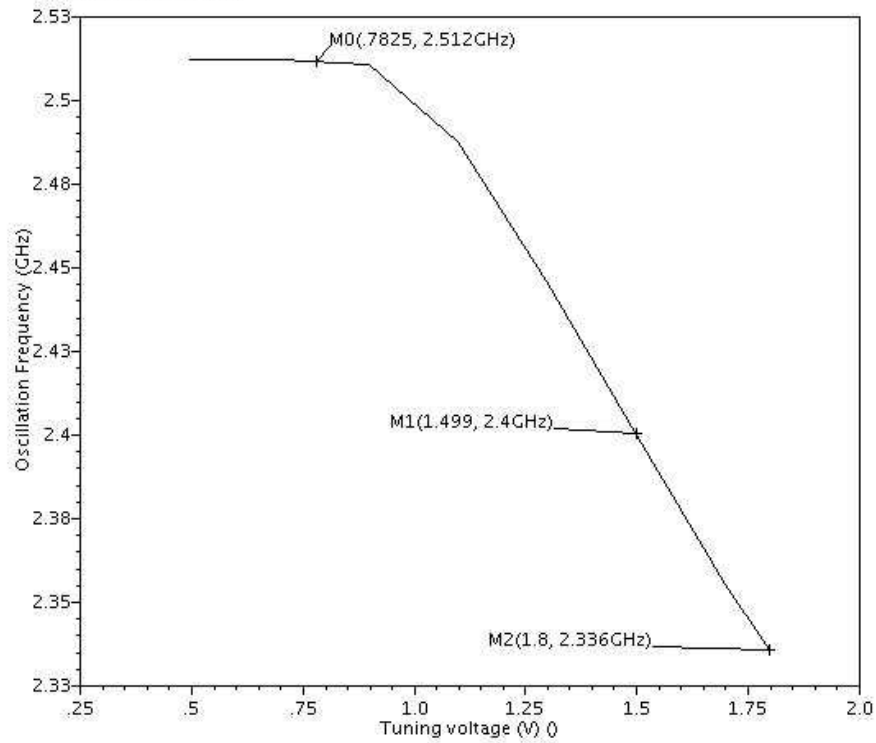
Figure 4.10: Simulated tuning characteristic of the VCO.
