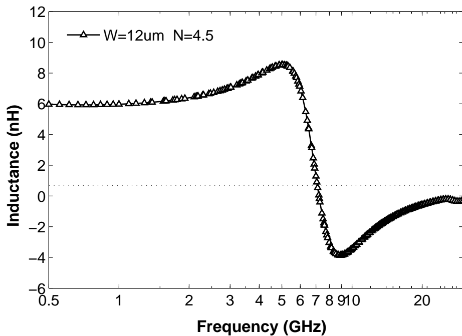
Figure 2.17: Inductance of the optimum design of 6 nH inductor as a function of frequency.
