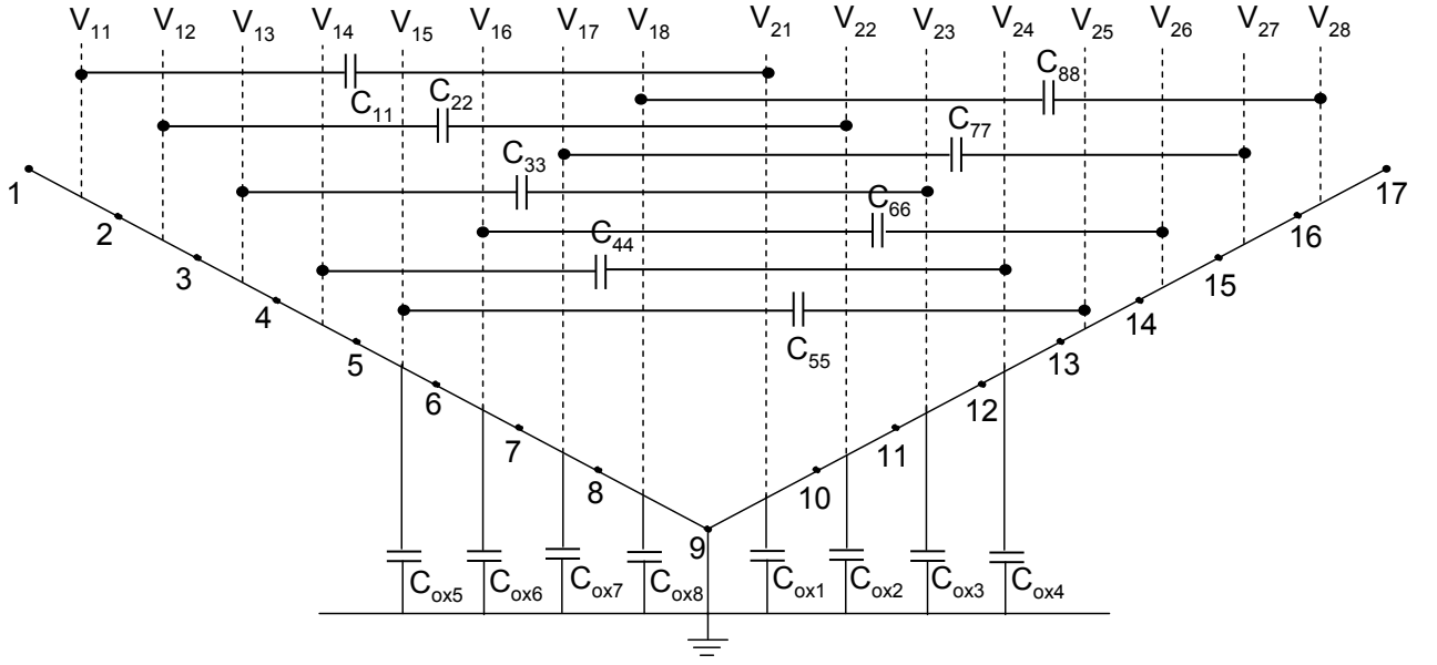
Figure A.1: Voltage profile and distributed capacitance of two layer conventional symmetric inductor.
