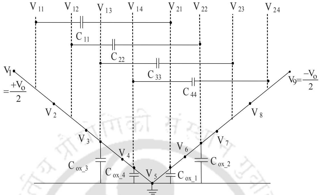
Figure 3.4: Voltage profile and distributed capacitance of multilayer pyramidal symmetric inductor.
