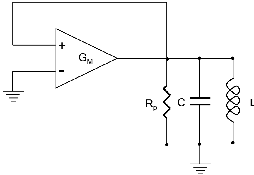
Figure 4.8: Transconductance model of the oscillator.
