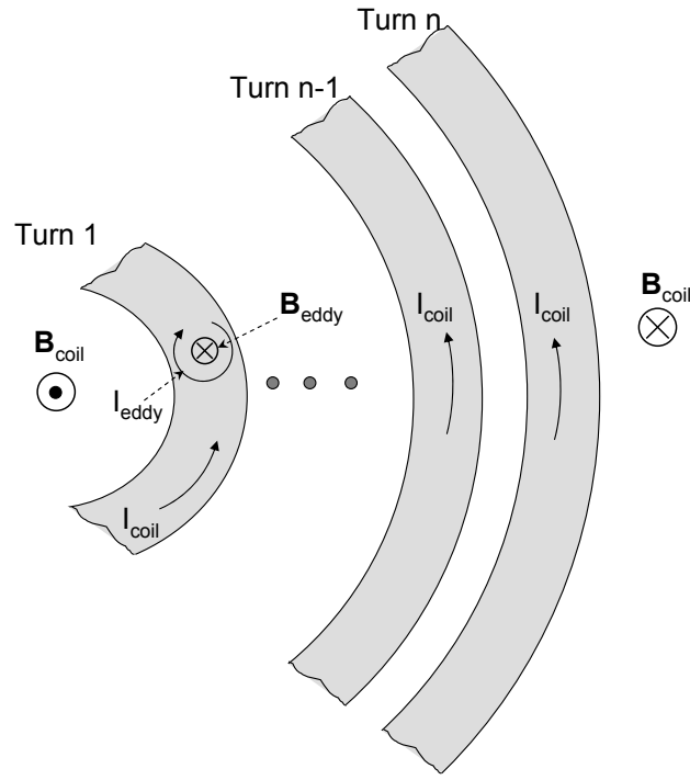
Figure 1.6: Section of an n -turn circular inductor with the fields and the eddy current.
