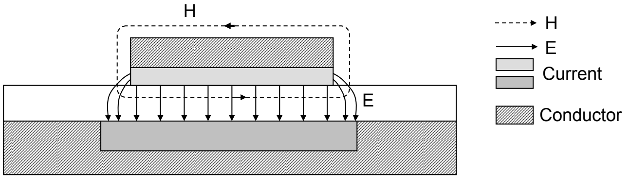
Figure 1.5: Eddy current effect in the microstrip stripline conductor.
