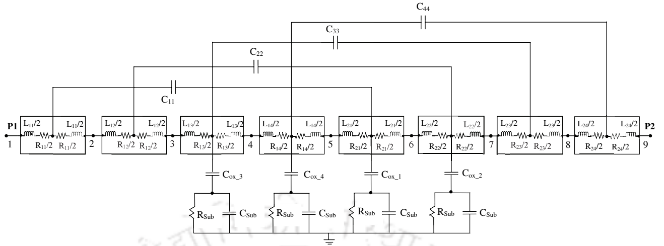
Figure 3.3: Lumped element model of a four layer multilayer pyramidal symmetric inductor.
