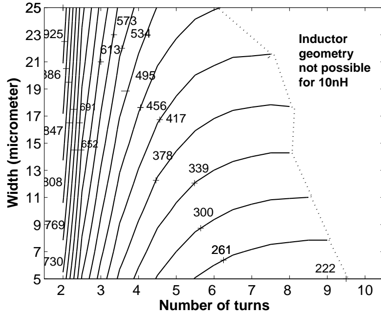
Figure 2.6: Contour plots of outer diameter (with labels in \mu\text{m} ) as a function of width and turns for a 10 nH inductor with spacing 6 \mu\text{m} .
