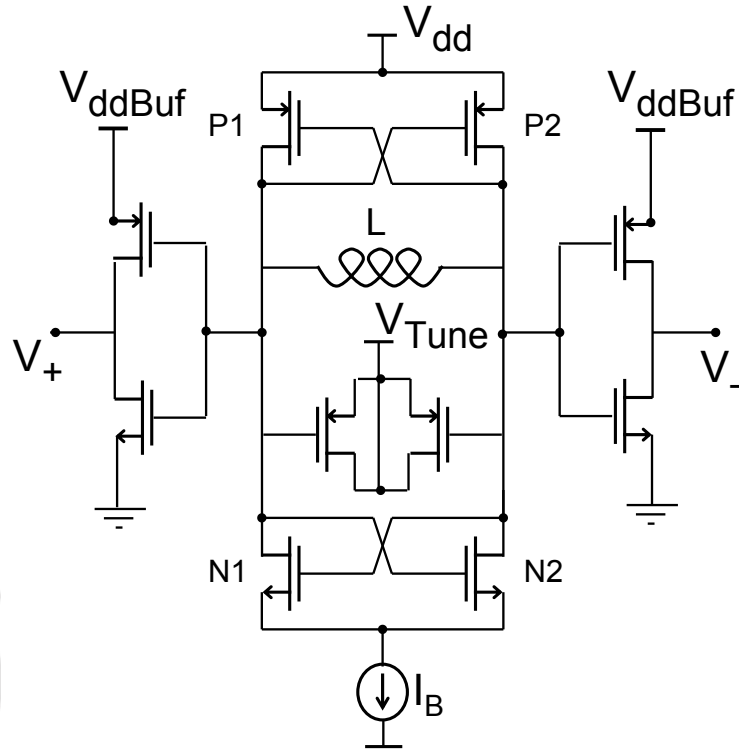
Figure 4.7: Schematic of the cross coupled LC voltage controlled oscillator.
