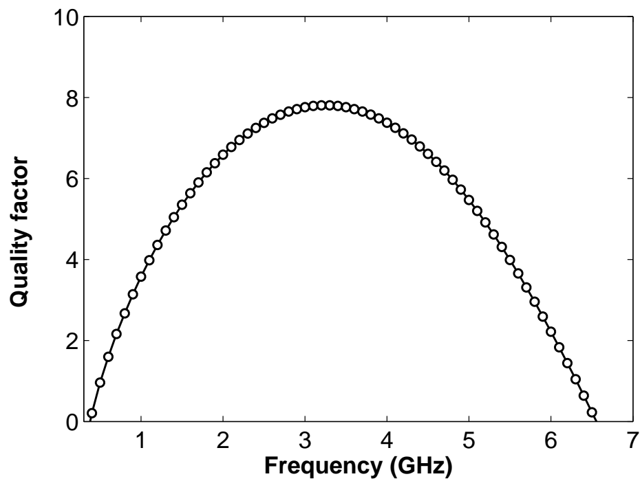
Figure 4.2: Quality factor plot of the tank MPS inductor.
