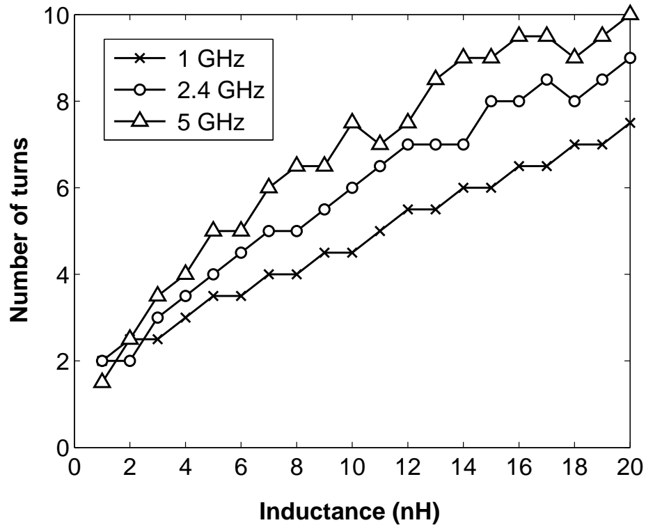
Figure 2.22: Optimum number of turns versus inductance at 1 GHz, 2.4 GHz and 5 GHz.
