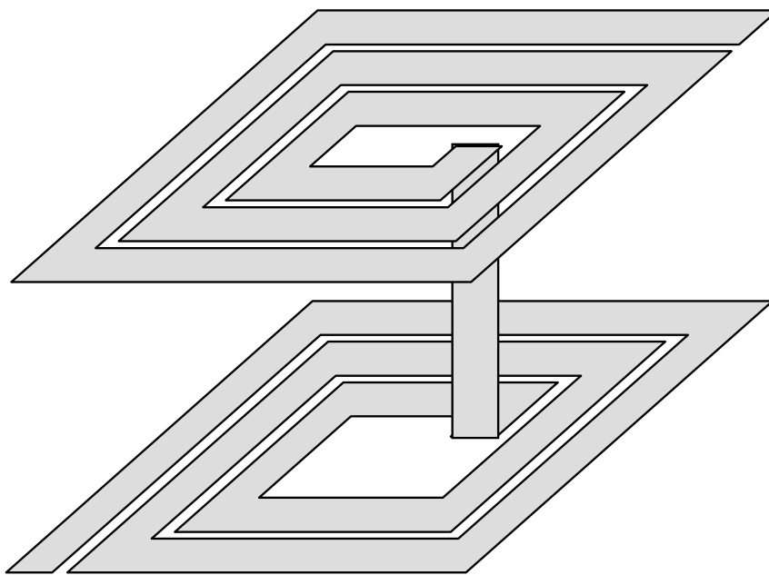
Figure 1.9: Conventional two layer stack spiral inductor.
