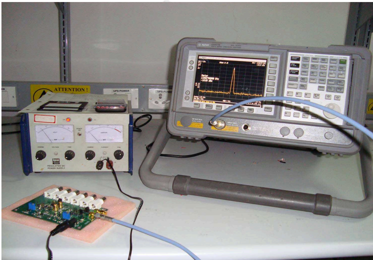
Figure 4.14: Testing and measurement of the VCO on the prototype board.
