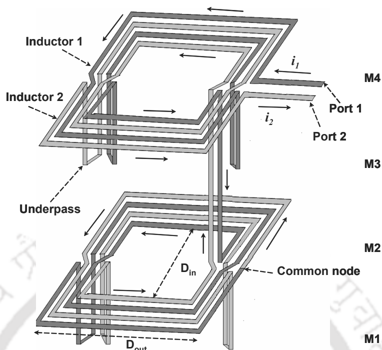
Figure 3.1: Layout of a two layer conventional symmetric inductor using four metal layers (not drawn to scale).
