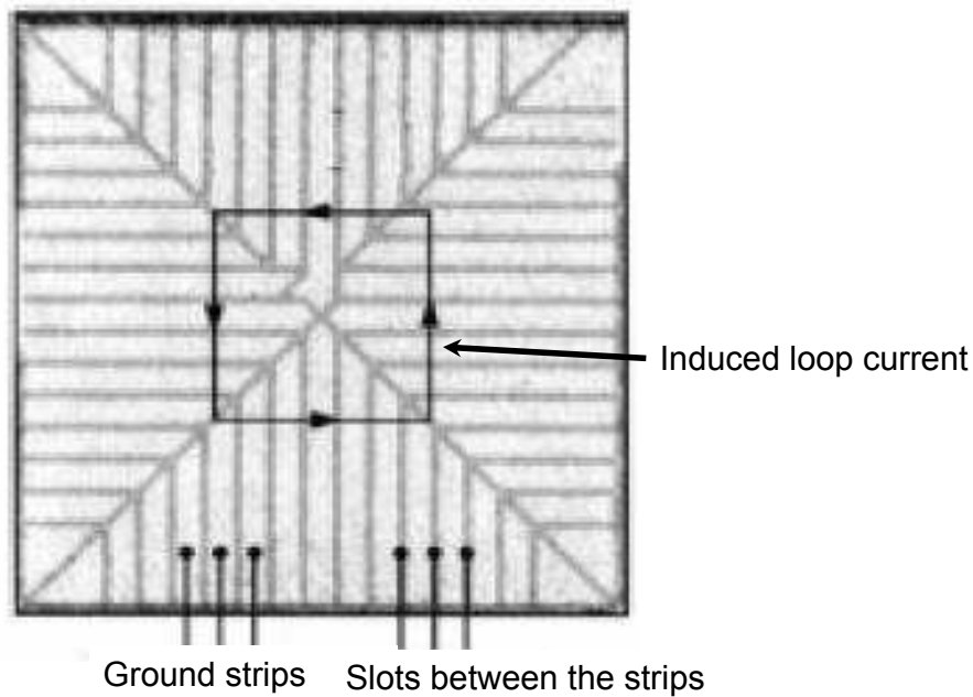
Figure 1.10: A patterned ground shield that can be inserted between an on-chip spiral inductor and silicon substrate to reduce the unwanted substrate effects [4].
