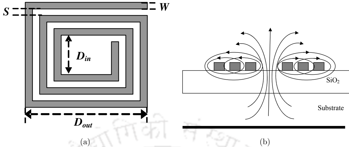
Figure 1.1: Planar spiral inductor and its cross section showing the magnetic field lines.
