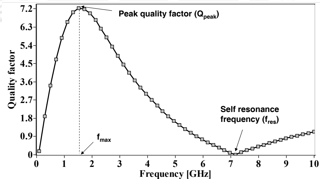
Figure 1.4: Quality factor as a function of frequency.
