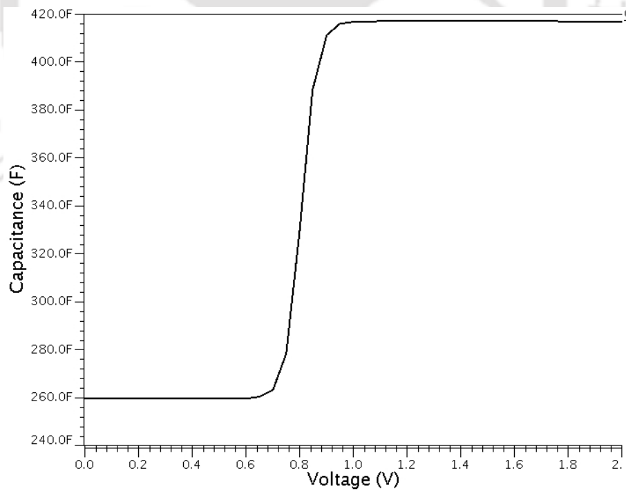
Figure 4.6: Variation of the capacitance for a single PMOS of the tank capacitor with the control voltage.
