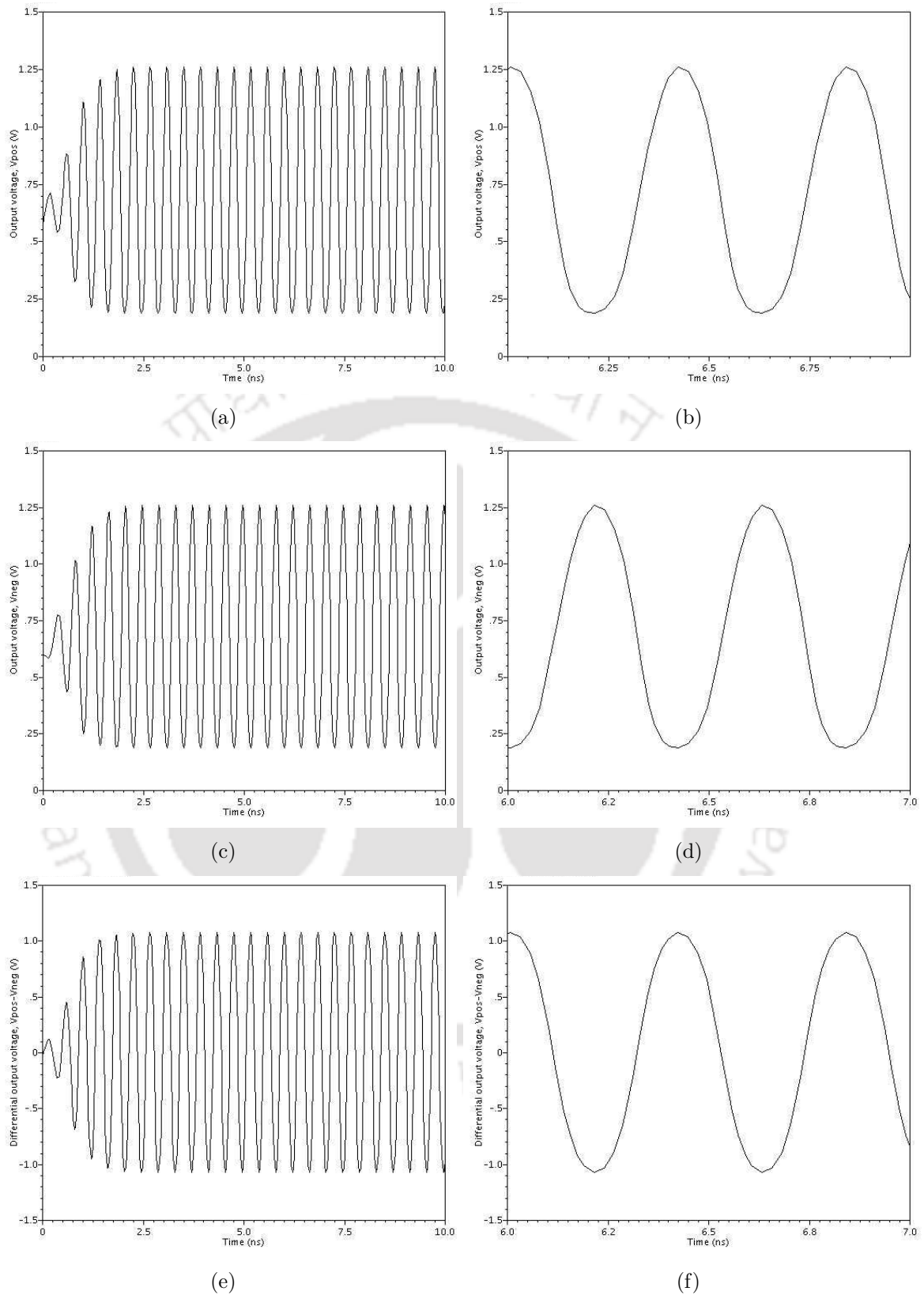
Figure 4.9: (a) Single ended outputs at positive node of the VCO. (b) Enlarged version of figure (a). (c) Single ended outputs at negative node of the VCO. (d) Enlarged version of figure (c). (e) Differential output of the VCO and (f) Enlarged version of (e).
