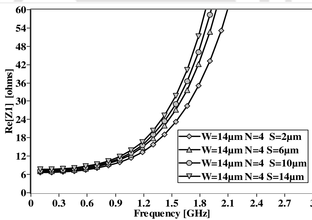
Figure 2.13: Parasitic series resistance for 10 nH inductors designed with different spacing of 2 μm, 6 μm, 10 μm and 14 μm.
