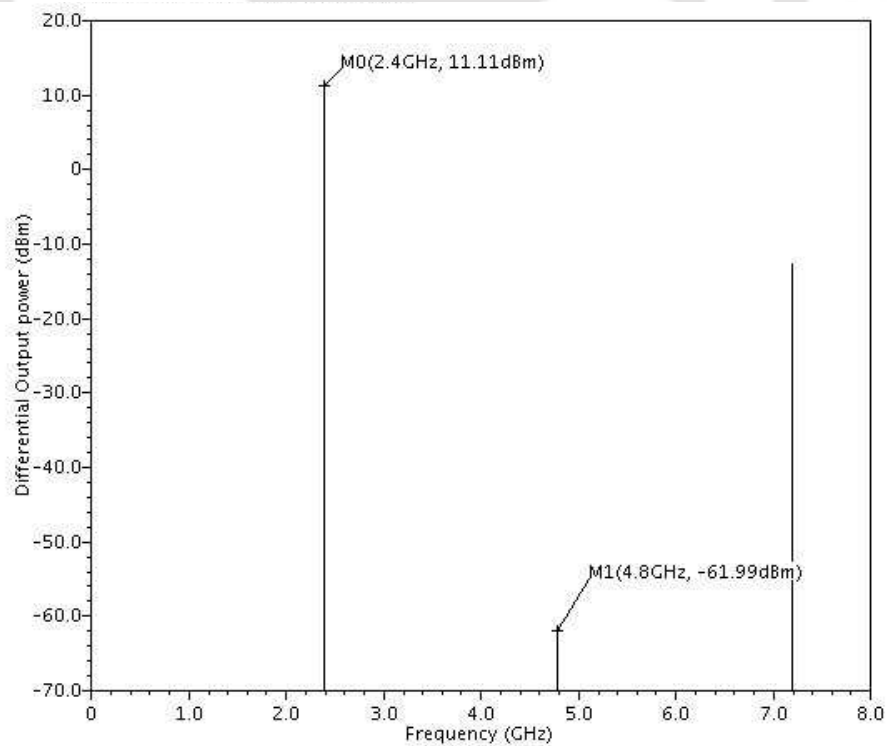
Figure 4.11: Simulated output power spectrum of the VCO.
