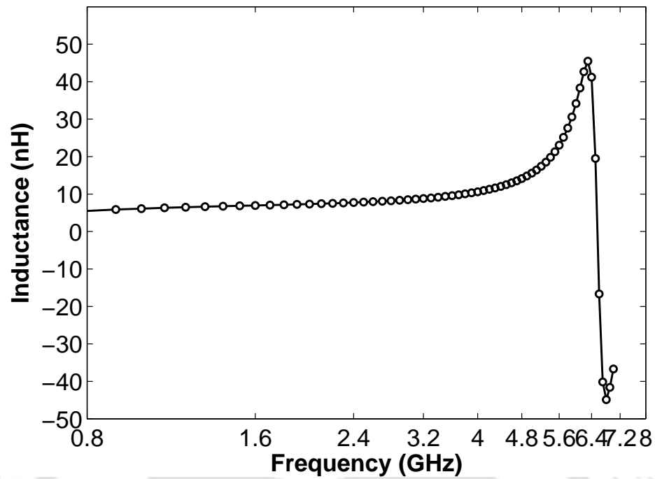
Figure 4.1: Inductance plot of the tank MPS inductor.
