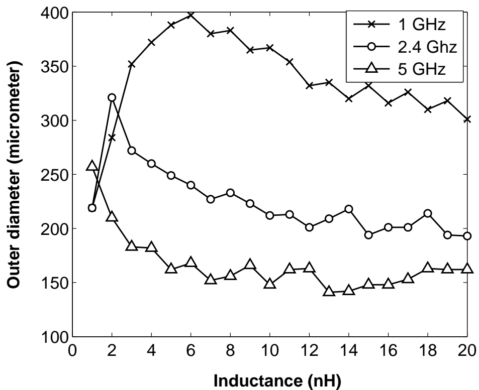
Figure 2.23: Optimum outer diameter versus inductance at 1 GHz, 2.4 GHz and 5 GHz.
