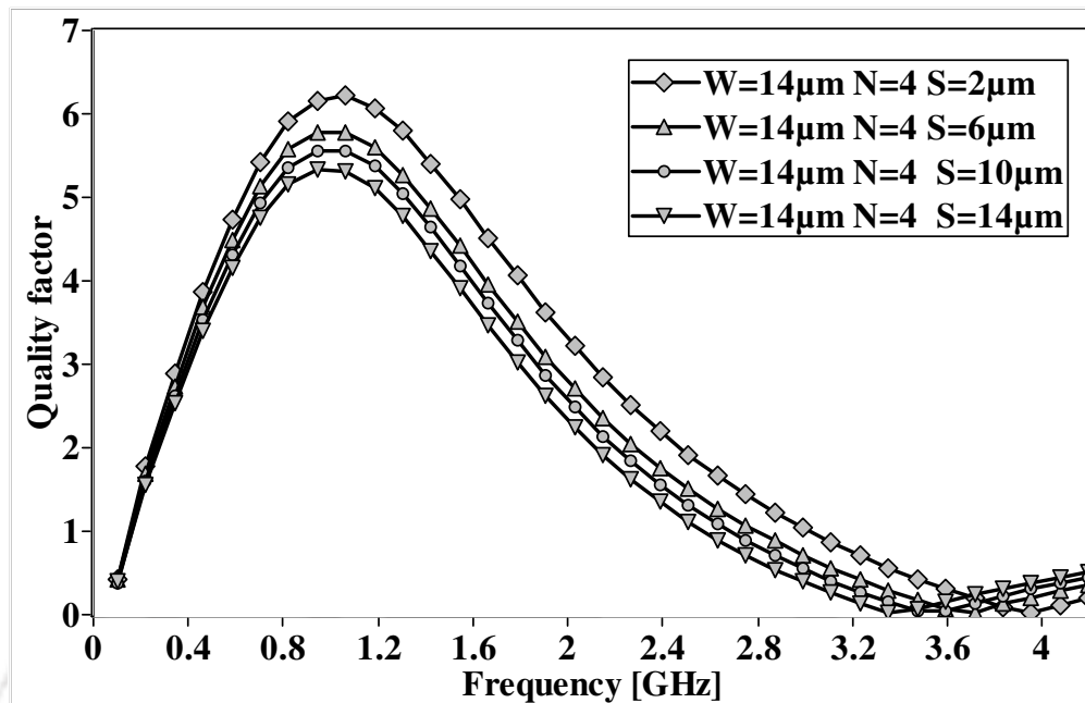
Figure 2.12: Quality factor for 10 nH inductors designed with different spacing of 2 μm, 6 μm, 10 μm and 14 μm with number of turns and width fixed at 4 and 14 μm respectively.
