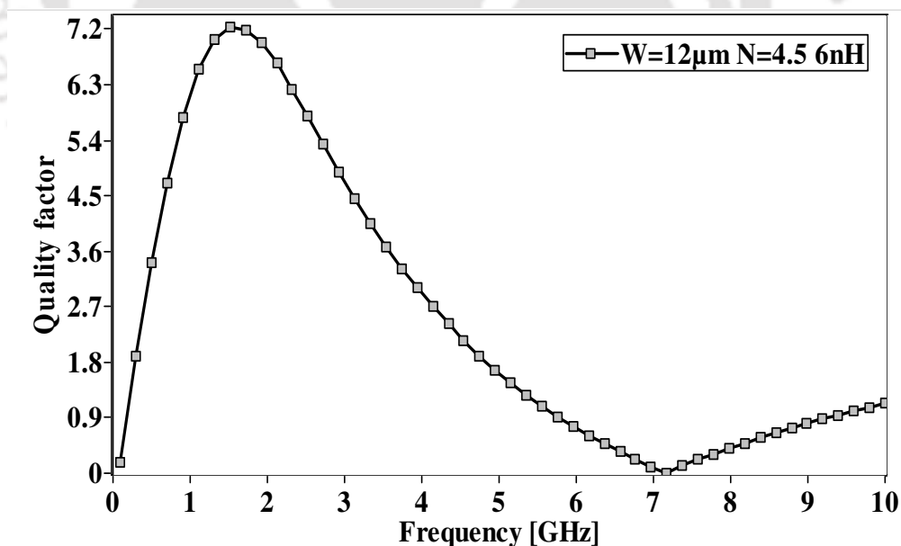
Figure 2.18: Quality factor of the optimum design of 6 nH inductor as a function of frequency.
