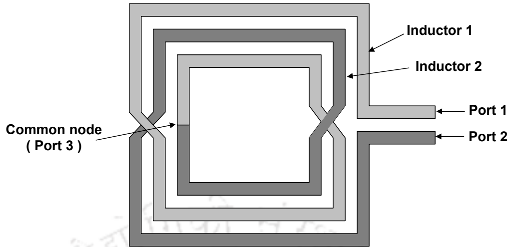
Figure 1.12: Layout of a pair of asymmetric planar inductor for differential circuit implementation.
