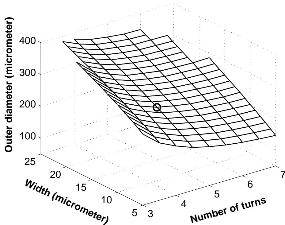
Figure 2.16: Outer diameters for 6 nH inductors as a function of width and number of turns.
