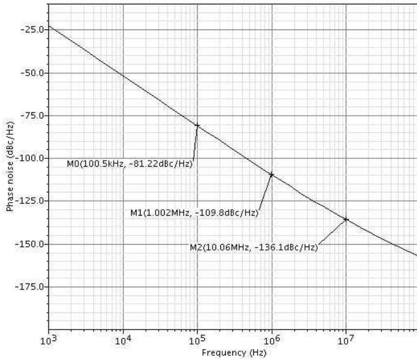
Figure 4.12: Simulated phase noise of the VCO.
