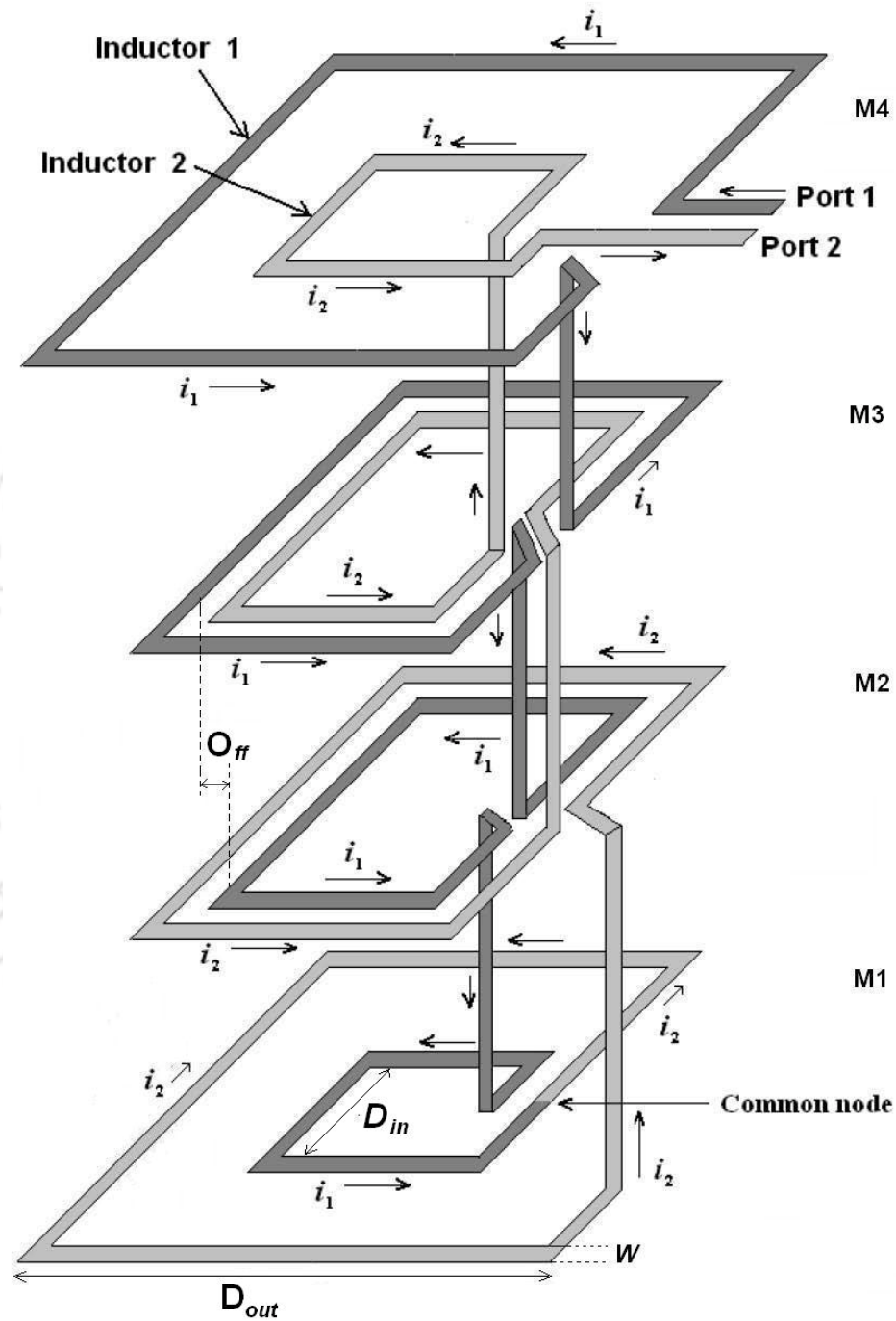
Figure 3.2: Multilayer pyramidal symmetric inductor.
