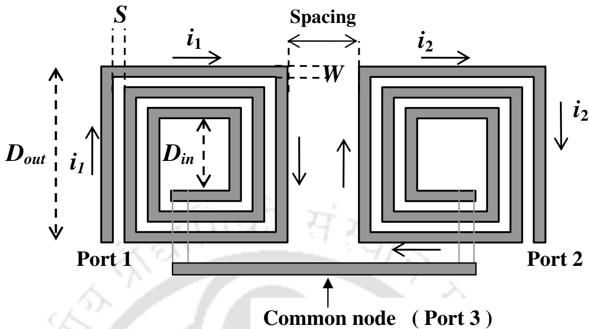
Figure 1.11: Layout of a pair of asymmetric planar inductor for differential circuit implementation.
