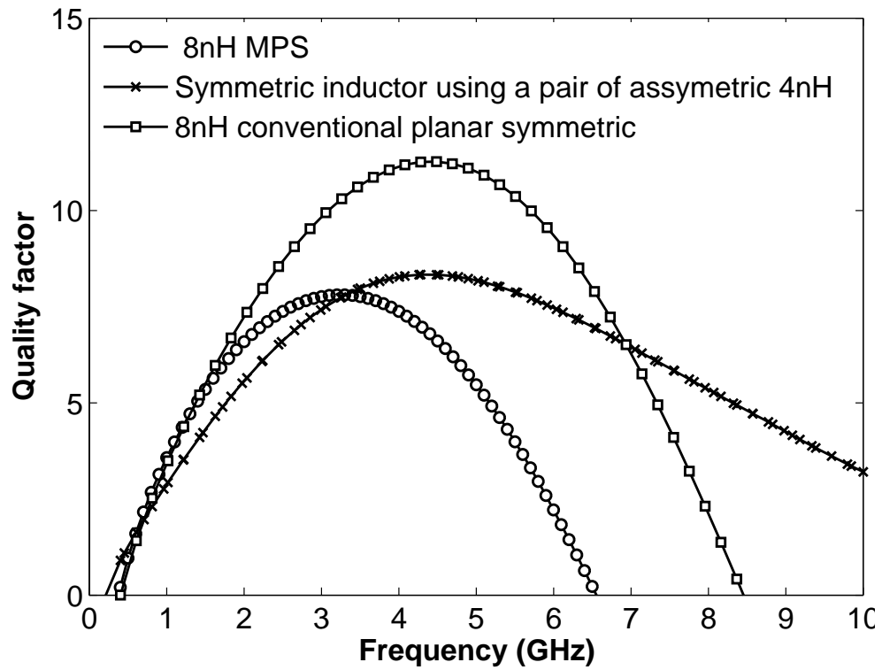
Figure 3.9: Quality factor comparison of 8 nH MPS inductors with conventional planar symmetric inductors.
