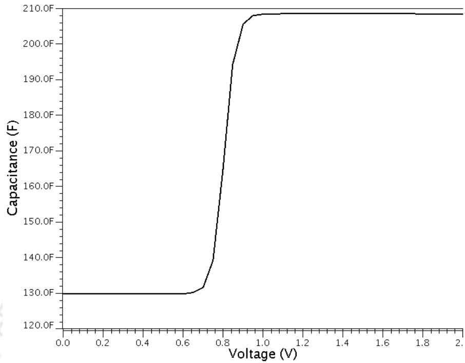
Figure 4.5: Variation of the total tank capacitance with the control voltage.
