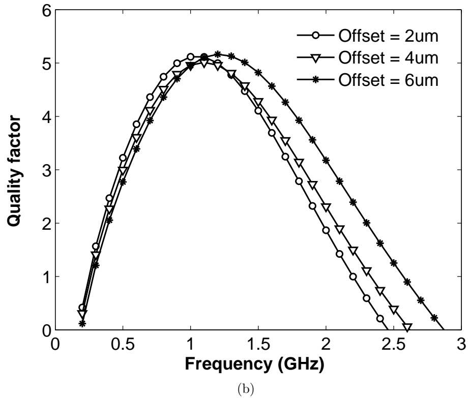
Figure 3.7: (a) Inductance and (b) Quality factor of MPS inductors (Group C) with different offsets between the adjacent metal layers. Width and outer diameter is kept constant at 12 \mu\text{m} and 222 \mu\text{m} respectively.
