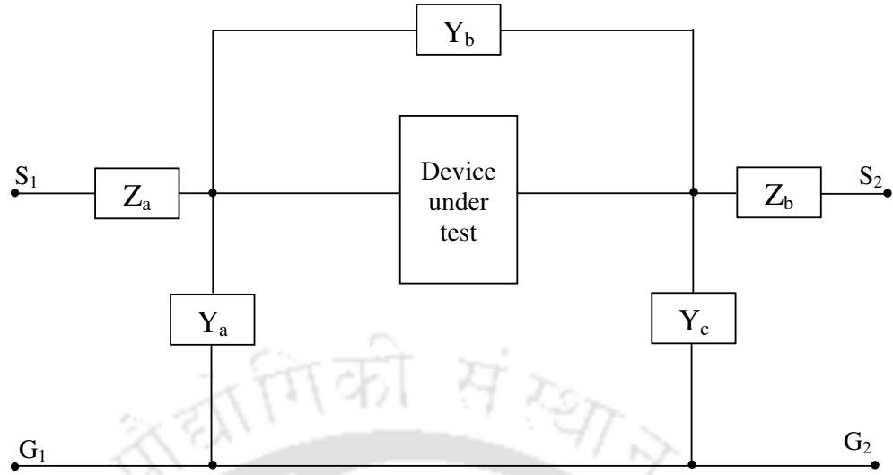
Figure 3.14: A simplified model of the DUT with the series and parallel parasitics.
