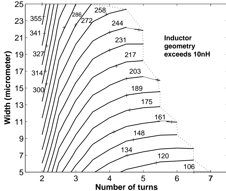
Figure 2.7: Contour plots of outer diameter (with labels in \mu\text{m} ) as a function of width and turns for a 10 nH inductor assumed to be designed by stacking two spirals of 2.5 nH inductance
