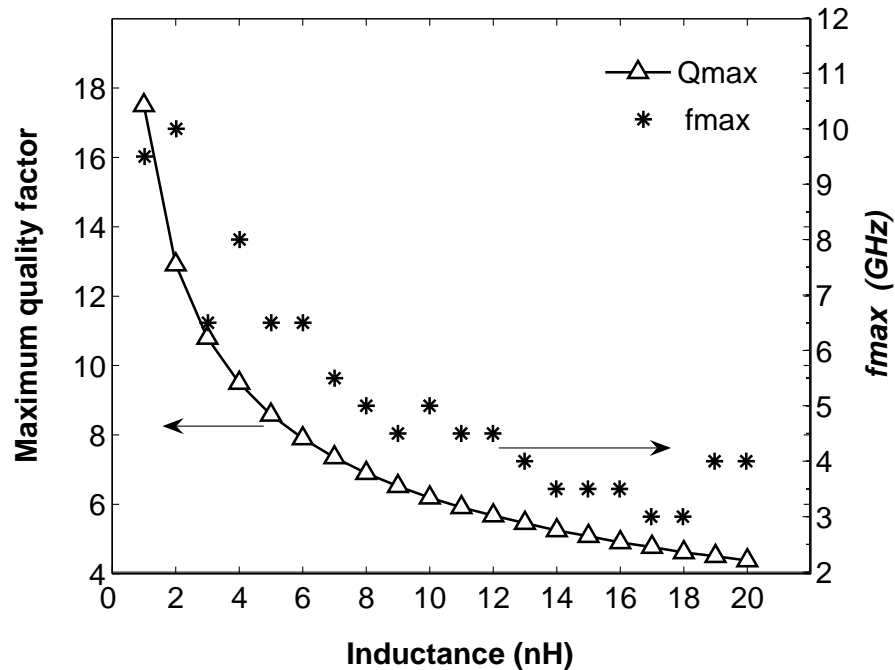
Figure 2.24: Maximum quality factor and their corresponding peak frequency for inductance range 1 nH - 20 nH.
