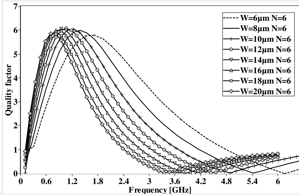
Figure 2.10: Quality factor for 10 nH inductors designed with different width of 6 \mu\text{m} , 8 \mu\text{m} , 10 \mu\text{m} , 12 \mu\text{m} , 14 \mu\text{m} , 16 \mu\text{m} , 18 \mu\text{m} and 20 \mu\text{m} .
