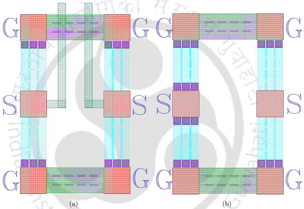
Figure 3.12: Standard test fixtures used to characterize the parasitics (a) Open and (b) Short.
