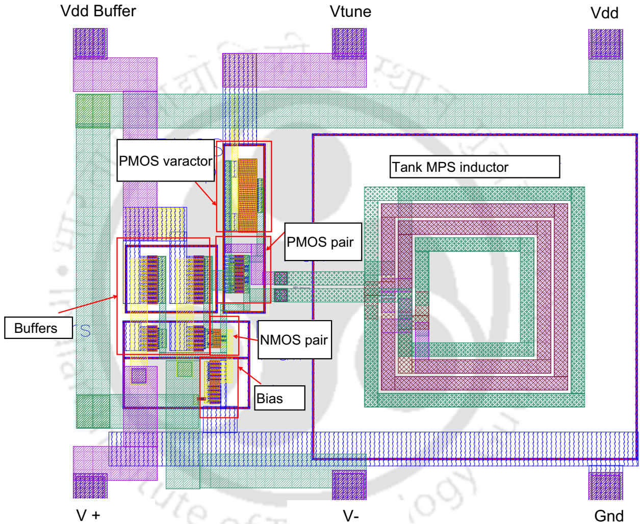
Figure 4.13: Layout of the VCO.
