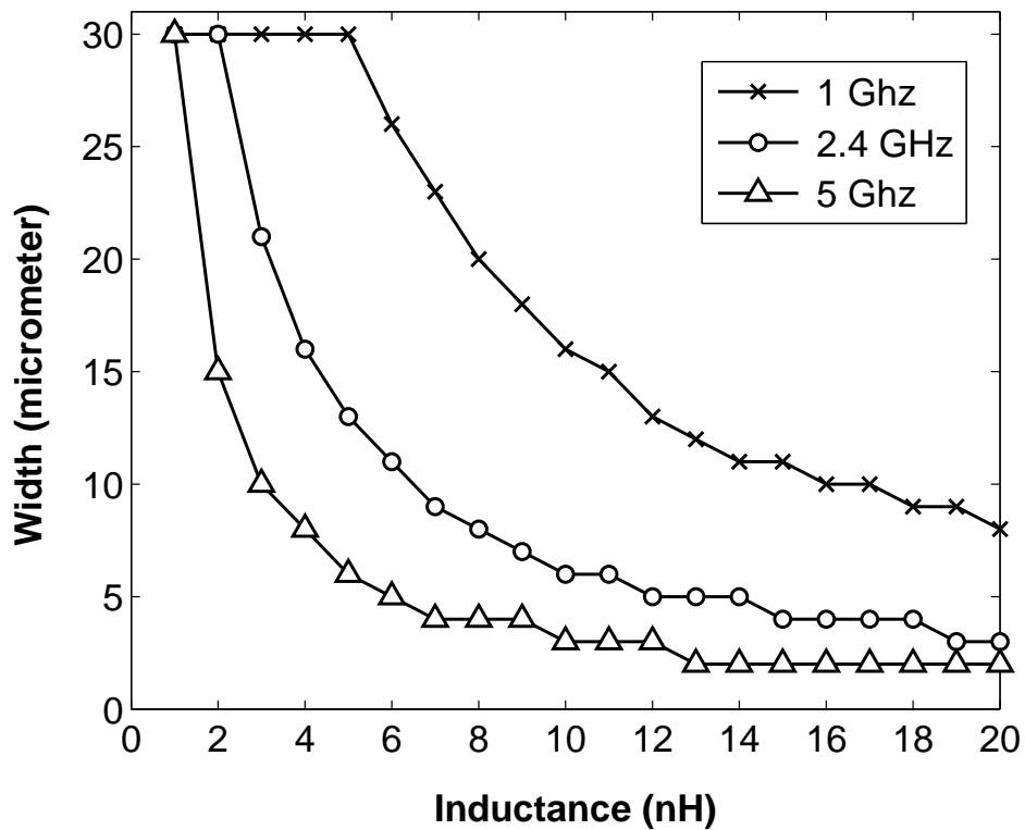
Figure 2.21: Optimum width versus inductance at 1 GHz, 2.4 GHz and 5 GHz.
