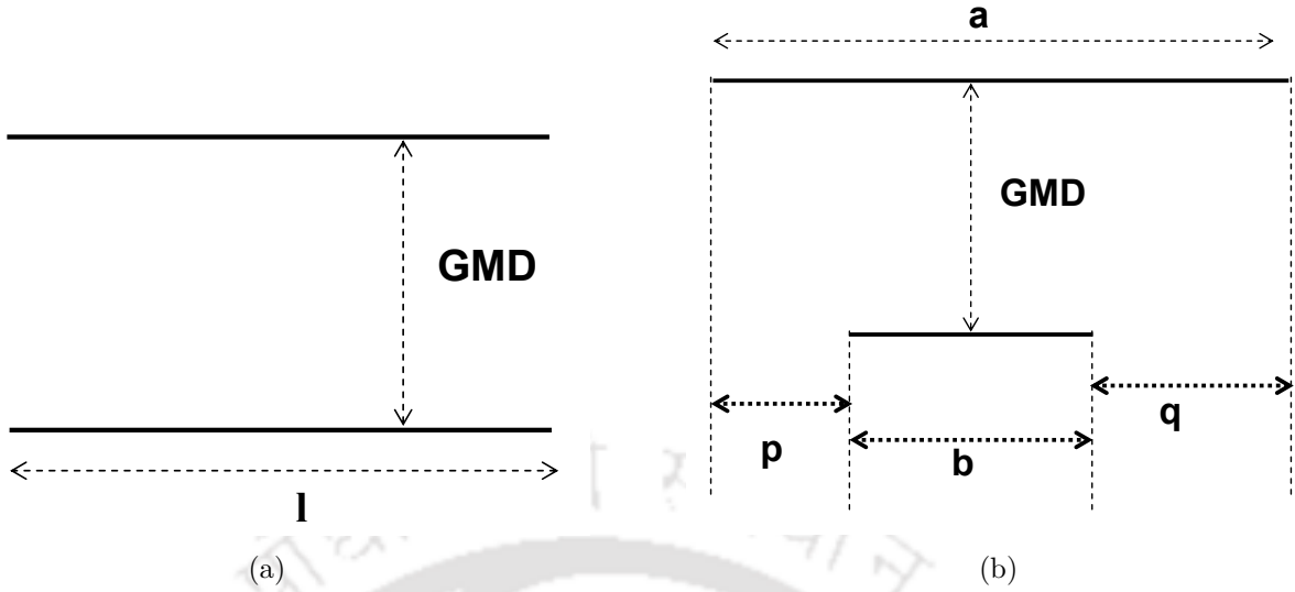
Figure 2.2: Parallel conductors of (a) equal length (b) different length.
