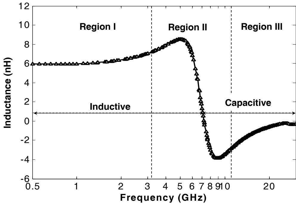
Figure 1.3: Inductance as a function of frequency.
