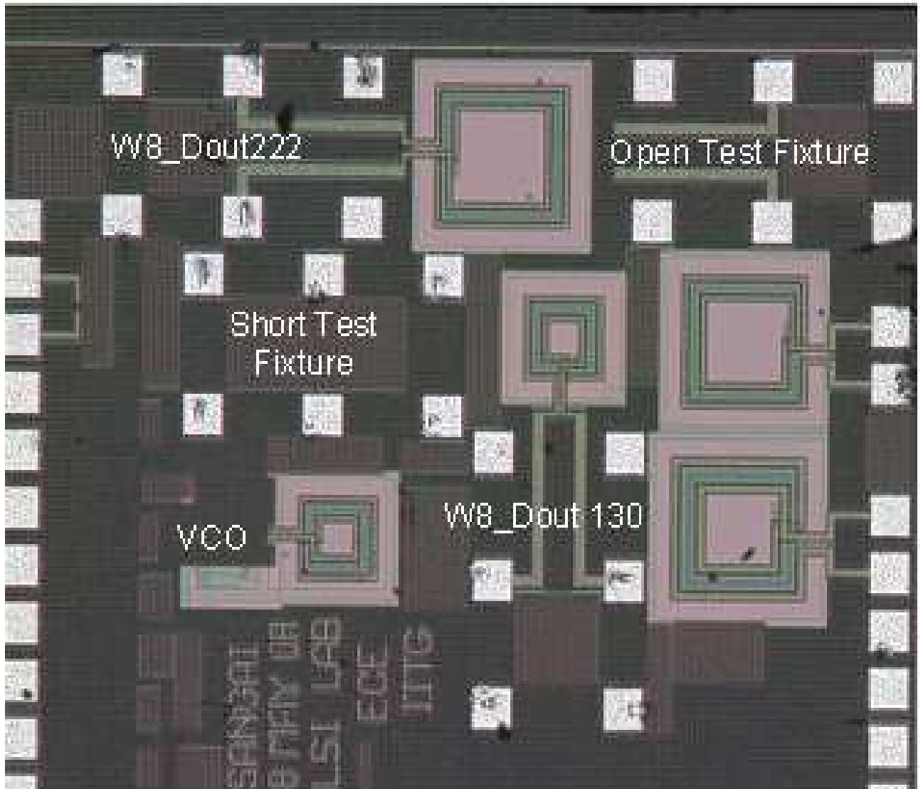
Figure 3.15: Micrograph of the chip with inductors and the VCO.
