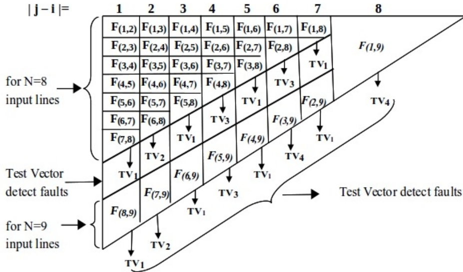
Figure 2.2: Demonstration of single input bridging faults for N=8 and N=9
