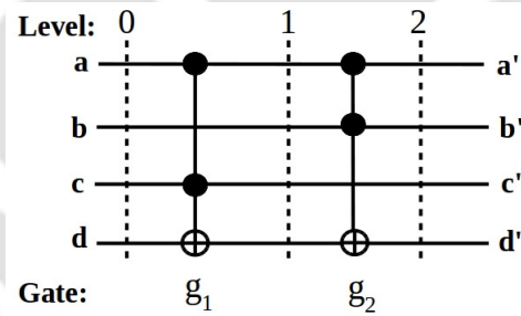
Figure 4.2: Toffoli_double_4 benchmark circuit
