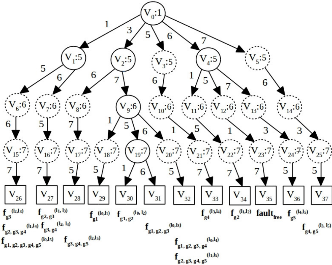
Figure 5.6: Unit vertices of a fault localization tree for the circuit Miller_11 during the reduction process
