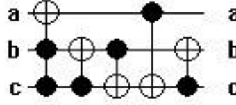
Figure 4.3: ham3tc benchmark circuit
