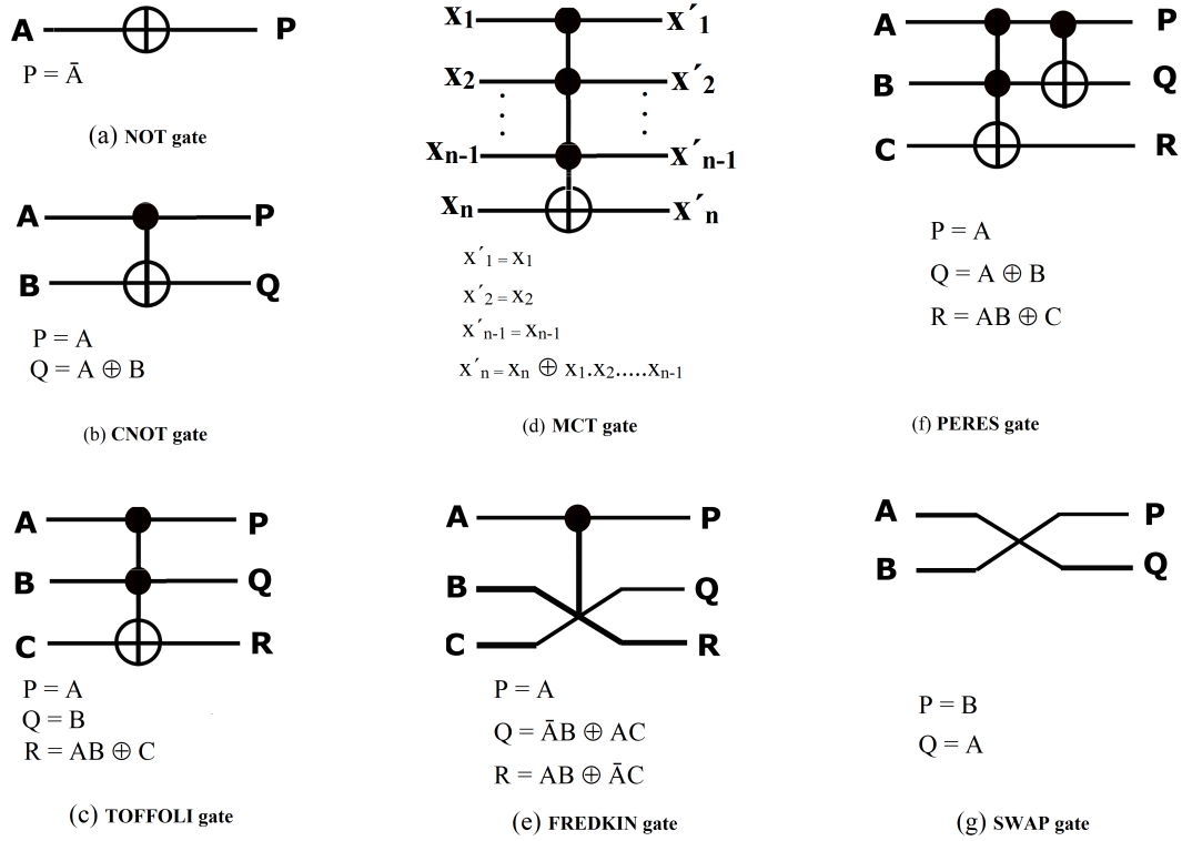
Figure 1.1: Reversible Gates and their Gate Operation.
