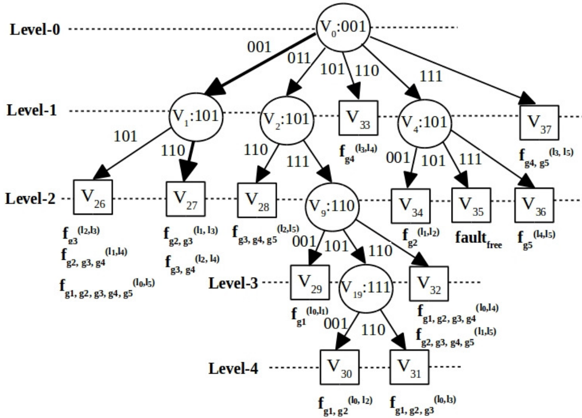
Figure 5.10: Traversal process of fault f_{g2}^{(l1, l2)} for the circuit Miller_11
