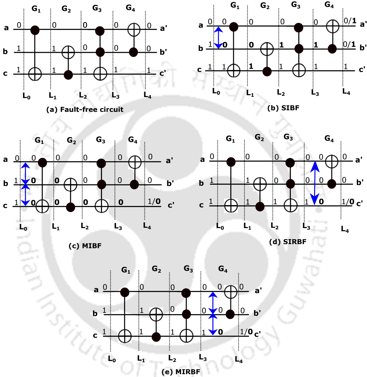
Figure 3.1: Demonstration of Reversible Circuit n^{th\_Prime3\_inc} for various bridging fault conditions
